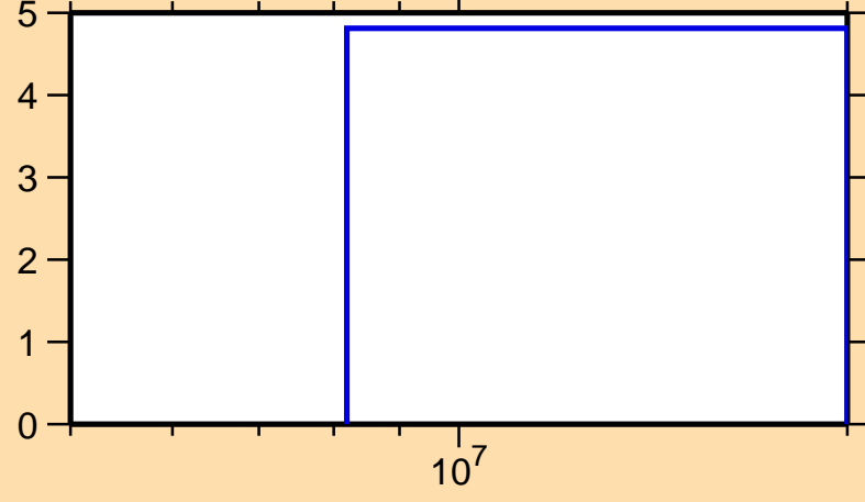
\Delta\sigma/\sigma vs. E for ^{204}\text{Fr}(n,\text{el.})
