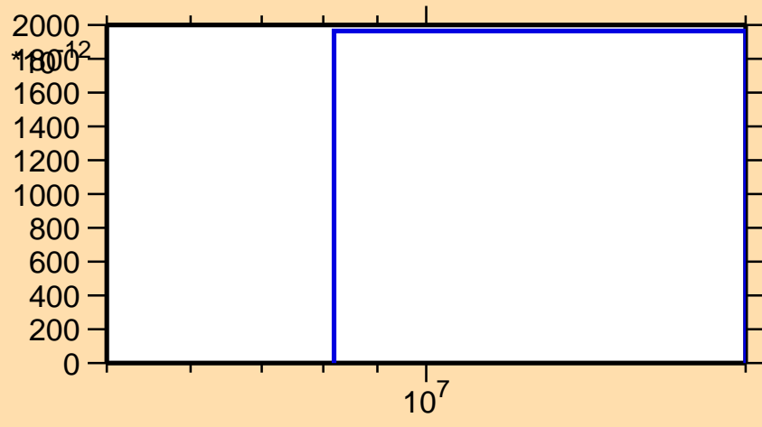
\sigma vs. E for ^{204}\text{Fr}(n,\text{pd})
