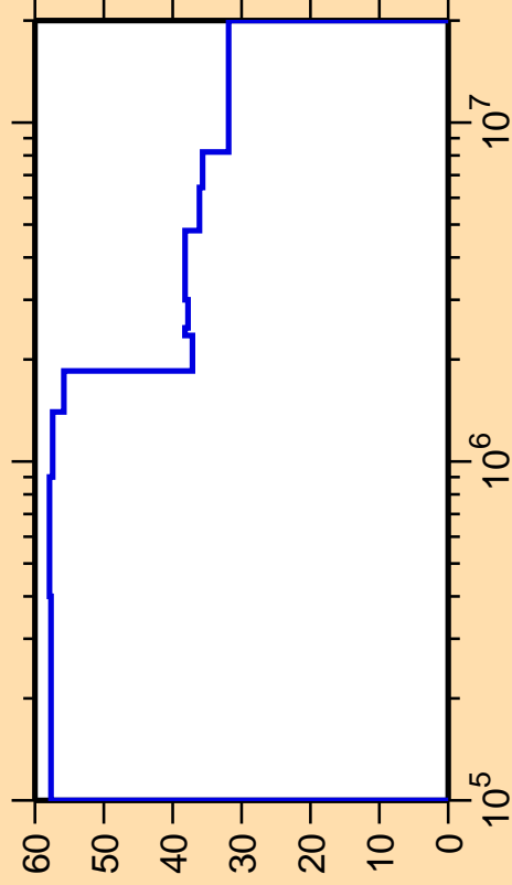
\Delta\sigma/\sigma vs. E for ^{204}\text{Fr}(n,n_2)
