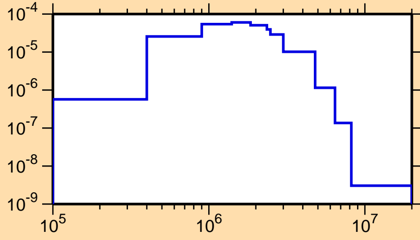
\sigma vs. E for ^{204}\text{Fr}(n,n_2)
