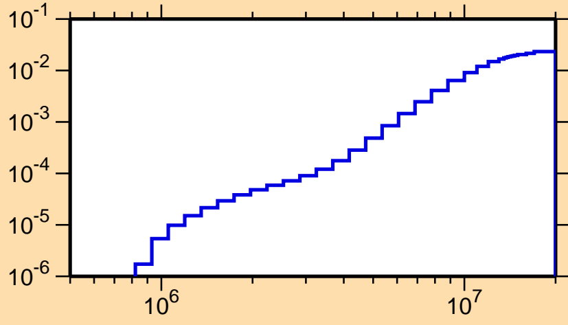
\sigma vs. E for ^{206}\text{Fr}(n,n\alpha)
