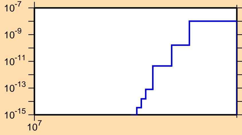
\sigma vs. E for ^{206}\text{Fr}(n,nt)
