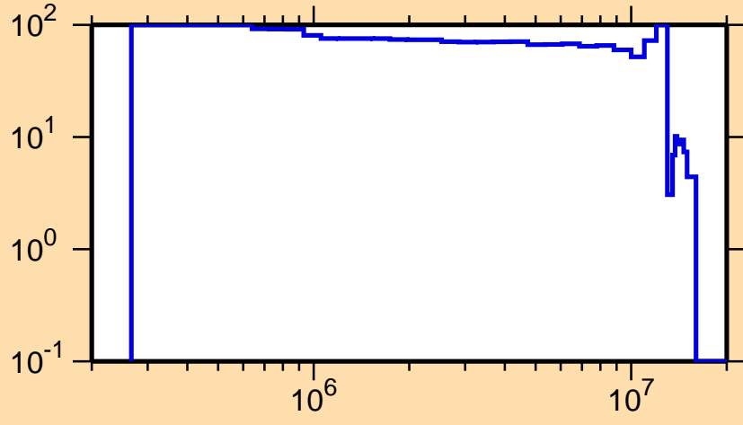
\Delta\sigma/\sigma vs. E for ^{206}\text{Fr}(n,n_1)
