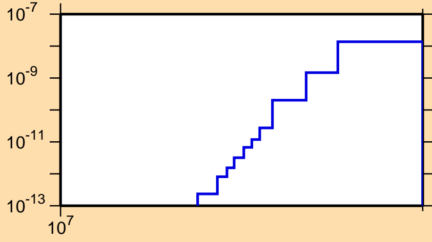
\sigma vs. E for ^{206}\text{Fr}(n,\text{pt})
