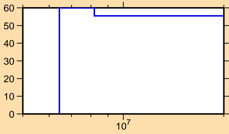
\Delta\sigma/\sigma vs. E for ^{206}\text{Fr}(n,2n)
