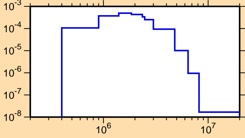
\sigma vs. E for ^{206}\text{Fr}(n,n_4)
