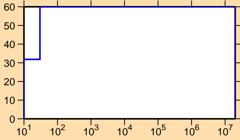
\Delta\sigma/\sigma vs. E for ^{206}\text{Fr}(n,p)
