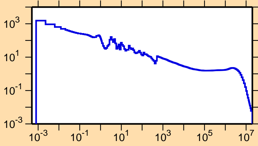
\sigma vs. E for ^{206}\text{Fr}(n,\gamma)
