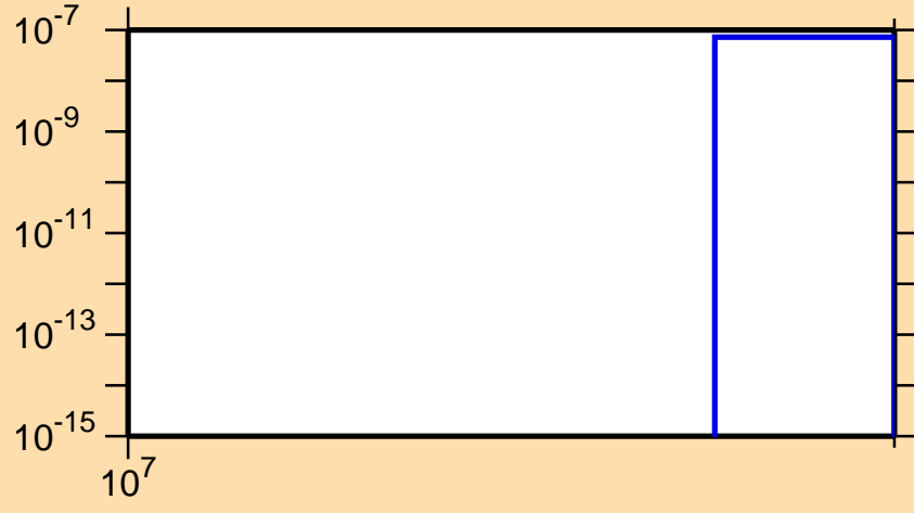
\sigma vs. E for ^{206}\text{Fr}(n,3n\alpha)
