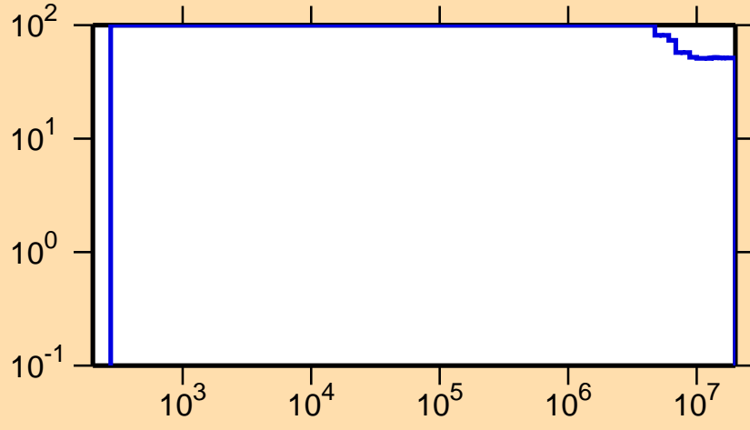
\Delta\sigma/\sigma vs. E for ^{206}\text{Fr}(n,p)
