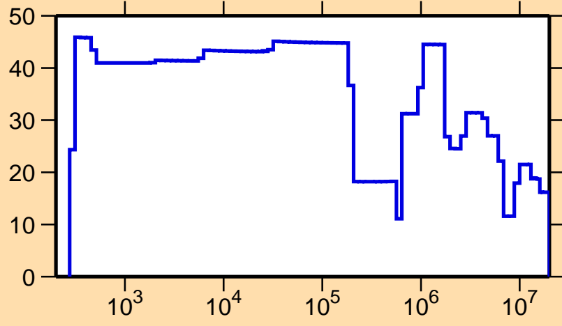
\Delta\sigma/\sigma vs. E for ^{206}\text{Fr}(n,\text{el.})
