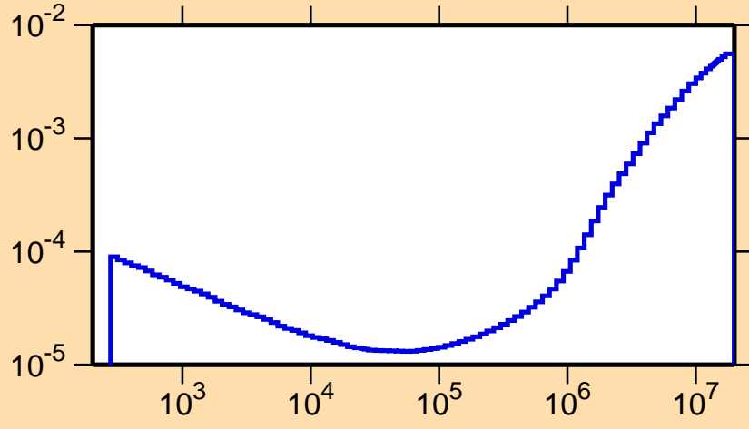
\sigma vs. E for ^{206}\text{Fr}(n,p\alpha)
