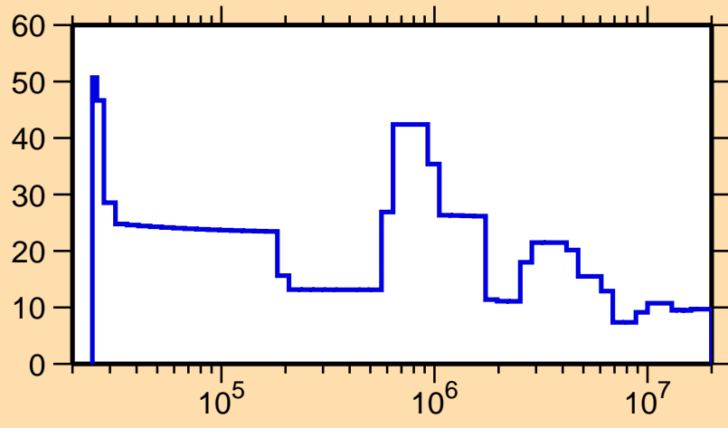
\Delta\sigma/\sigma vs. E for ^{206}\text{Fr}(n,\text{tot.})
