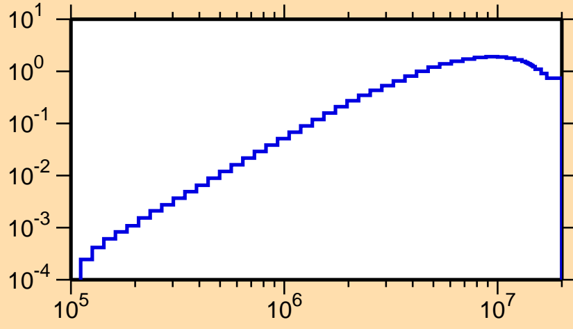
\sigma vs. E for ^{206}\text{Fr}(n,\text{inel.})
