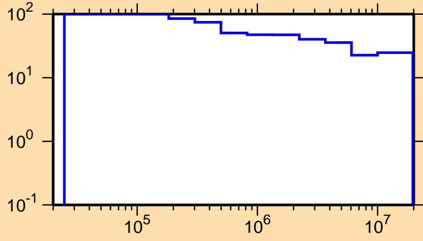
\Delta\sigma/\sigma vs. E for ^{206}\text{Fr}(n, ncont.)
