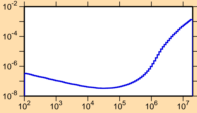
\sigma vs. E for ^{207}\text{Fr}(n,p\alpha)
