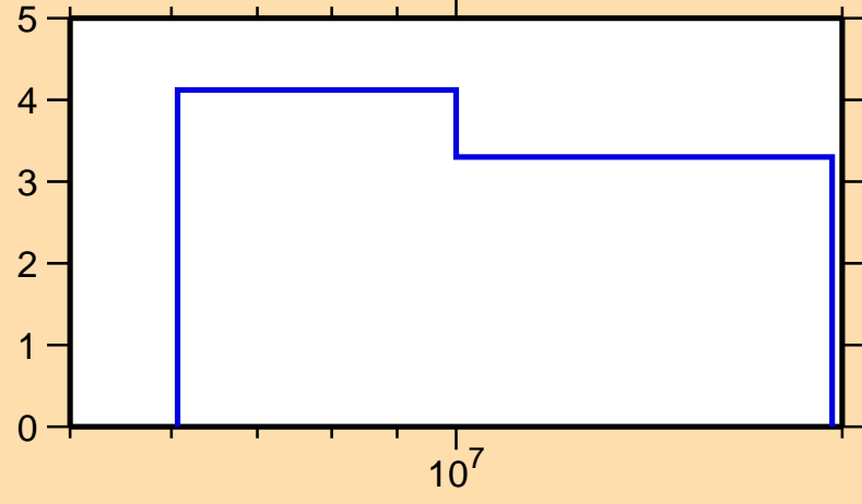
\Delta\sigma/\sigma vs. E for ^{207}\text{Fr}(n,\text{nonel.})
