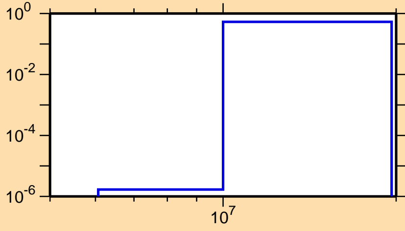
\sigma vs. E for ^{207}\text{Fr}(n,2n)
