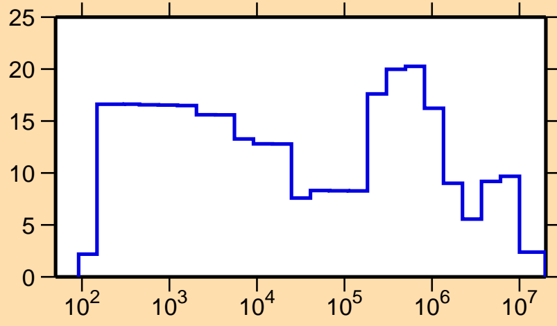
\Delta\sigma/\sigma vs. E for ^{207}\text{Fr}(n,\text{el.})
