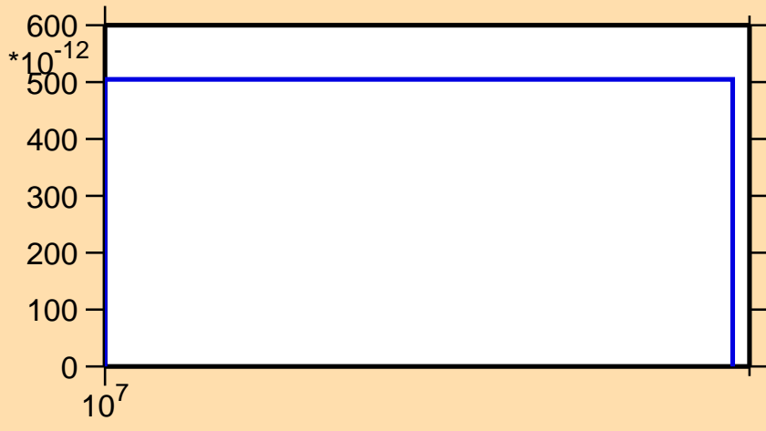
\sigma vs. E for ^{207}\text{Fr}(n,nt)
