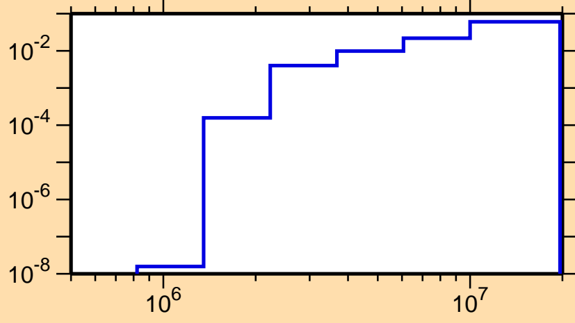
\sigma vs. E for ^{207}\text{Fr}(n,n\alpha)
