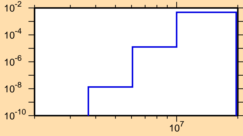
\sigma vs. E for ^{207}\text{Fr}(n,d)
