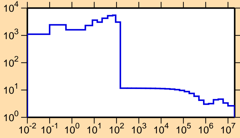
\sigma vs. E for ^{207}\text{Fr}(n,\text{el.})
