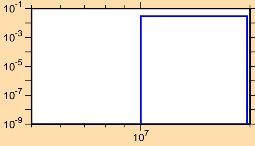
\sigma vs. E for ^{207}\text{Fr}(n,2n\alpha)
