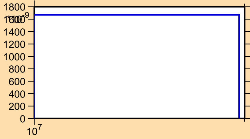
\sigma vs. E for ^{207}\text{Fr}(n,3n)
