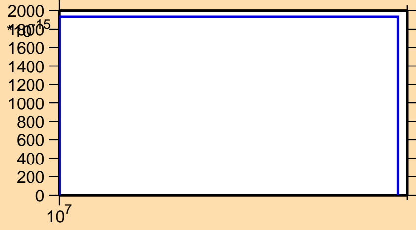
\sigma vs. E for ^{207}\text{Fr}(n,\text{pt})
