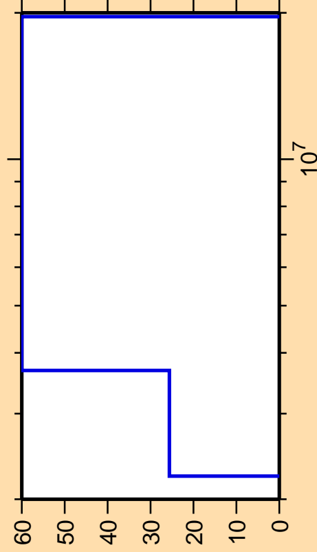
\Delta\sigma/\sigma vs. E for ^{207}\text{Fr}(n,d)
