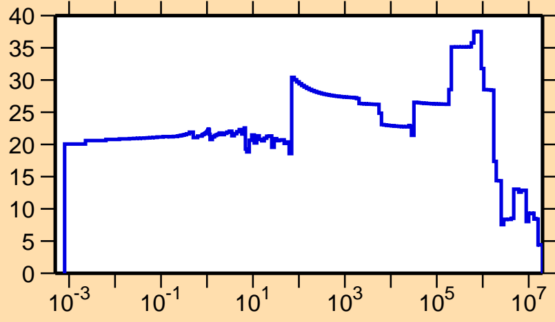
\Delta\sigma/\sigma vs. E for ^{208}\text{Fr}(n,\text{el.})
