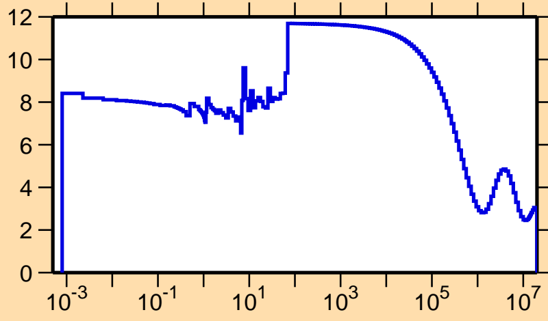
\sigma vs. E for ^{208}\text{Fr}(n,\text{el.})
