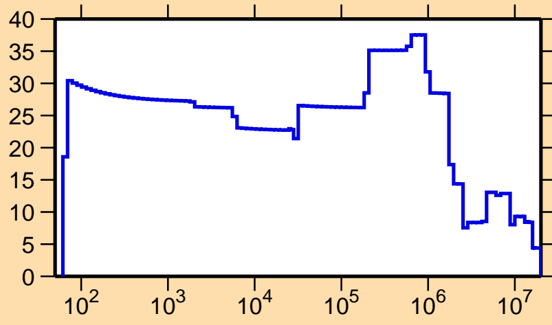
\Delta\sigma/\sigma vs. E for ^{208}\text{Fr}(n,\text{el.})
