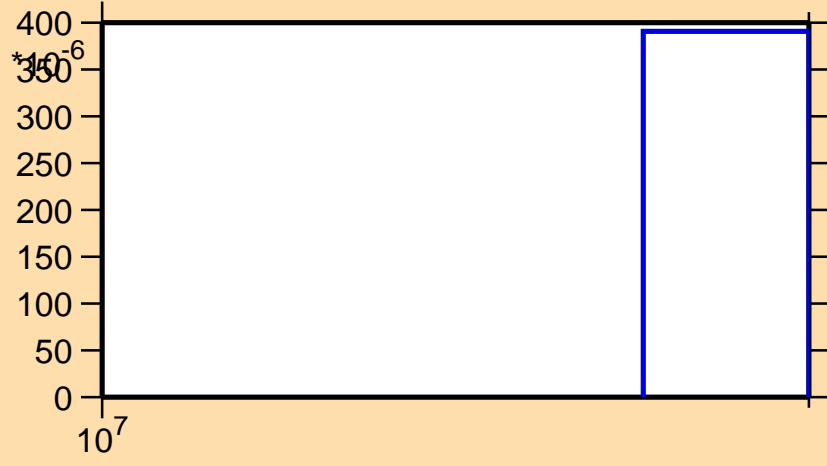
\sigma vs. E for ^{208}\text{Fr}(n,3n)
