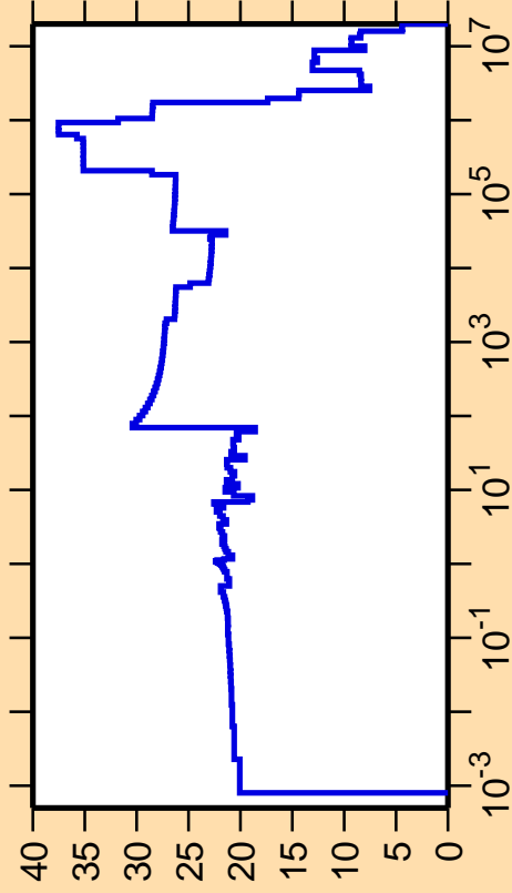
\Delta\sigma/\sigma vs. E for ^{208}\text{Fr}(n,\text{el.})
