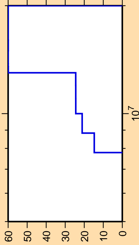
\Delta\sigma/\sigma vs. E for ^{208}\text{Fr}(n,n\text{cont.})
