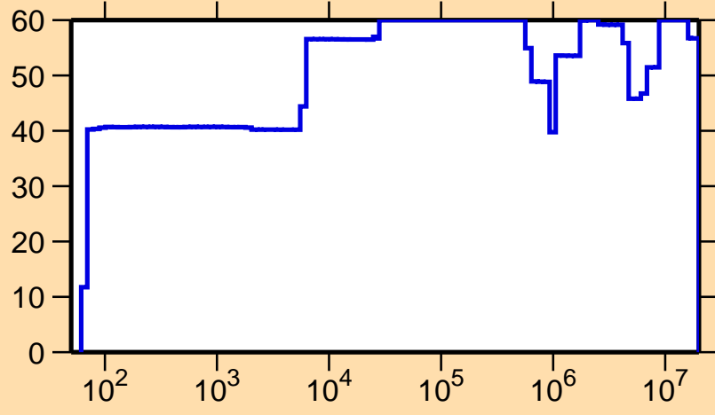
\Delta\sigma/\sigma vs. E for ^{208}\text{Fr}(n,p)
