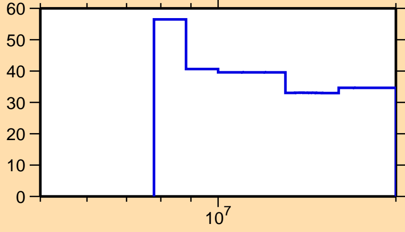
\Delta\sigma/\sigma vs. E for ^{208}\text{Fr}(n,2n)
