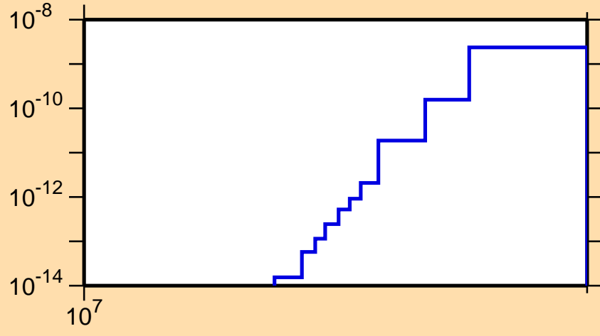
\sigma vs. E for ^{208}\text{Fr}(\text{mt } 34)
