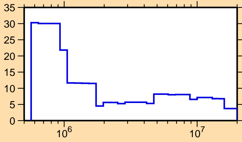
\Delta\sigma/\sigma vs. E for ^{208}\text{Fr}(n,\text{tot.})
