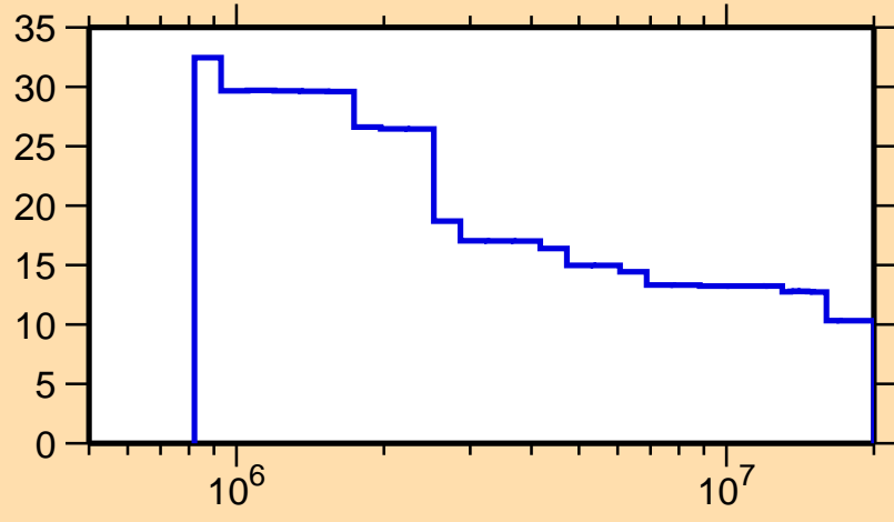
\Delta\sigma/\sigma vs. E for ^{208}\text{Fr}(n,\text{nonel.})
