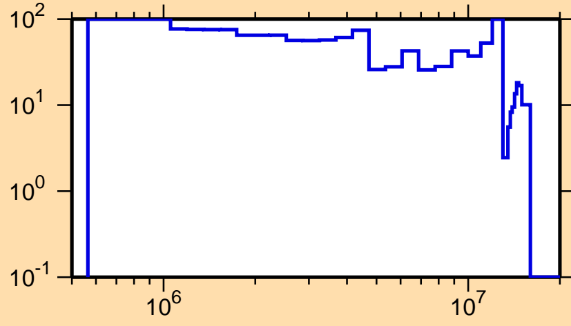
\Delta\sigma/\sigma vs. E for ^{208}\text{Fr}(n,n_1)
