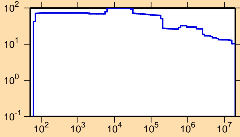
\Delta\sigma/\sigma vs. E for ^{208}\text{Fr}(n,\text{nonel.})
