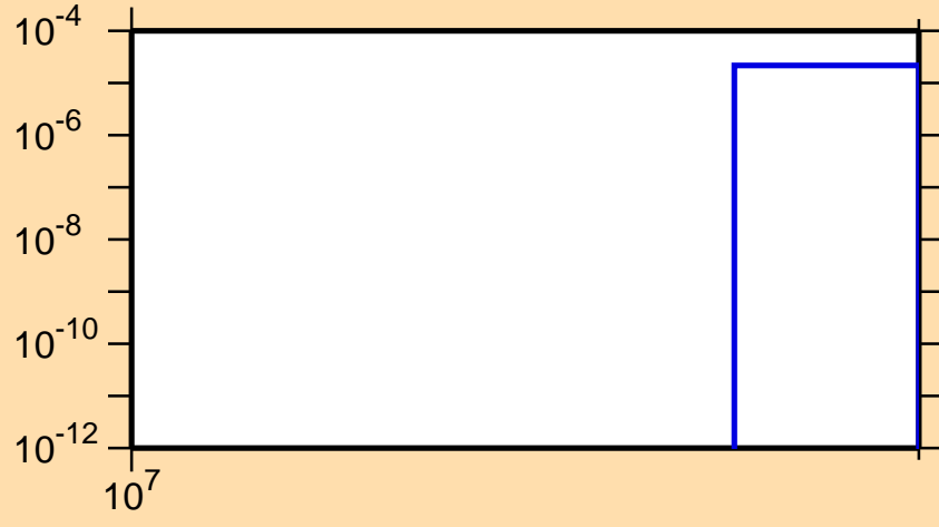
\sigma vs. E for ^{208}\text{Fr}(n,3n\alpha)
