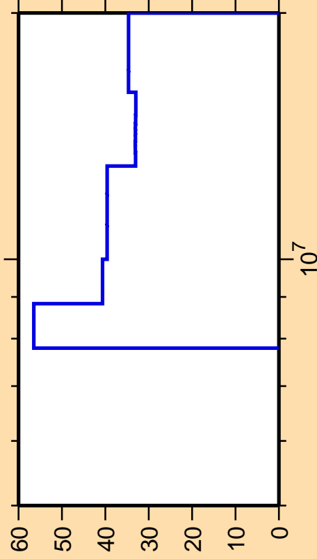
\Delta\sigma/\sigma vs. E for ^{208}\text{Fr}(n,2n)
