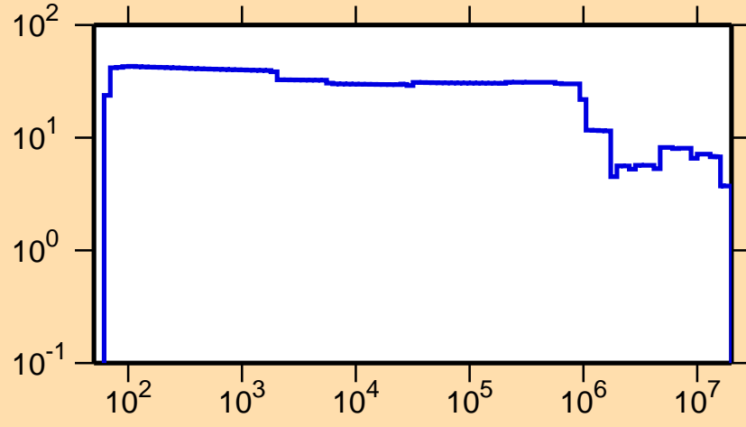
\Delta\sigma/\sigma vs. E for ^{208}\text{Fr}(n,\text{tot.})
