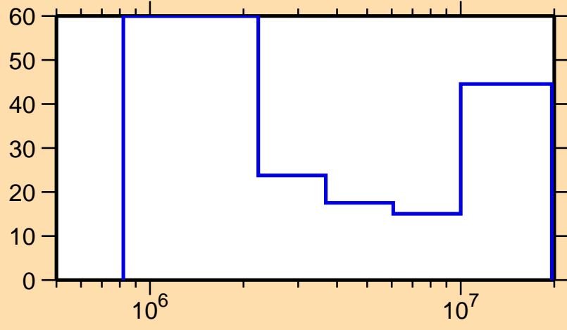
\Delta\sigma/\sigma vs. E for ^{208}\text{Fr}(n,n\text{cont.})
