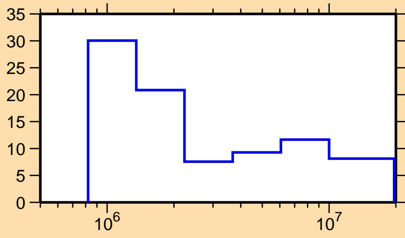
\Delta\sigma/\sigma vs. E for ^{208}\text{Fr}(n, el.)
