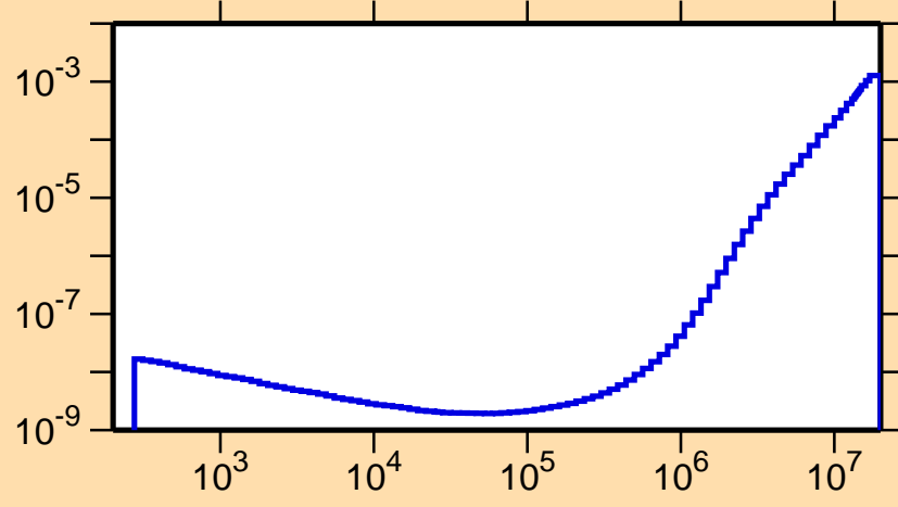
\sigma vs. E for ^{209}\text{Fr}(n,p\alpha)
