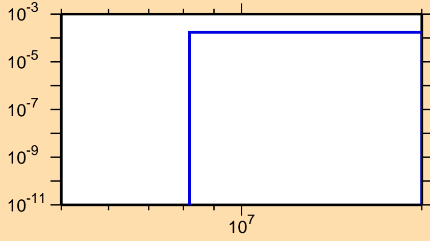
\sigma vs. E for ^{209}\text{Fr}(n,t)
