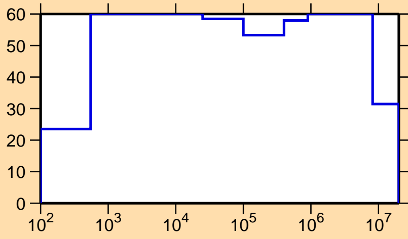
\Delta\sigma/\sigma vs. E for ^{209}\text{Fr}(n,p)
