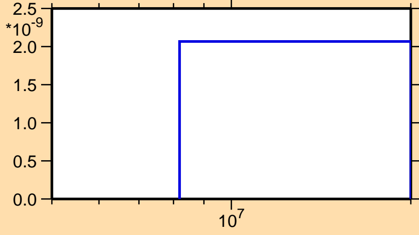
\sigma vs. E for ^{209}\text{Fr}(n,nt)
