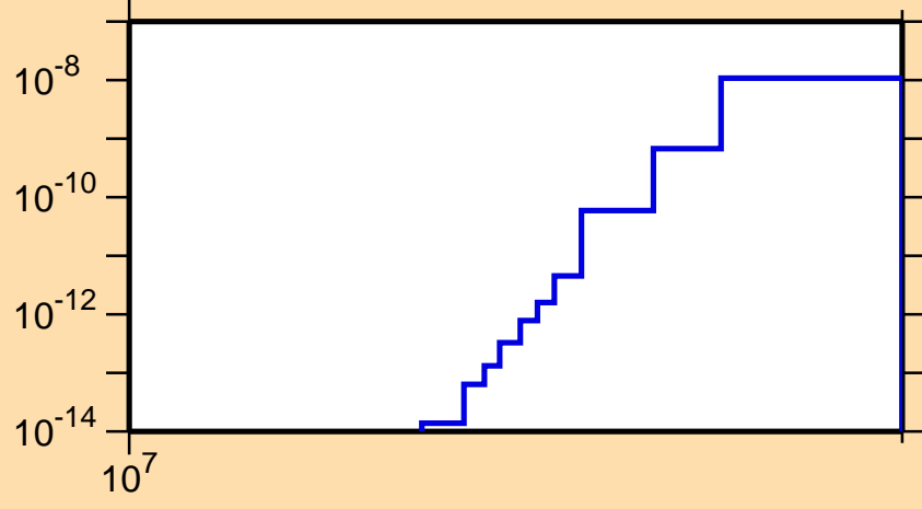
\sigma vs. E for ^{210}\text{Fr}(n,pt)
