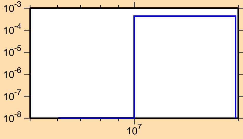
\sigma vs. E for ^{210}\text{Fr}(n,t)
