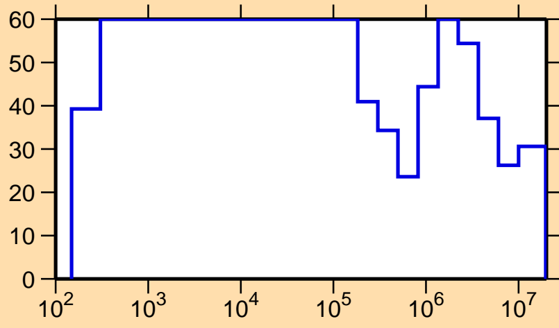
\Delta\sigma/\sigma vs. E for ^{210}\text{Fr}(n,p)
