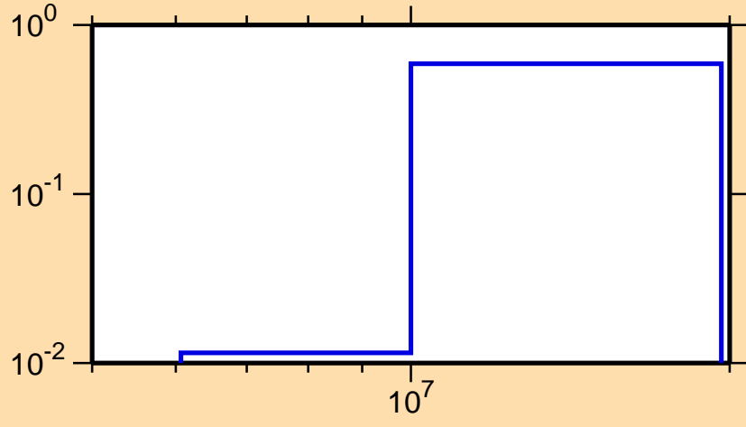
\sigma vs. E for ^{210}\text{Fr}(n,2n\alpha)
