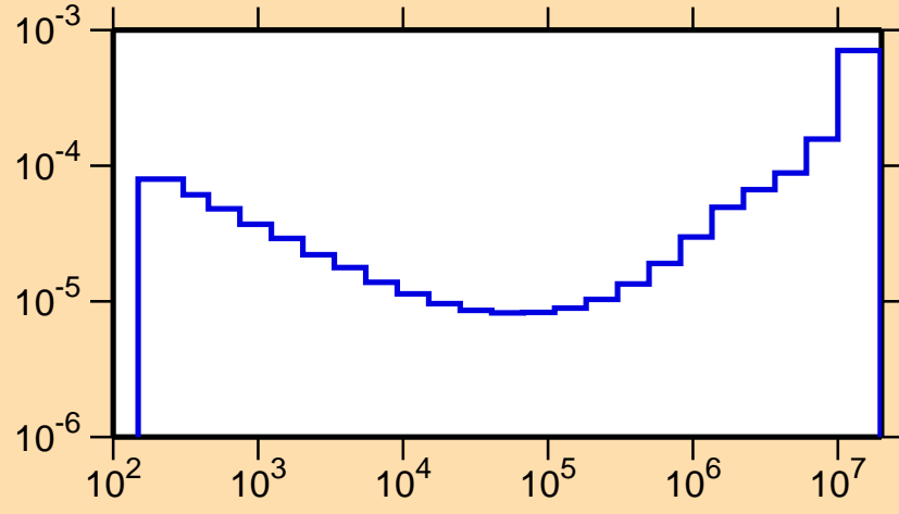
\sigma vs. E for ^{210}\text{Fr}(n,p\alpha)
