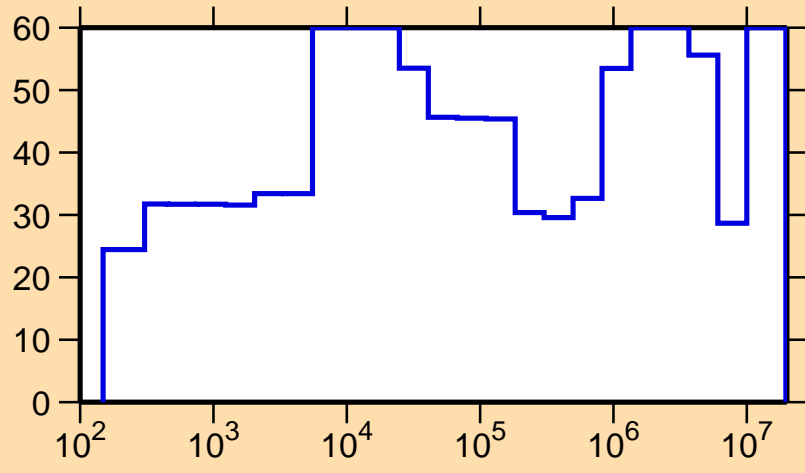
\Delta\sigma/\sigma vs. E for ^{210}\text{Fr}(n,\gamma)
