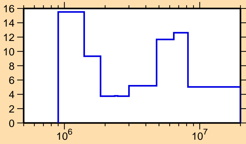
\Delta\sigma/\sigma vs. E for ^{210}\text{Fr}(n, el.)
