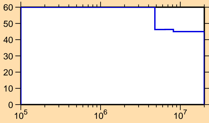
\Delta\sigma/\sigma vs. E for ^{210}\text{Fr}(n,n_1)
