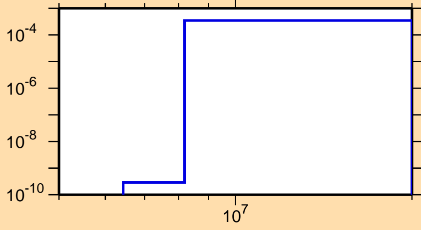
\sigma vs. E for ^{210}\text{Fr}(n,t)
