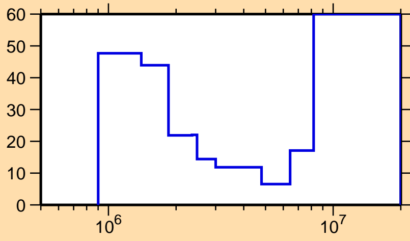
\Delta\sigma/\sigma vs. E for ^{210}\text{Fr}(n,ncont.)
