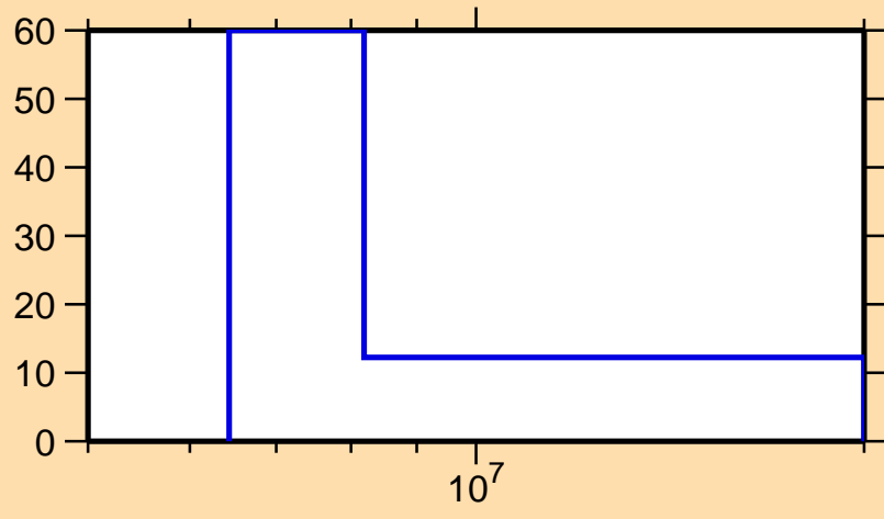
\Delta\sigma/\sigma vs. E for ^{210}\text{Fr}(n,2n)
