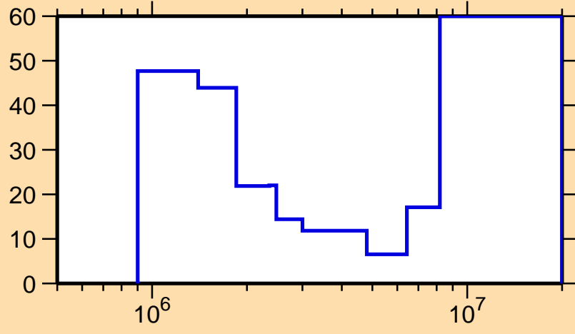
\Delta\sigma/\sigma vs. E for ^{210}\text{Fr}(n,n\text{cont.})
