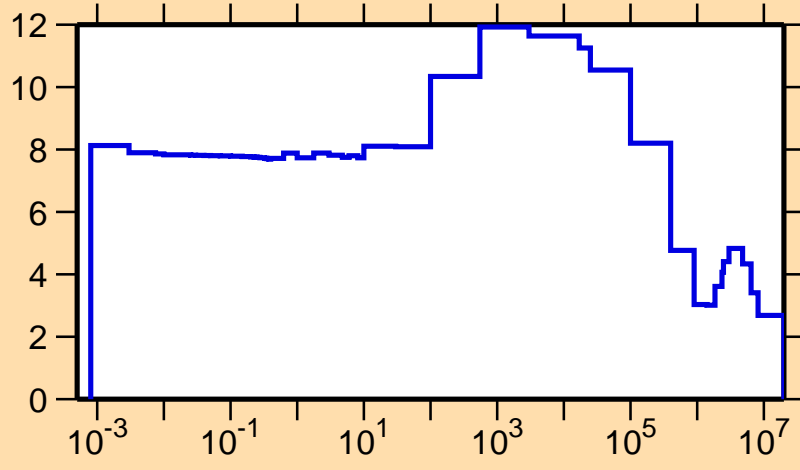
\sigma vs. E for ^{210}\text{Fr}(n,\text{el.})
