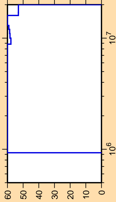
\Delta\sigma/\sigma vs. E for ^{212}\text{Fr}(n,n\alpha)
