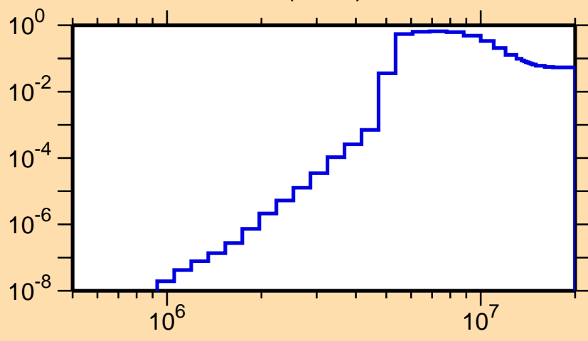
\sigma vs. E for ^{212}\text{Fr}(n,n\alpha)
