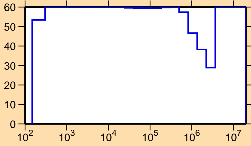
\Delta\sigma/\sigma vs. E for ^{212}\text{Fr}(n,\gamma)
