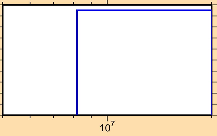
\sigma vs. E for ^{212}\text{Fr}(n,\text{He3})
