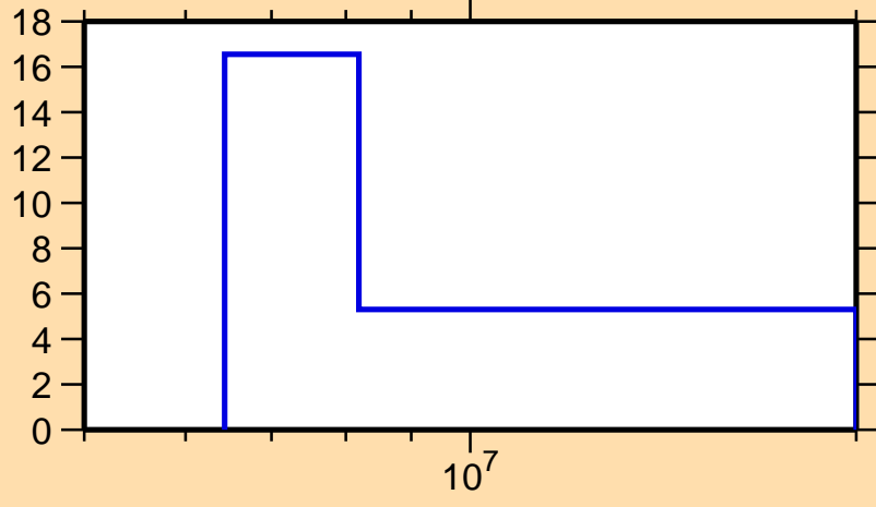
\Delta\sigma/\sigma vs. E for ^{212}\text{Fr}(n,\text{el.})
