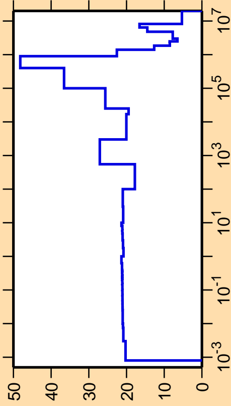
\Delta\sigma/\sigma vs. E for ^{212}\text{Fr}(n,\text{el.})
