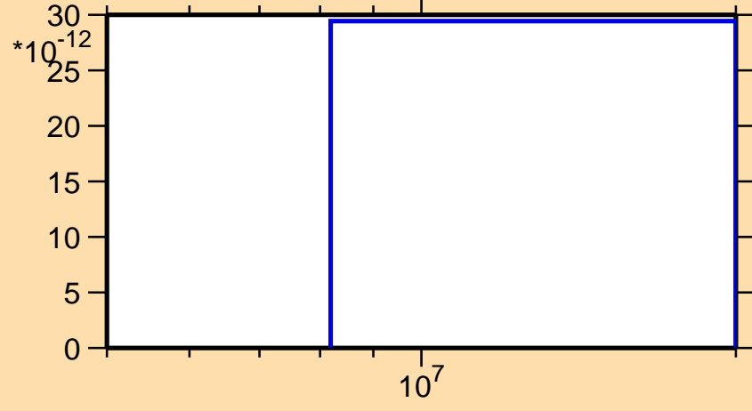
\sigma vs. E for ^{212}\text{Fr}(n,\text{pt})
