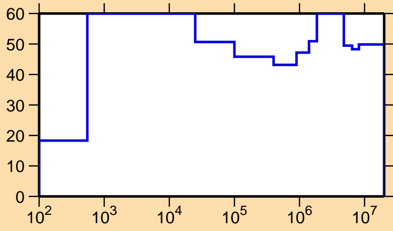
\Delta\sigma/\sigma vs. E for ^{212}\text{Fr}(n,p)
