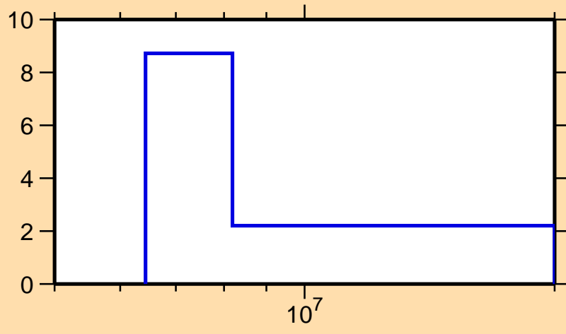
\Delta\sigma/\sigma vs. E for ^{212}\text{Fr}(n,\text{tot.})
