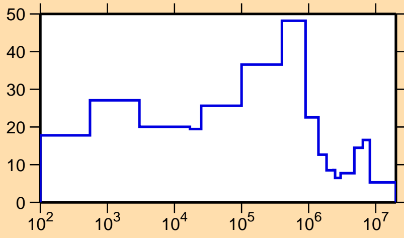
\Delta\sigma/\sigma vs. E for ^{212}\text{Fr}(n,\text{el.})
