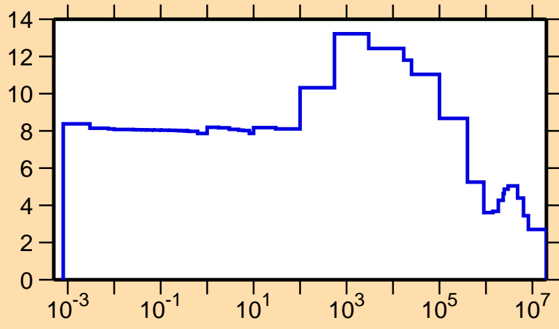
\sigma vs. E for ^{212}\text{Fr}(n,\text{el.})
