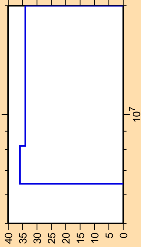
\Delta\sigma/\sigma vs. E for ^{212}\text{Fr}(n,n_1)
