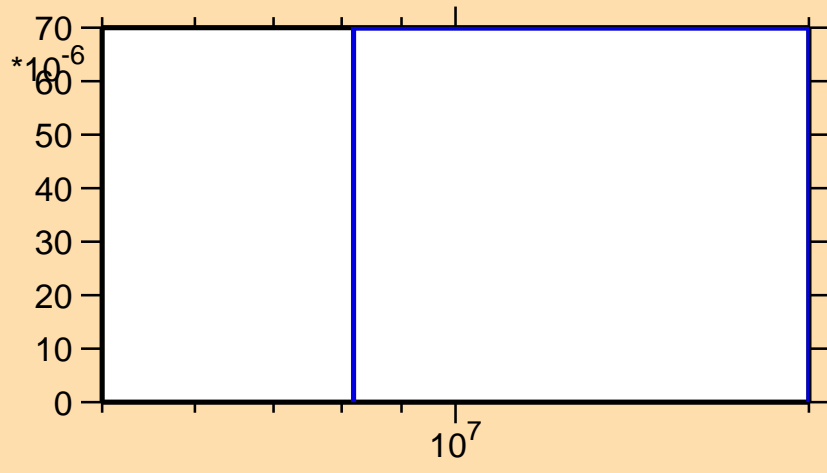
\sigma vs. E for ^{212}\text{Fr}(n,2np)
