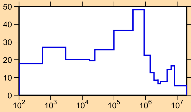
\Delta\sigma/\sigma vs. E for ^{212}\text{Fr}(n,el.)
