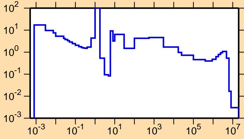
\sigma vs. E for ^{212}\text{Fr}(n,\gamma)
