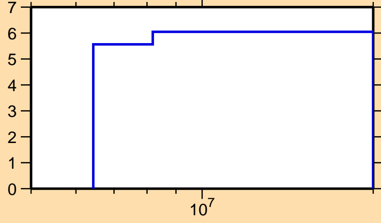
\Delta\sigma/\sigma vs. E for ^{212}\text{Fr}(n,\text{nonel.})
