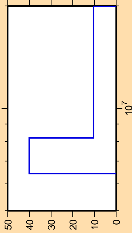
\Delta\sigma/\sigma vs. E for ^{212}\text{Fr}(n,2n)
