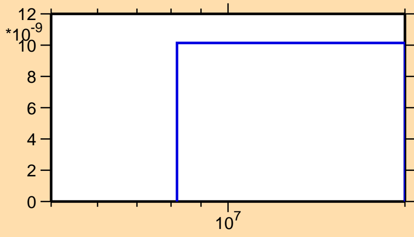
\sigma vs. E for ^{212}\text{Fr}(n,nt)
