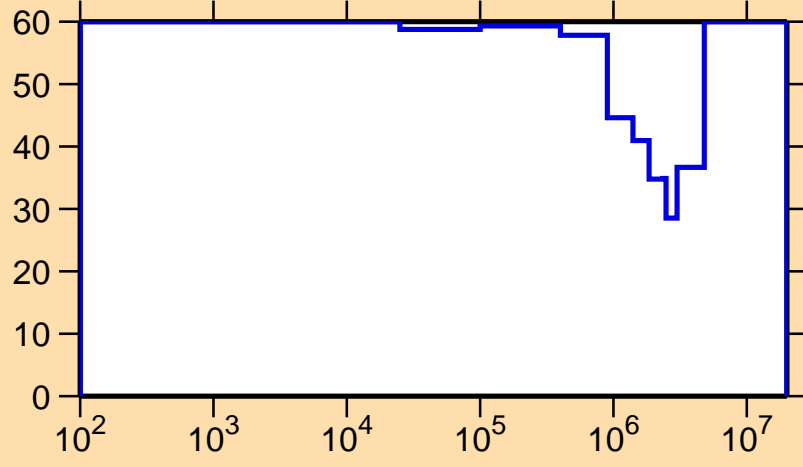
\Delta\sigma/\sigma vs. E for ^{212}\text{Fr}(n,\gamma)
