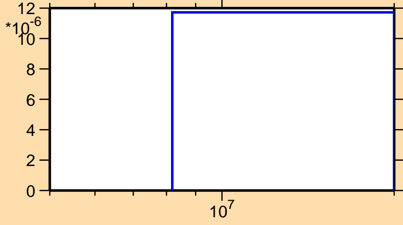
\sigma vs. E for ^{212}\text{Fr}(n,3n\alpha)
