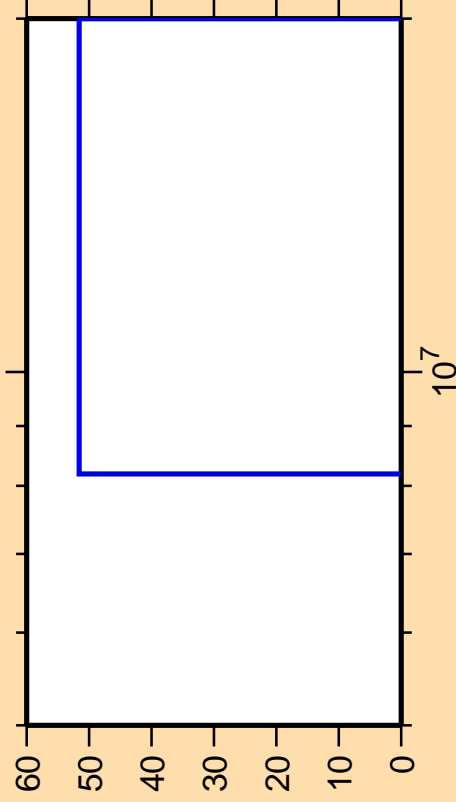
\Delta\sigma/\sigma vs. E for ^{212}\text{Fr}(n,3n)
