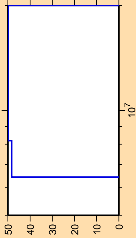
\Delta\sigma/\sigma vs. E for ^{212}\text{Fr}(n,p)
