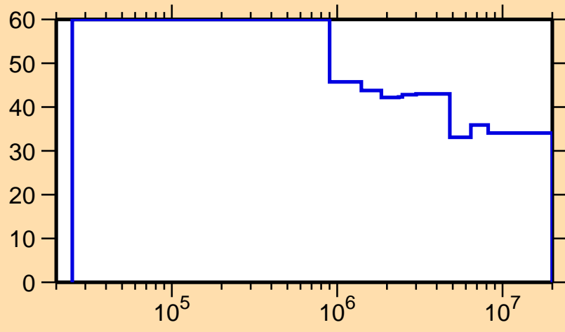
\Delta\sigma/\sigma vs. E for ^{212}\text{Fr}(n,n_1)
