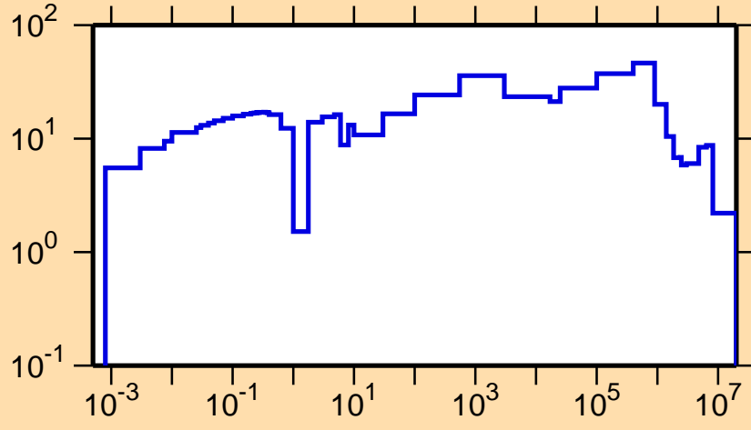
\Delta\sigma/\sigma vs. E for ^{212}\text{Fr}(n,\text{tot.})
