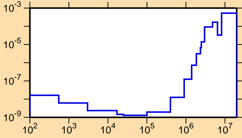
\sigma vs. E for ^{212}\text{Fr}(n,p\alpha)
