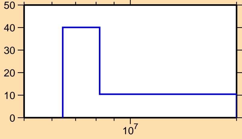
\Delta\sigma/\sigma vs. E for ^{212}\text{Fr}(n,2n)
