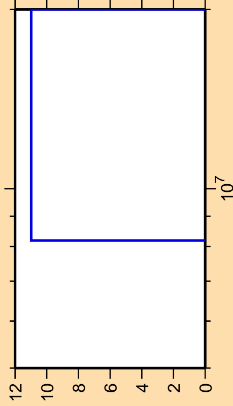
\Delta\sigma/\sigma vs. E for ^{212}\text{Fr}(\text{mt } 34)
