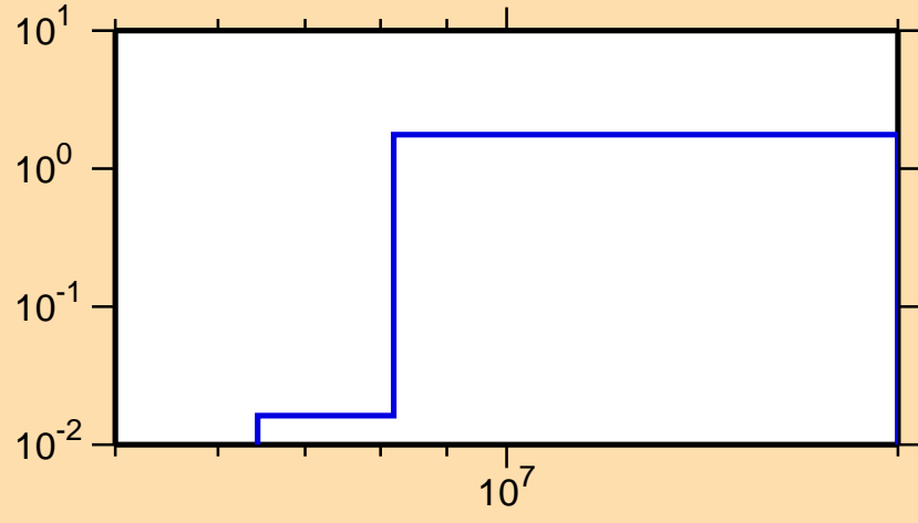
\sigma vs. E for ^{212}\text{Fr}(n,2n)
