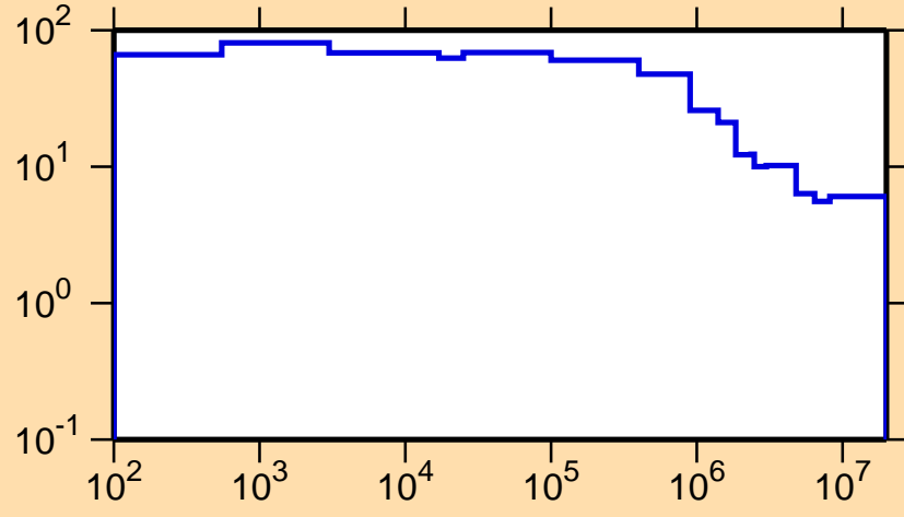
\Delta\sigma/\sigma vs. E for ^{212}\text{Fr}(n,\text{nonel.})
