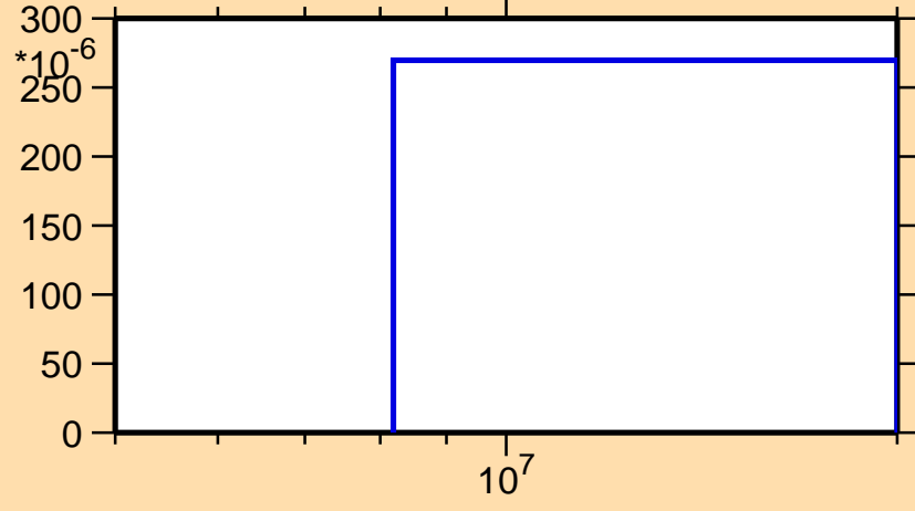
\sigma vs. E for ^{212}\text{Fr}(n,3n)
