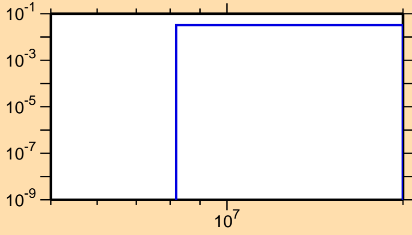
\sigma vs. E for ^{212}\text{Fr}(n,2n\alpha)
