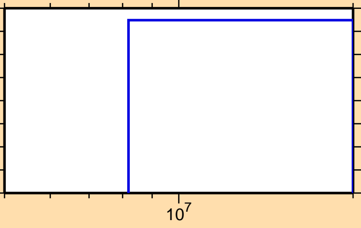
\sigma vs. E for ^{212}\text{Fr}(n,\text{nd})
