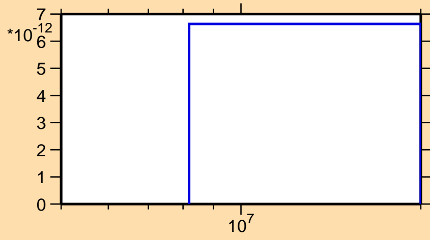
\sigma vs. E for ^{212}\text{Fr}(\text{mt } 34)
