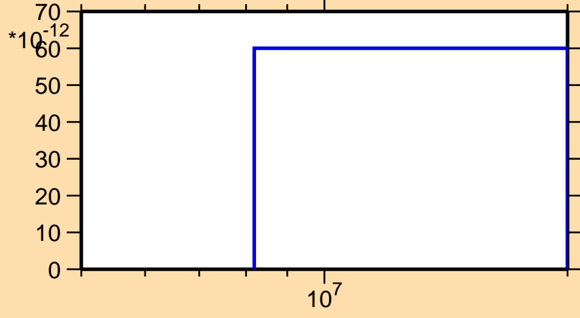
\sigma vs. E for ^{212}\text{Fr}(n,\text{pd})
