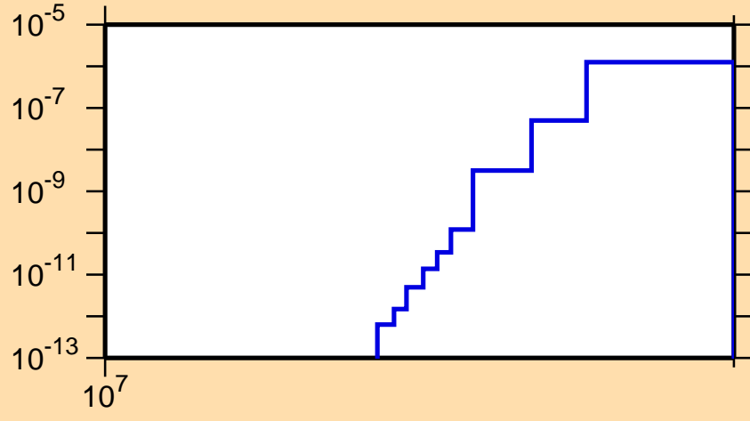
\sigma vs. E for ^{213}\text{Fr}(n,nt)
