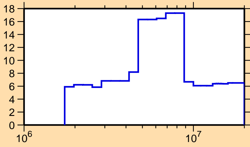
\Delta\sigma/\sigma vs. E for ^{213}\text{Fr}(n, el.)
