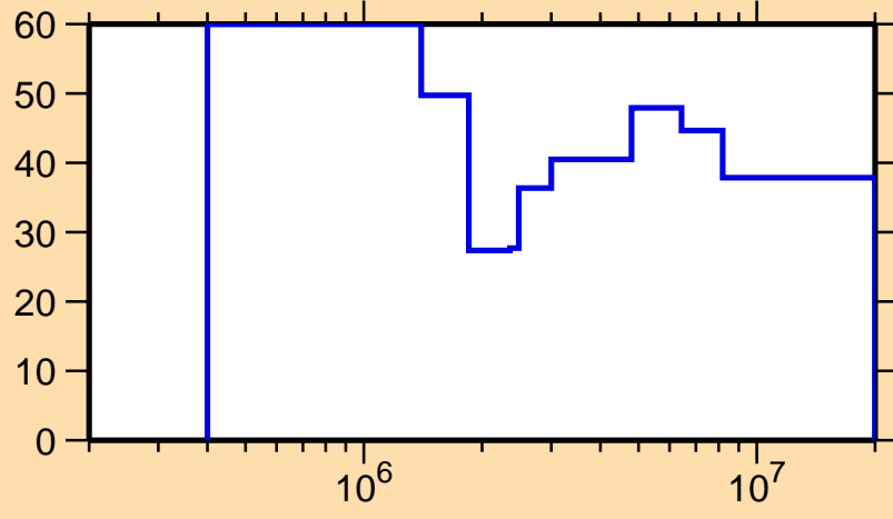
\Delta\sigma/\sigma vs. E for ^{213}\text{Fr}(n,n_1)
