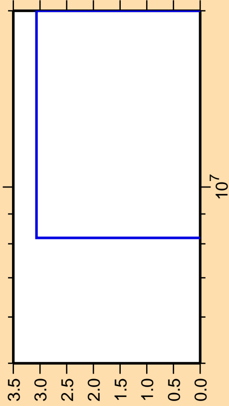
\Delta\sigma/\sigma vs. E for ^{213}\text{Fr}(\text{mt } 34)
