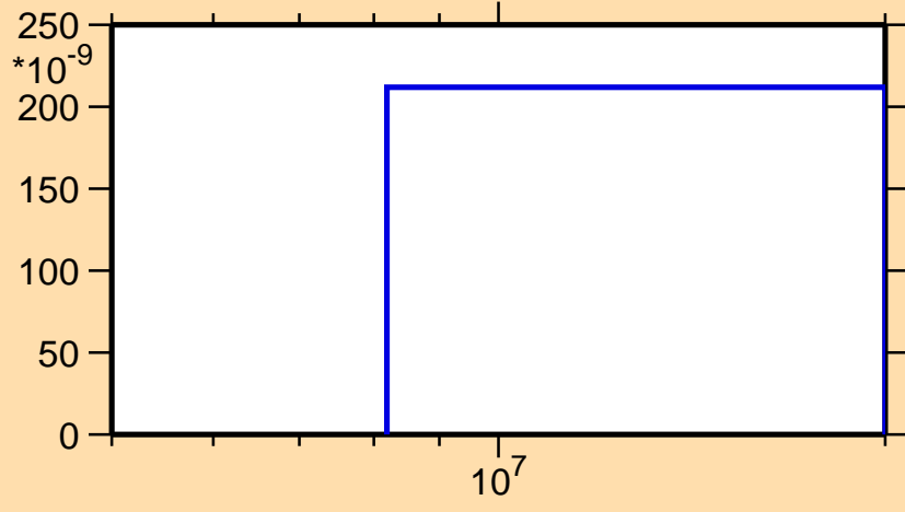
\sigma vs. E for ^{213}\text{Fr}(n,\text{nd})
