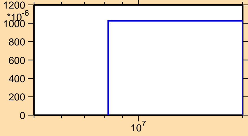
\sigma vs. E for ^{213}\text{Fr}(n,3n)
