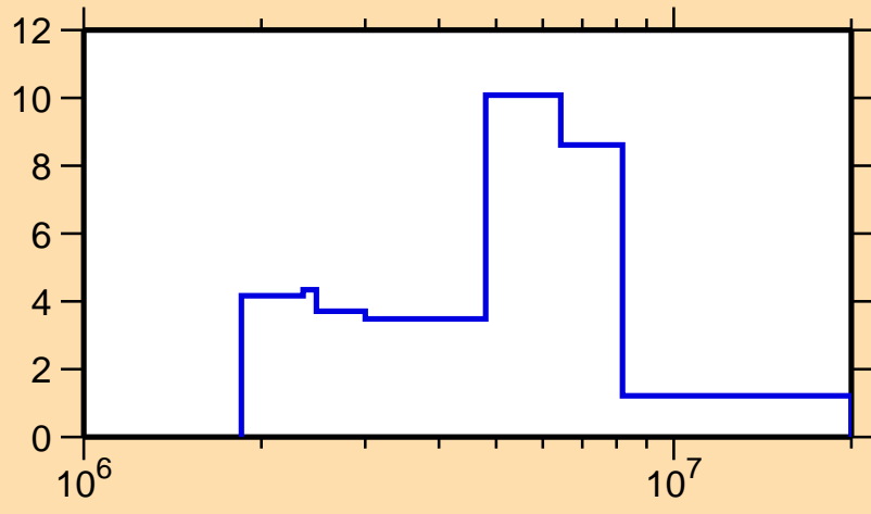
\Delta\sigma/\sigma vs. E for ^{213}\text{Fr}(n,\text{tot.})
