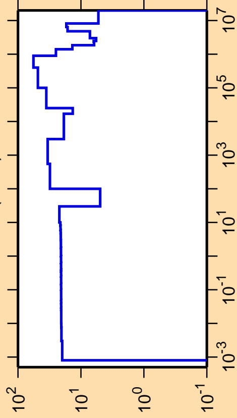
\Delta\sigma/\sigma vs. E for ^{213}\text{Fr}(n,\text{el.})
