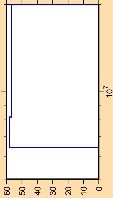
\Delta\sigma/\sigma vs. E for ^{213}\text{Fr}(n,p)
