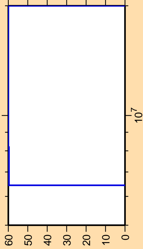
\Delta\sigma/\sigma vs. E for ^{213}\text{Fr}(n,n\text{cont.})
