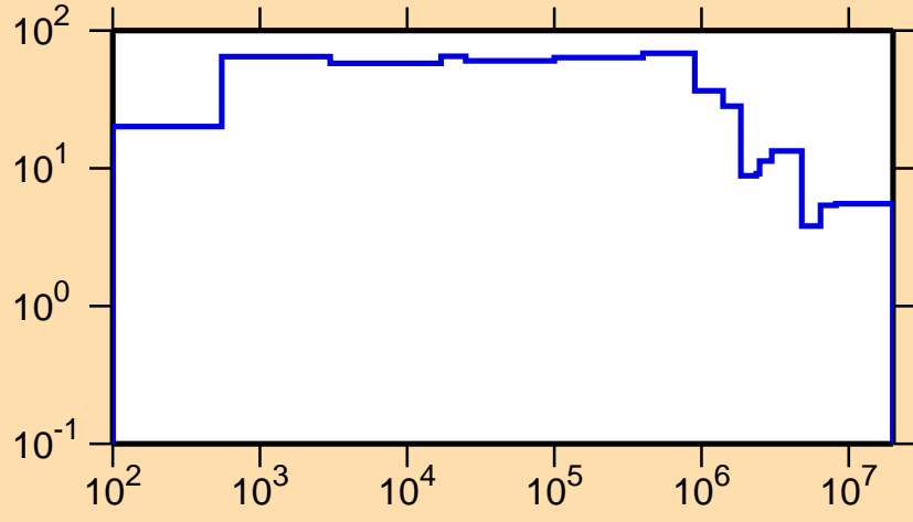
\Delta\sigma/\sigma vs. E for ^{213}\text{Fr}(n,\text{nonel.})
