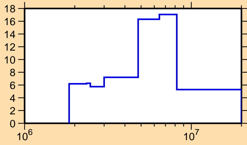
\Delta\sigma/\sigma vs. E for ^{213}\text{Fr}(n,\text{el.})
