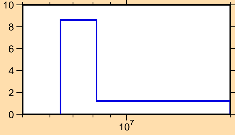
\Delta\sigma/\sigma vs. E for ^{213}\text{Fr}(n,\text{tot.})
