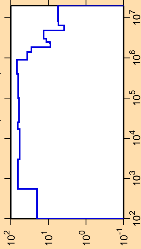
\Delta\sigma/\sigma vs. E for ^{213}\text{Fr}(n,\text{nonel.})
