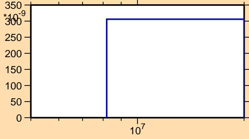
\sigma vs. E for ^{213}\text{Fr}(n,3n\alpha)
