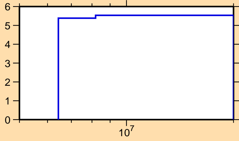
\Delta\sigma/\sigma vs. E for ^{213}\text{Fr}(n,\text{nonel.})
