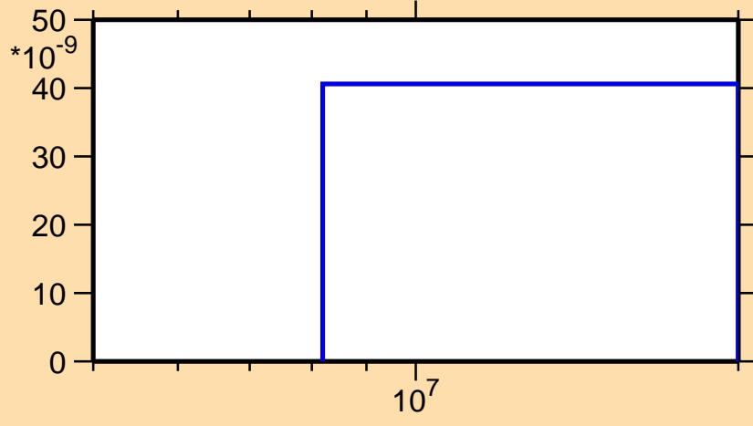
\sigma vs. E for ^{213}\text{Fr}(n,\text{He3})
