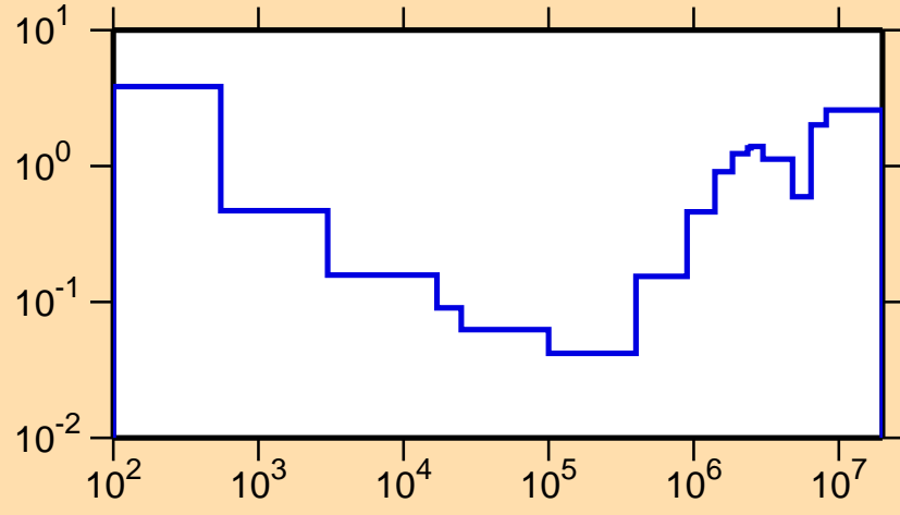
\sigma vs. E for ^{213}\text{Fr}(n,\text{nonel.})
