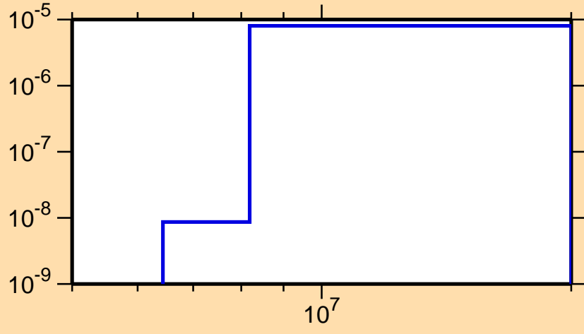
\sigma vs. E for ^{213}\text{Fr}(\text{mt } 45)
