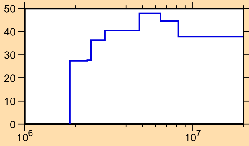
\Delta\sigma/\sigma vs. E for ^{213}\text{Fr}(n,n_1)
