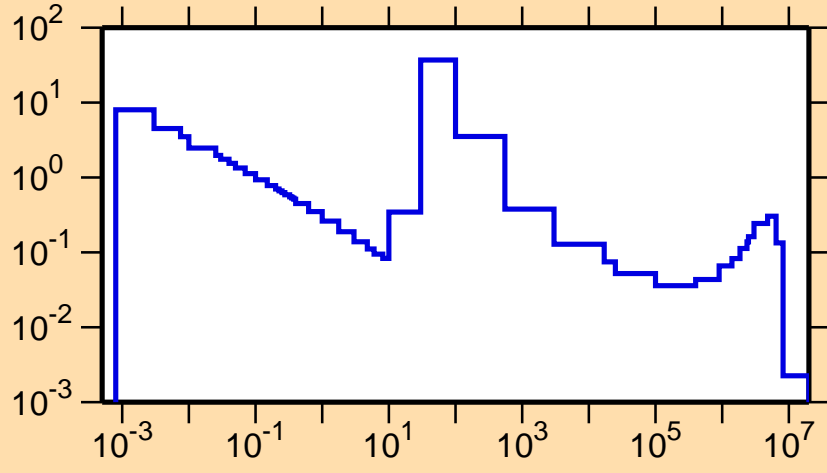
\sigma vs. E for ^{213}\text{Fr}(n,\gamma)
