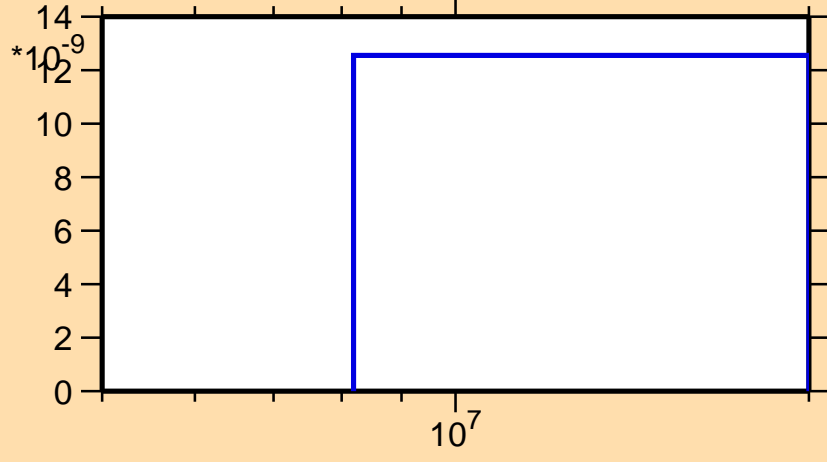
\sigma vs. E for ^{213}\text{Fr}(n,nt)
