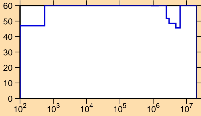
\Delta\sigma/\sigma vs. E for ^{213}\text{Fr}(n,\gamma)
