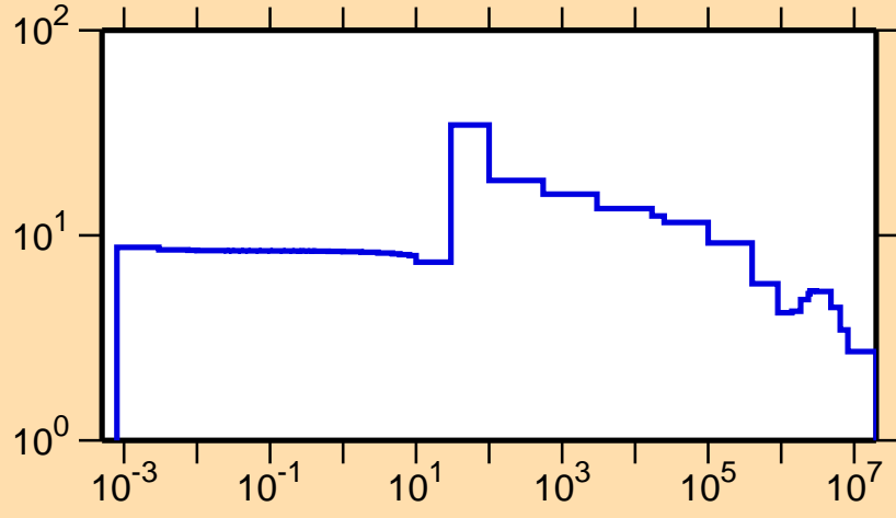
\sigma vs. E for ^{213}\text{Fr}(n,\text{el.})
