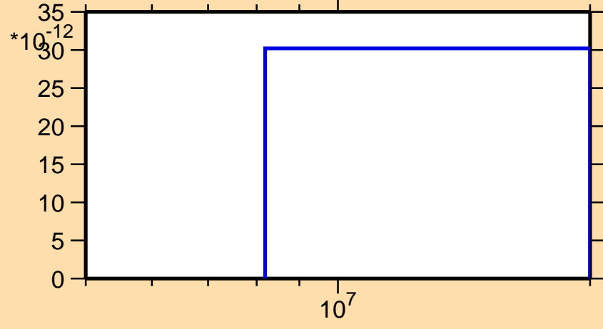
\sigma vs. E for ^{213}\text{Fr}(n,\text{pd})
