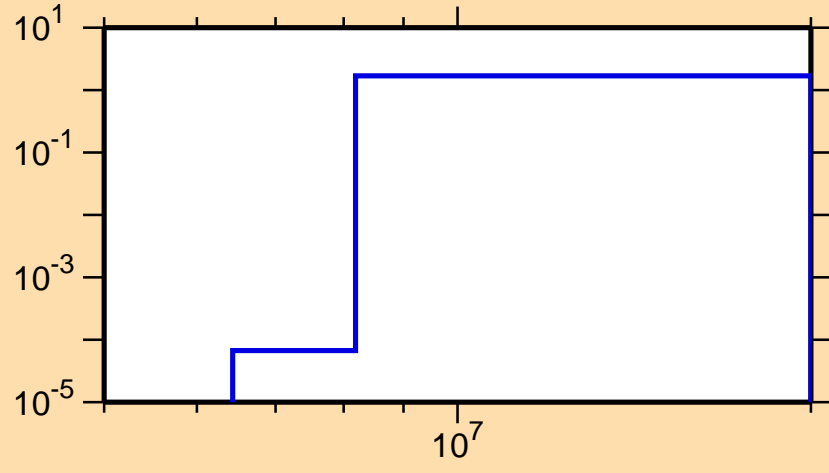
\sigma vs. E for ^{213}\text{Fr}(n,2n)
