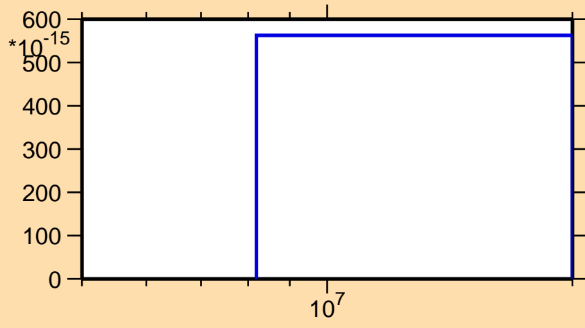
\sigma vs. E for ^{213}\text{Fr}(n,\text{pt})
