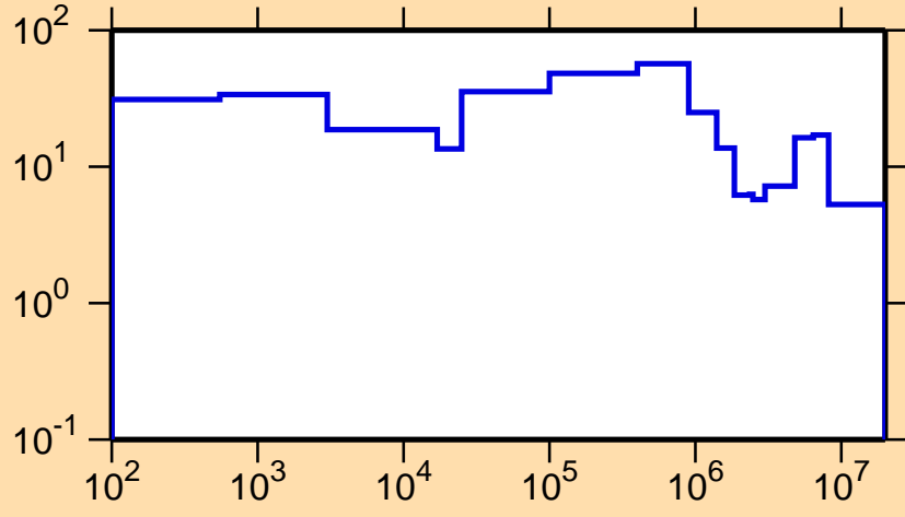
\Delta\sigma/\sigma vs. E for ^{213}\text{Fr}(n,\text{el.})
