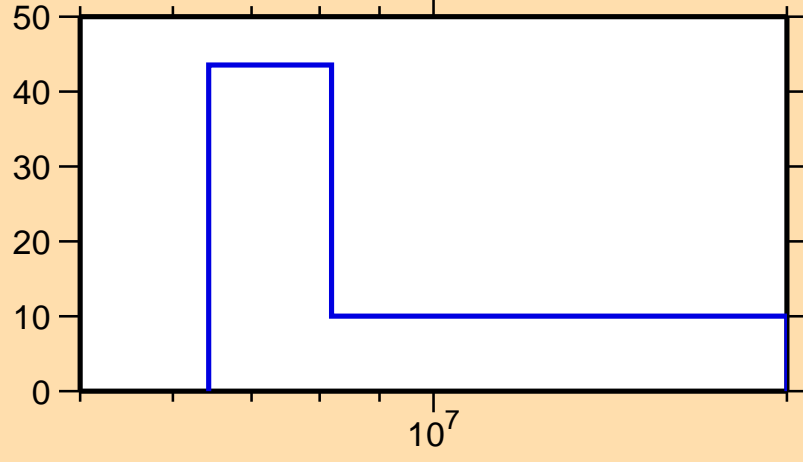
\Delta\sigma/\sigma vs. E for ^{213}\text{Fr}(n,2n)
