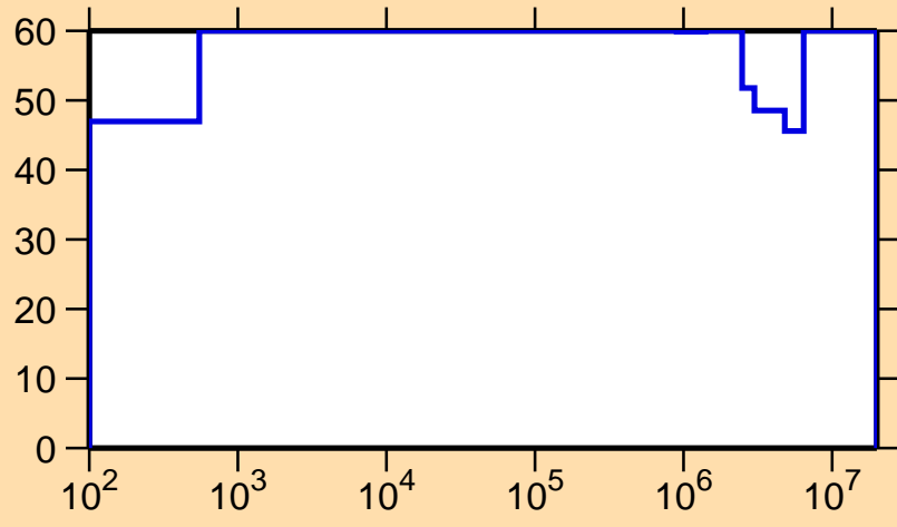
\Delta\sigma/\sigma vs. E for ^{213}\text{Fr}(n,\gamma)
