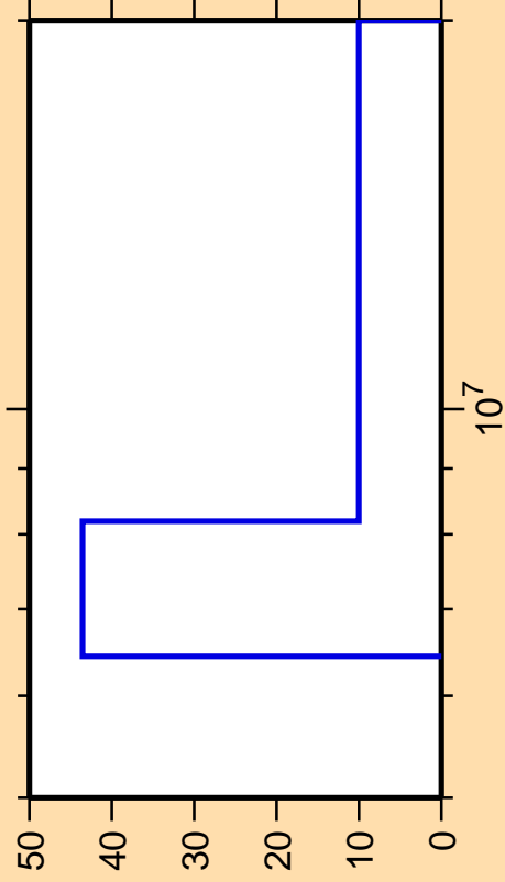
\Delta\sigma/\sigma vs. E for ^{213}\text{Fr}(n,2n)
