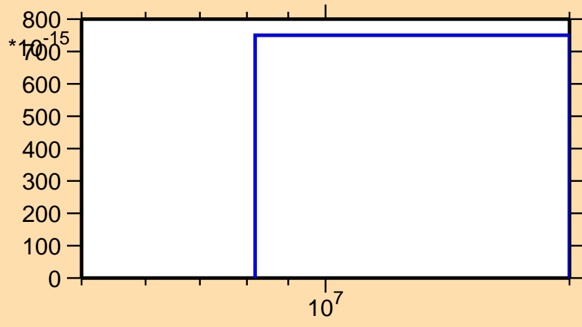
\sigma vs. E for ^{213}\text{Fr}(\text{mt } 34)
