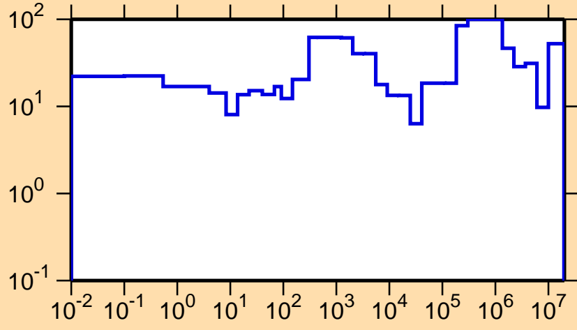
\Delta\sigma/\sigma vs. E for ^{221}\text{Fr}(n,el.)
