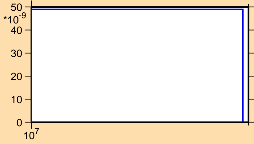
\sigma vs. E for ^{221}\text{Fr}(n,2np)
