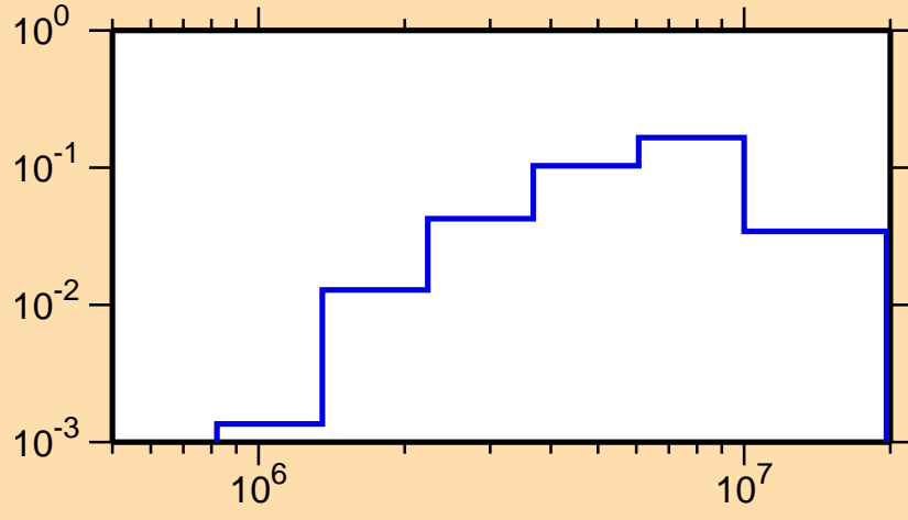
\sigma vs. E for ^{221}\text{Fr}(n,n\alpha)
