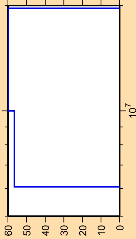
\Delta\sigma/\sigma vs. E for ^{221}\text{Fr}(\text{mt117})
