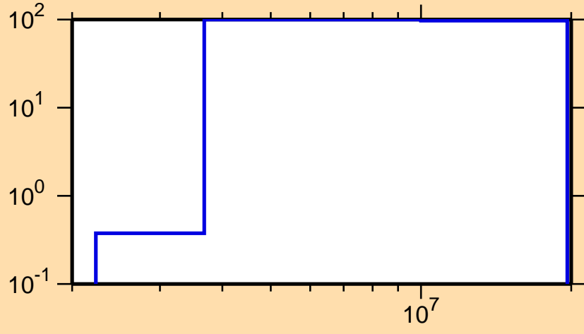
\Delta\sigma/\sigma vs. E for ^{221}\text{Fr}(n,p)
