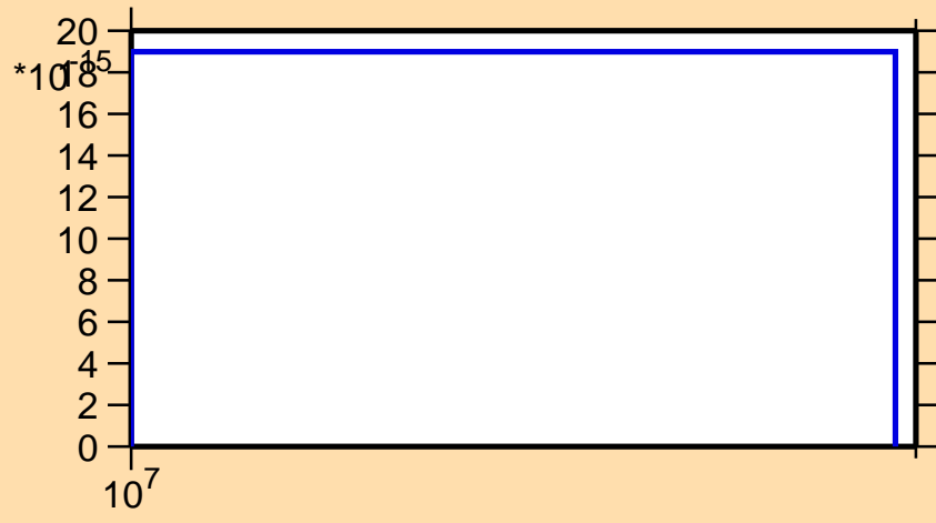
\sigma vs. E for ^{221}\text{Fr}(\text{mt } 42)
