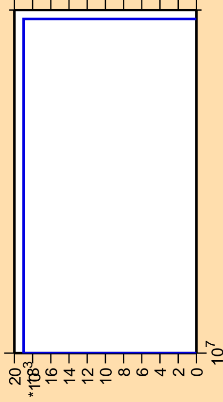
\Delta\sigma/\sigma vs. E for ^{221}\text{Fr}(\text{mt } 42)
