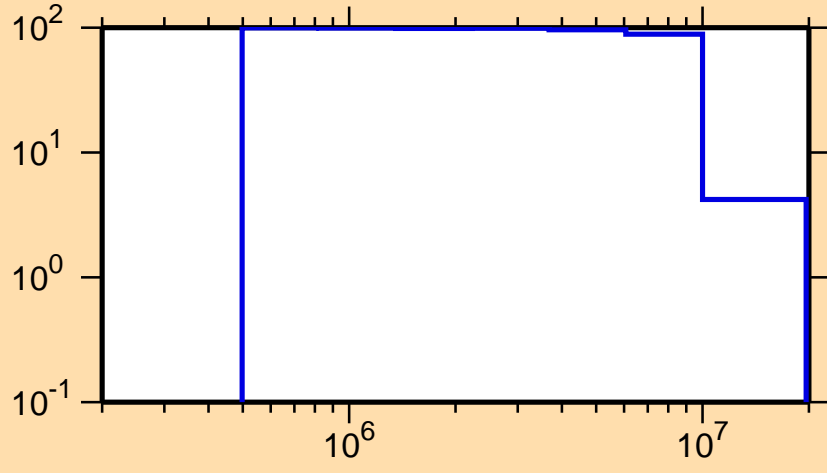
\Delta\sigma/\sigma vs. E for ^{221}\text{Fr}(n,n\text{cont.})
