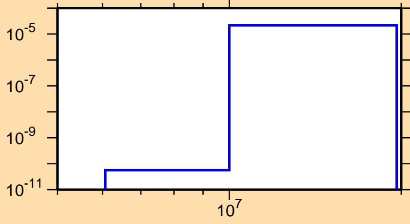
\sigma vs. E for ^{221}\text{Fr}(\text{mt117})
