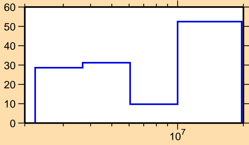
\Delta\sigma/\sigma vs. E for ^{221}\text{Fr}(n,\text{el.})
