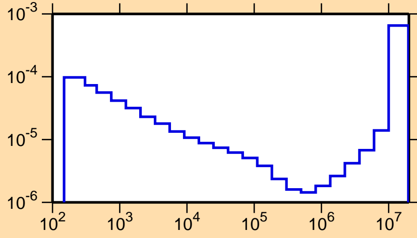
\sigma vs. E for ^{221}\text{Fr}(n,\alpha)
