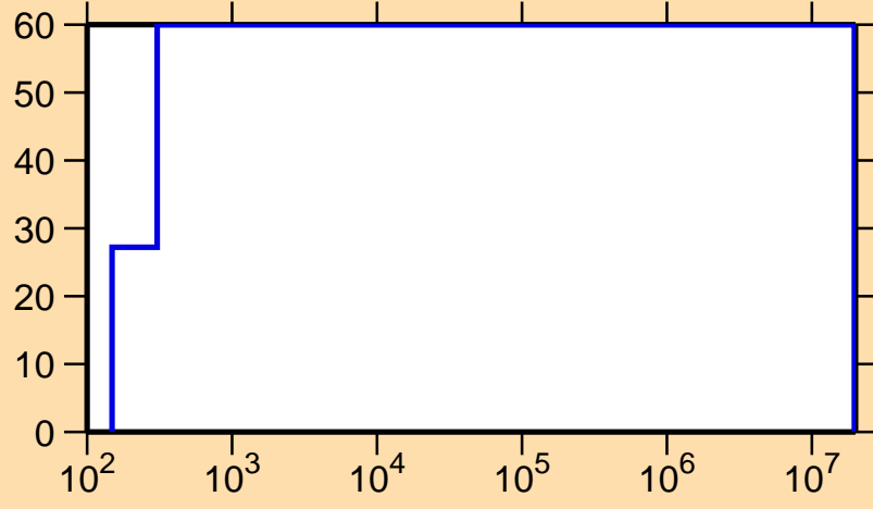
\Delta\sigma/\sigma vs. E for ^{221}\text{Fr}(n,\gamma)
