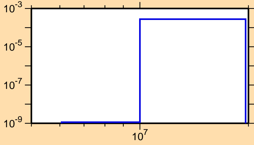
\sigma vs. E for ^{221}\text{Fr}(n,np)
