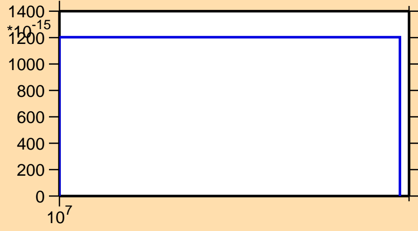
\sigma vs. E for ^{221}\text{Fr}(n,\text{He}3)
