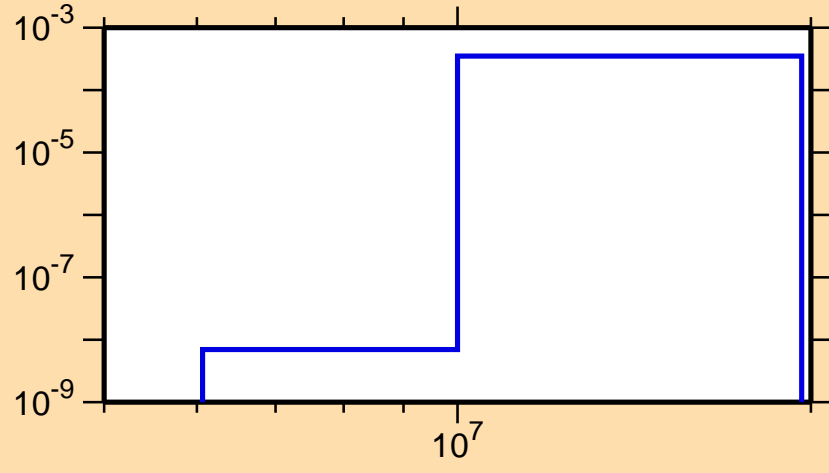
\sigma vs. E for ^{221}\text{Fr}(n,d)
