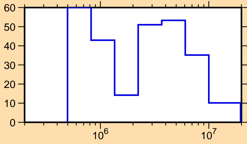
\Delta\sigma/\sigma vs. E for ^{221}\text{Fr}(n,\text{tot.})
