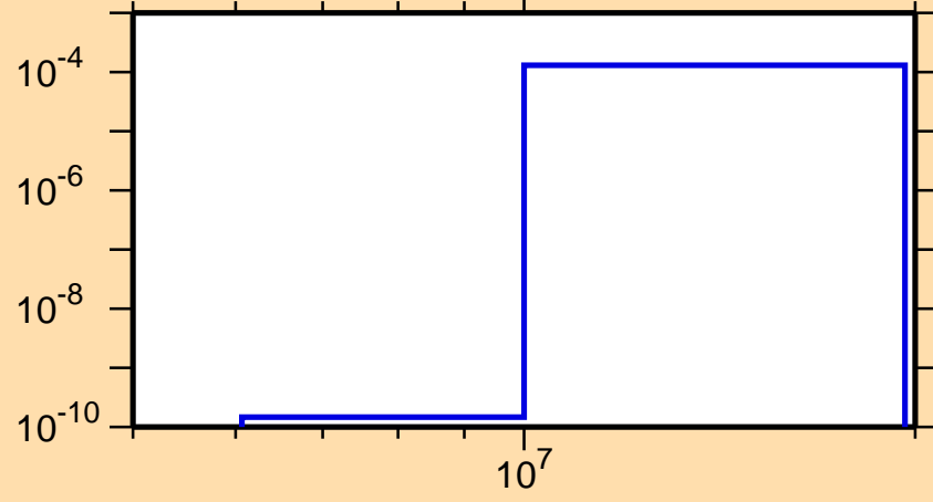
\sigma vs. E for ^{221}\text{Fr}(n,t)
