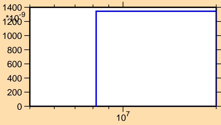
\sigma vs. E for ^{221}\text{Fr}(n,nt)
