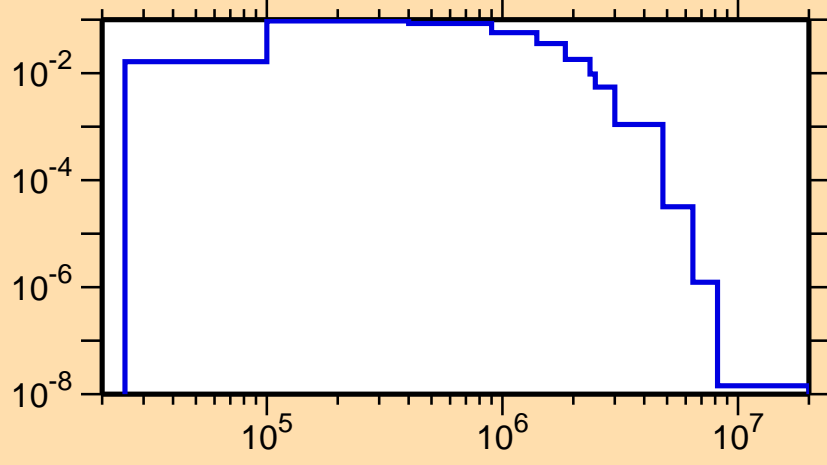
\sigma vs. E for ^{221}\text{Fr}(n,n_3)
