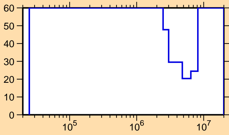
\Delta\sigma/\sigma vs. E for ^{221}\text{Fr}(n,n_1)
