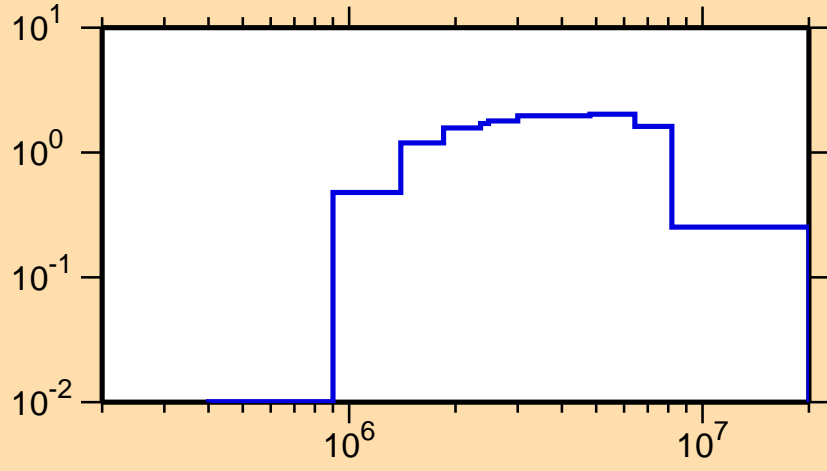
\sigma vs. E for ^{221}\text{Fr}(n,n\text{cont.})
