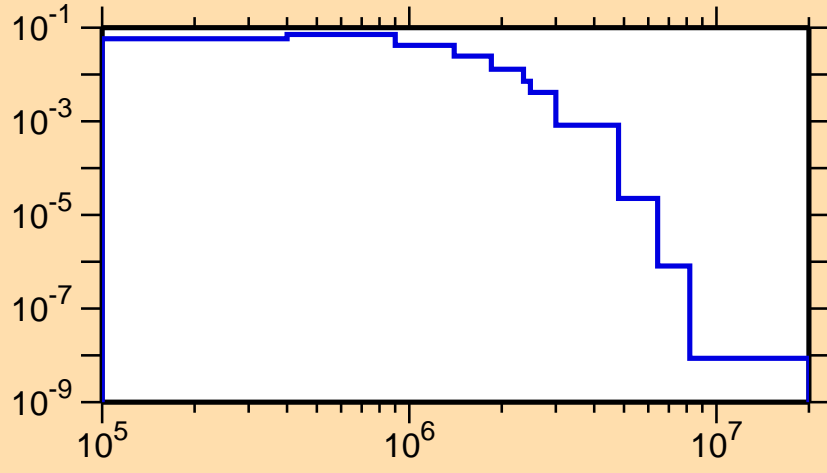
\sigma vs. E for ^{221}\text{Fr}(n,n_4)
