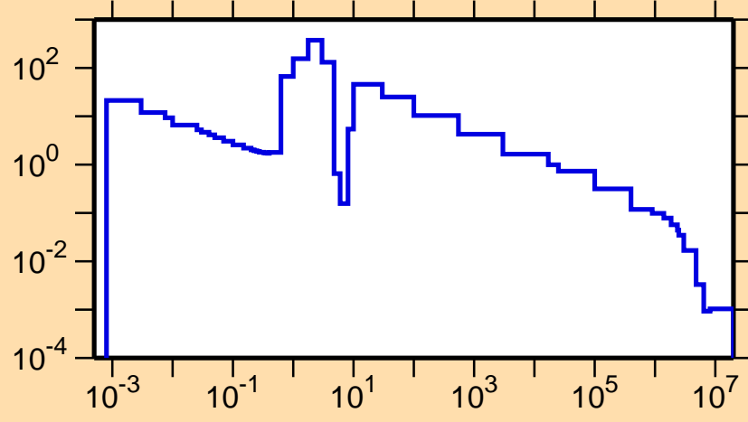
\sigma vs. E for ^{221}\text{Fr}(n,\gamma)
