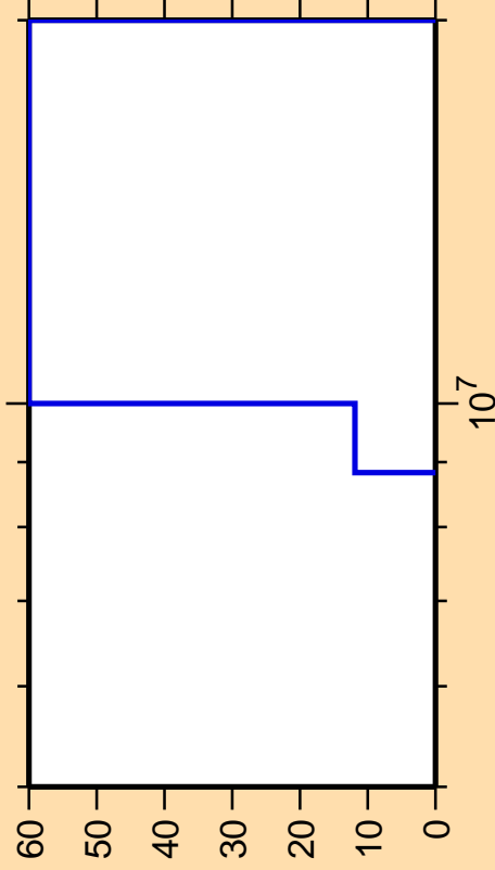
\Delta\sigma/\sigma vs. E for ^{222}\text{Fr} (mt 45)
