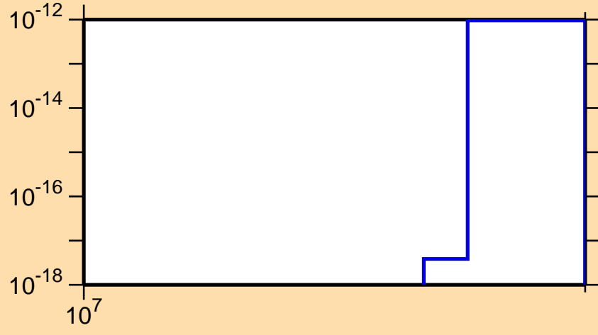
\sigma vs. E for ^{222}\text{Fr} (mt 42)
