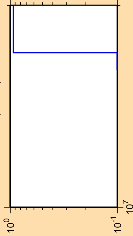
\Delta\sigma/\sigma vs. E for ^{222}\text{Fr} (mt 42)
