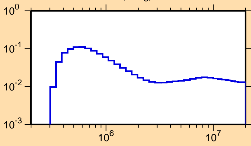
\sigma vs. E for ^{222}\text{Fr}(n,n_3)
