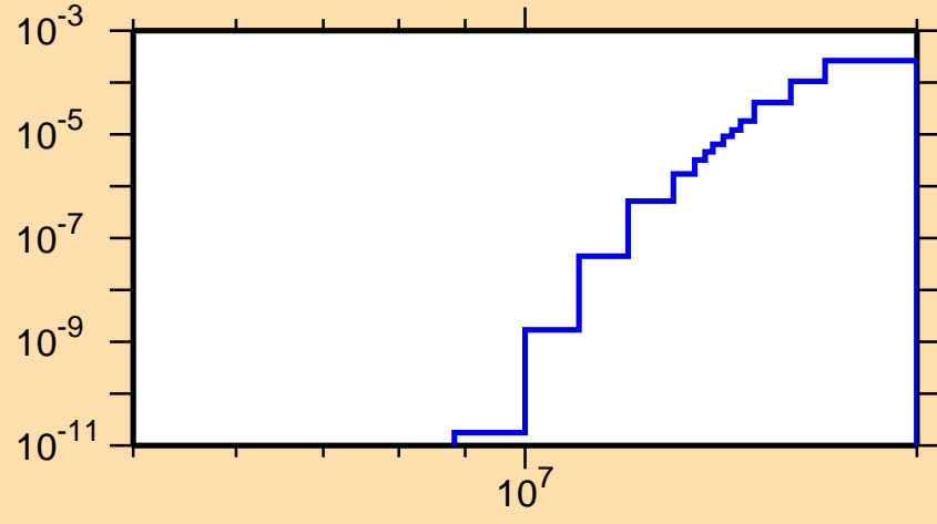
\sigma vs. E for ^{222}\text{Fr} (mt 45)
