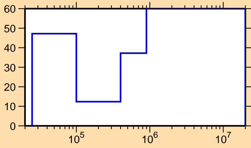
\Delta\sigma/\sigma vs. E for ^{222}\text{Fr}(n,n_1)
