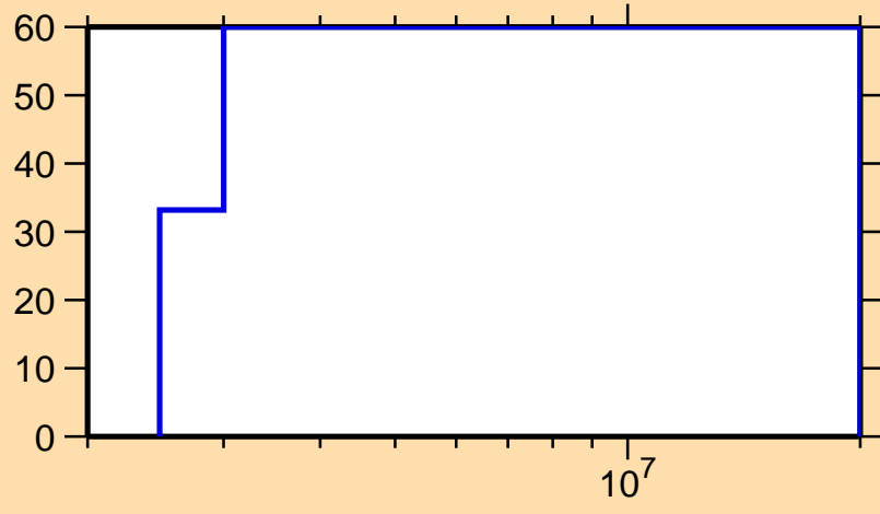
\Delta\sigma/\sigma vs. E for ^{222}\text{Fr}(n,p)
