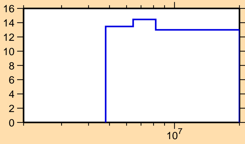
\Delta\sigma/\sigma vs. E for ^{222}\text{Fr}(n,\text{nonel.})
