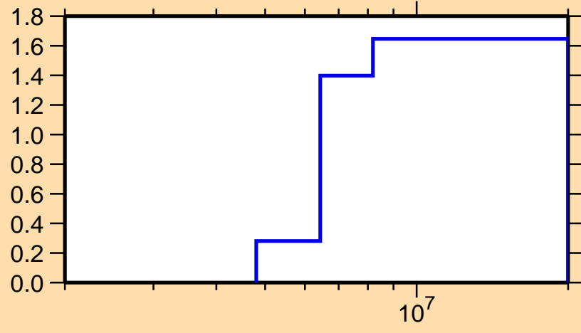
\sigma vs. E for ^{222}\text{Fr}(n,2n)
