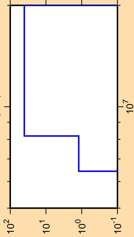
\Delta\sigma/\sigma vs. E for ^{222}\text{Fr}(n,d)
