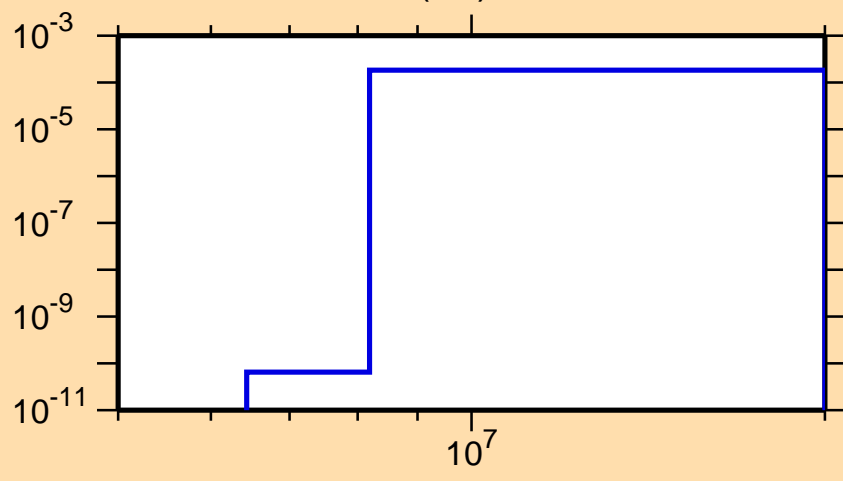
\sigma vs. E for ^{222}\text{Fr}(n,t)
