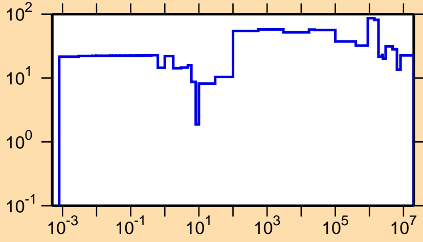
\Delta\sigma/\sigma vs. E for ^{222}\text{Fr}(n,el.)
