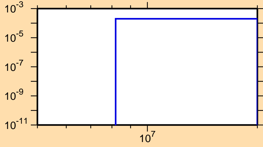
\sigma vs. E for ^{222}\text{Fr}(n,d)
