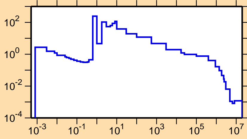
\sigma vs. E for ^{222}\text{Fr}(n,\gamma)
