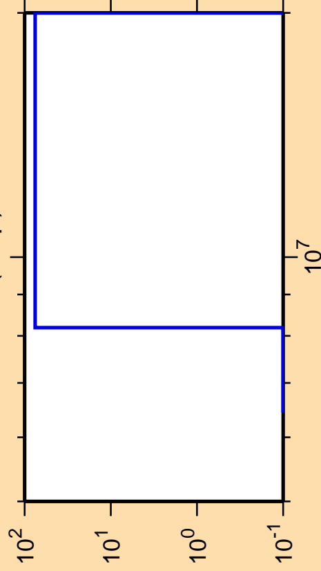
\Delta\sigma/\sigma vs. E for ^{222}\text{Fr}(n,np)
