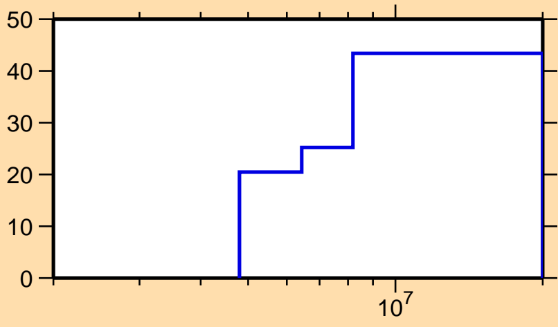
\Delta\sigma/\sigma vs. E for ^{222}\text{Fr}(n,2n)
