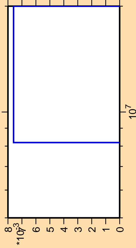
\Delta\sigma/\sigma vs. E for ^{222}\text{Fr}(\text{mt } 42)
