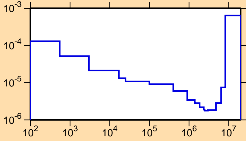
\sigma vs. E for ^{222}\text{Fr}(n,\alpha)
