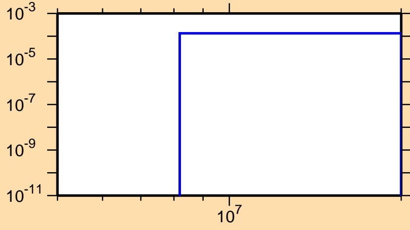
\sigma vs. E for ^{222}\text{Fr}(n,np)
