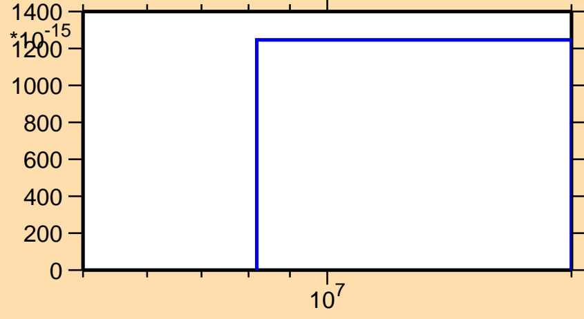
\sigma vs. E for ^{222}\text{Fr}(n,\text{He3})
