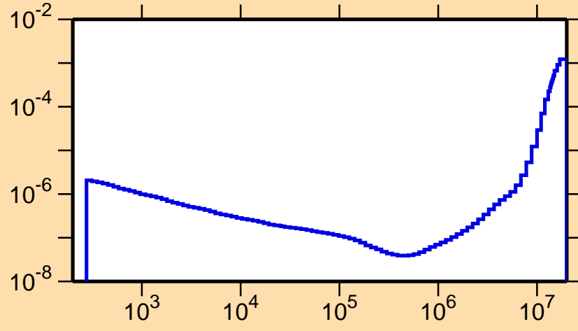
\sigma vs. E for ^{223}\text{Fr}(n,\alpha)
