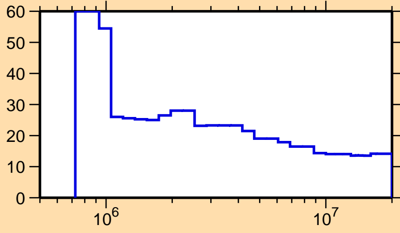
\Delta\sigma/\sigma vs. E for ^{223}\text{Fr}(n,n\text{onel.})
