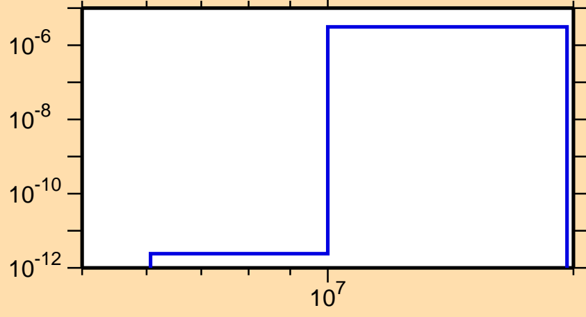
\sigma vs. E for ^{223}\text{Fr}(\text{mt117})
