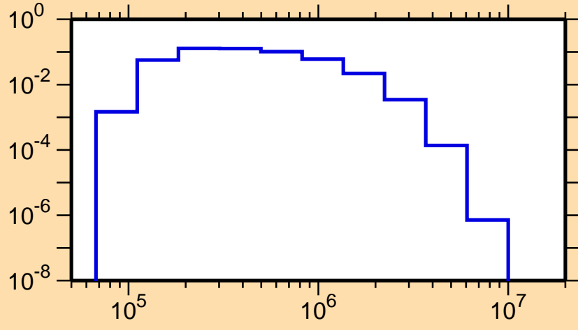
\sigma vs. E for ^{223}\text{Fr}(n,n_4)
