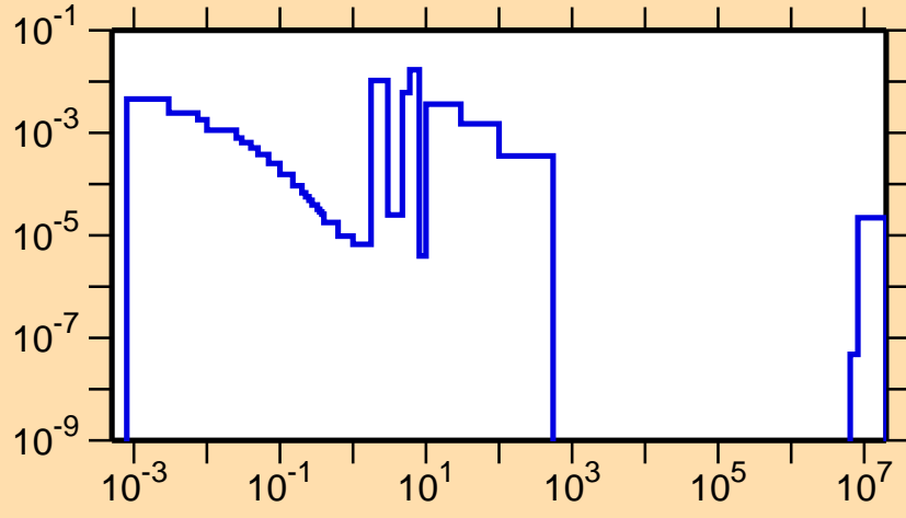
\sigma vs. E for ^{223}\text{Fr}(n,f)
