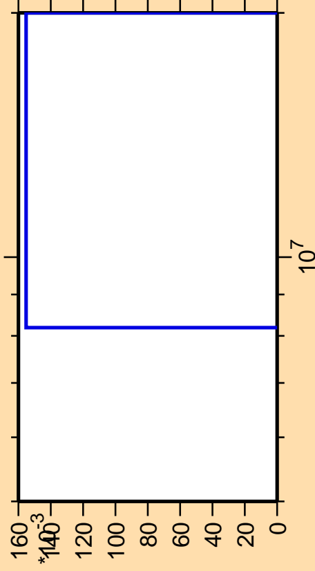
\Delta\sigma/\sigma vs. E for ^{223}\text{Fr}(n,\text{He3})
