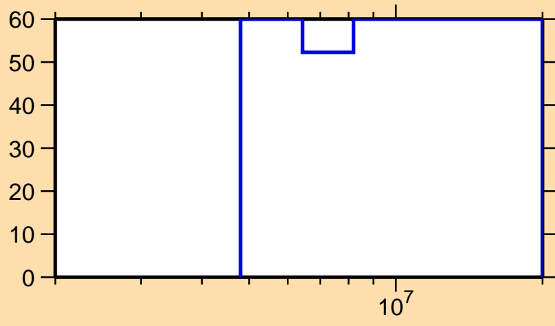
\Delta\sigma/\sigma vs. E for ^{223}\text{Fr}(n,2n)
