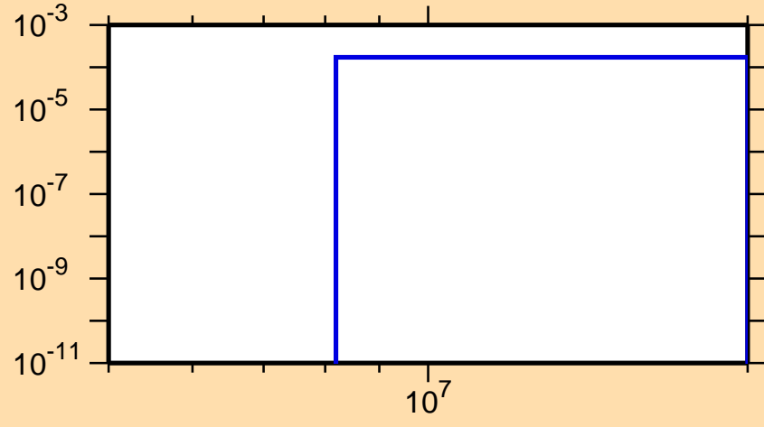
\sigma vs. E for ^{223}\text{Fr}(n,d)
