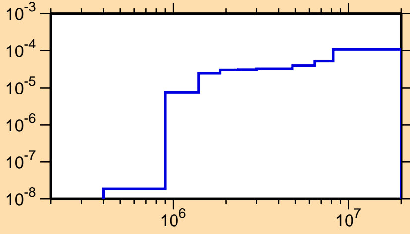
\sigma vs. E for ^{223}\text{Fr}(n,n\alpha)
