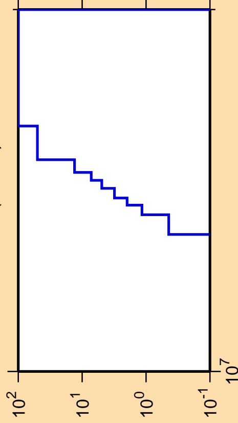
\Delta\sigma/\sigma vs. E for ^{224}\text{Fr}(\text{mt } 45)
