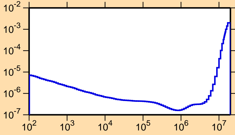
\sigma vs. E for ^{224}\text{Fr}(n,\alpha)
