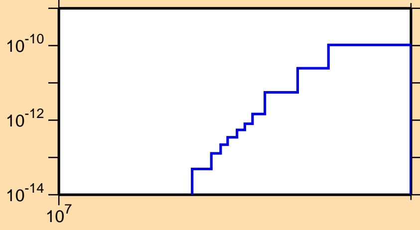
\sigma vs. E for ^{224}\text{Fr}(\text{mt } 45)
