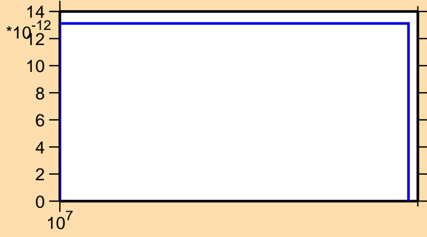
\sigma vs. E for ^{224}\text{Fr}(\text{mt117})
