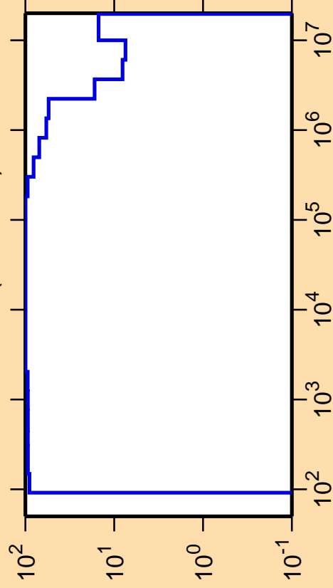
\Delta\sigma/\sigma vs. E for ^{224}\text{Fr}(n,\text{nonel.})
