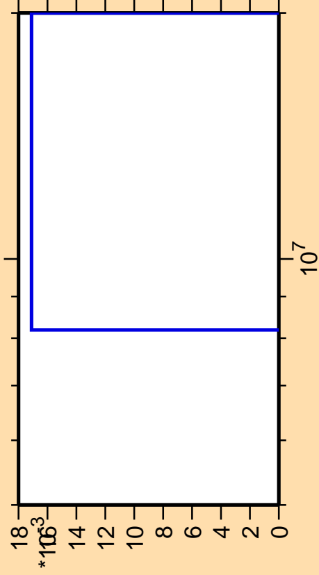
\Delta\sigma/\sigma vs. E for ^{224}\text{Fr} (mt 42)
