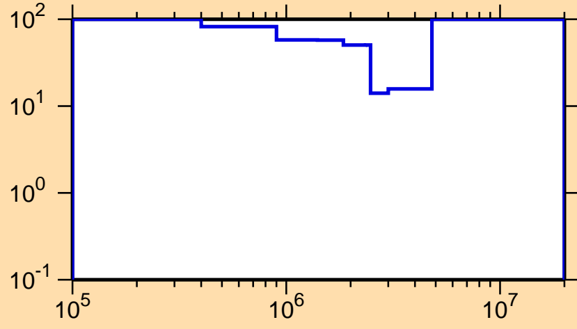
\Delta\sigma/\sigma vs. E for ^{224}\text{Fr}(n, n\text{cont.})
