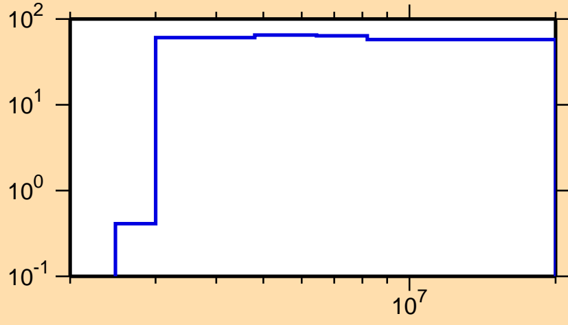
\Delta\sigma/\sigma vs. E for ^{224}\text{Fr}(n,p)
