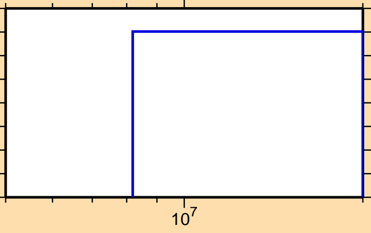
\sigma vs. E for ^{224}\text{Fr}(n,nt)
