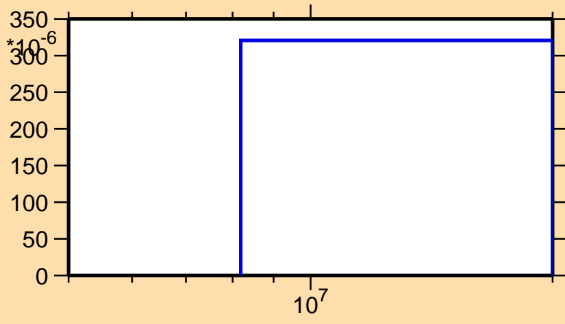
\sigma vs. E for ^{224}\text{Fr}(n,3n\alpha)
