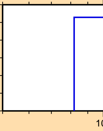
\sigma vs. E for ^{224}\text{Fr}(\text{mt117})
