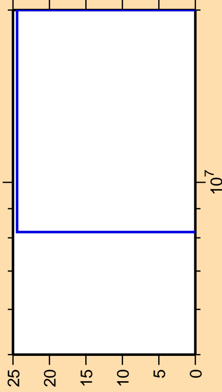
\Delta\sigma/\sigma vs. E for ^{224}\text{Fr} (mt 45)
