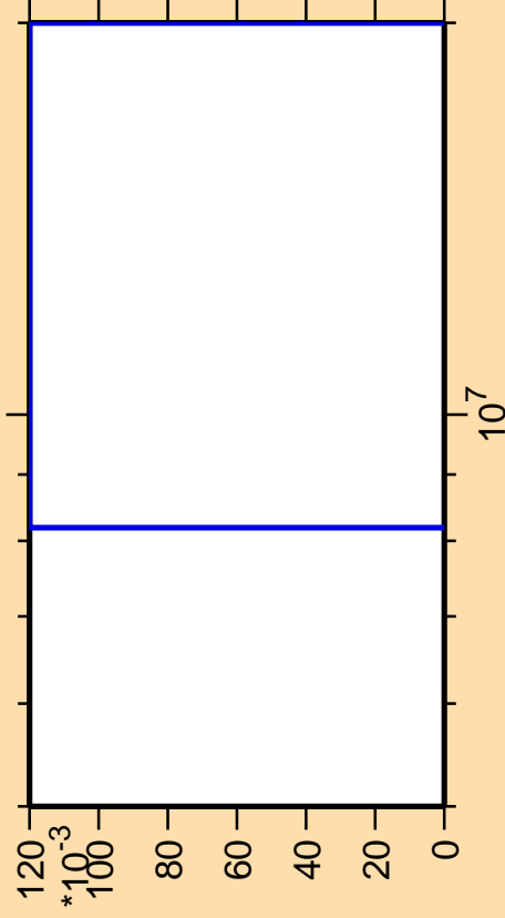
\Delta\sigma/\sigma vs. E for ^{224}\text{Fr}(\text{mt } 11)
