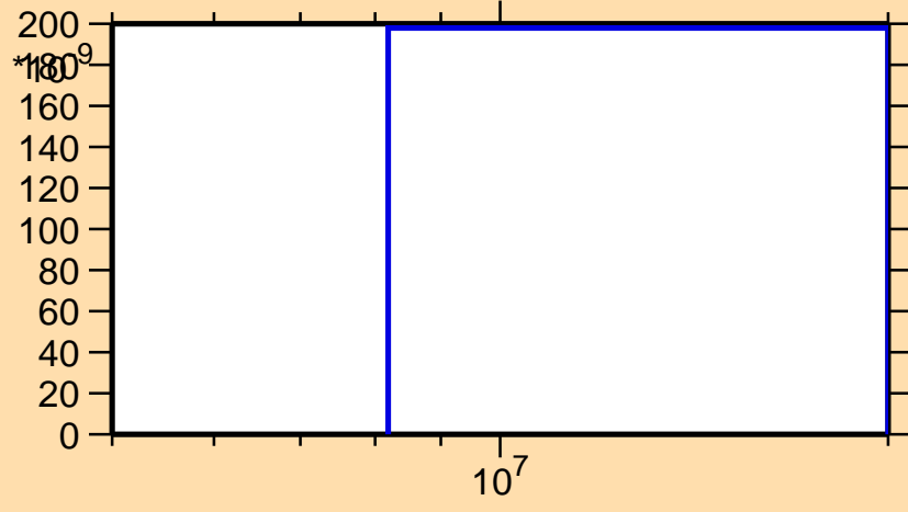
\sigma vs. E for ^{224}\text{Fr}(n,2np)
