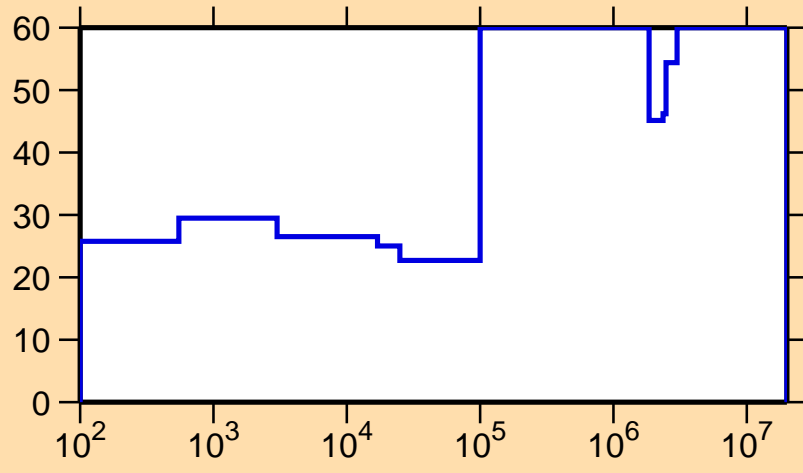
\Delta\sigma/\sigma vs. E for ^{224}\text{Fr}(n,\text{el.})
