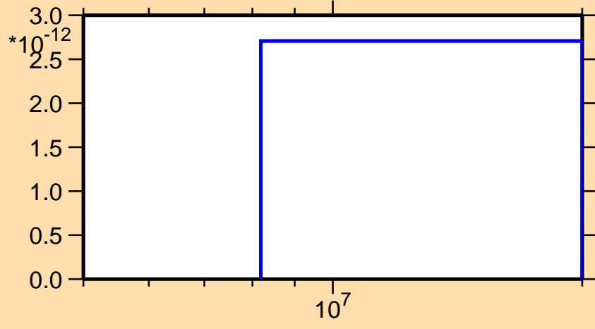
\sigma vs. E for ^{224}\text{Fr} (mt 45)
