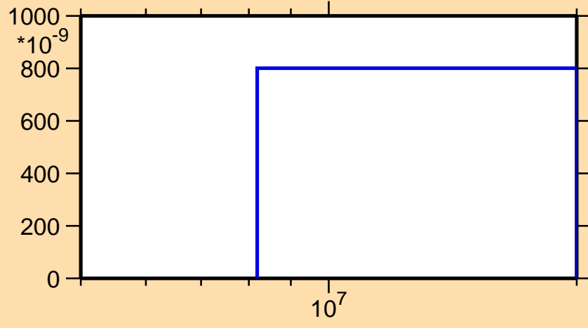
\sigma vs. E for ^{224}\text{Fr}(n,\text{nd})
