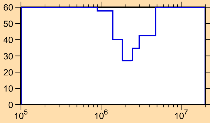
\Delta\sigma/\sigma vs. E for ^{224}\text{Fr}(n,\text{tot.})
