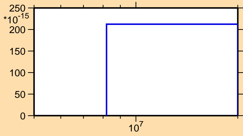
\sigma vs. E for ^{224}\text{Fr}(\text{mt } 11)
