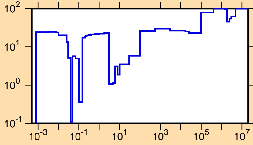
\Delta\sigma/\sigma vs. E for ^{224}\text{Fr}(n,el.)
