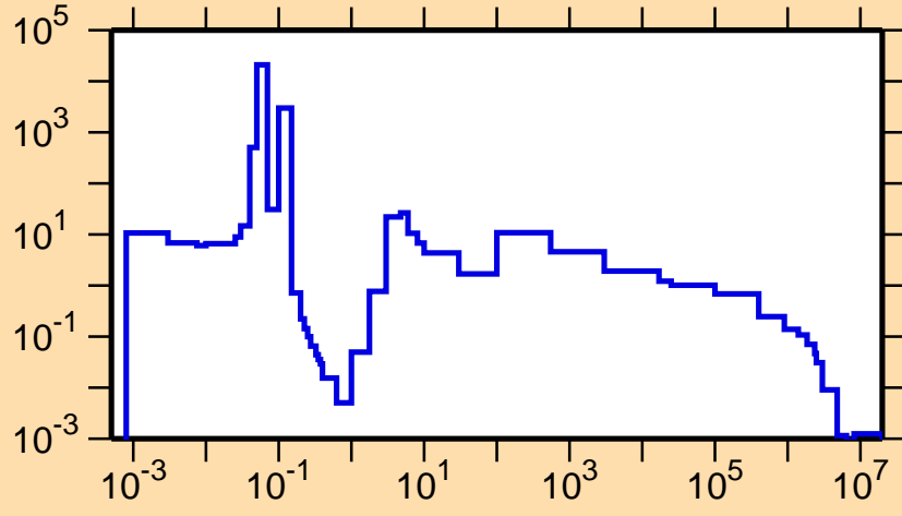
\sigma vs. E for ^{224}\text{Fr}(n,\gamma)
