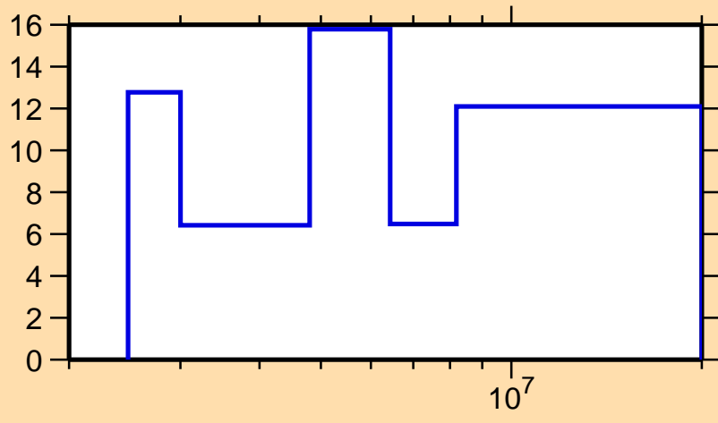
\Delta\sigma/\sigma vs. E for ^{224}\text{Fr}(n,\text{nonel.})
