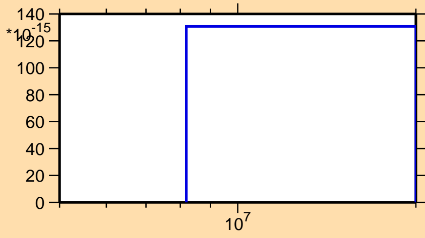
\sigma vs. E for ^{224}\text{Fr}(n,\text{He3})
