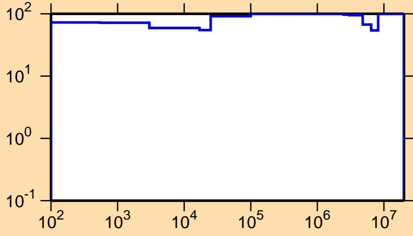
\Delta\sigma/\sigma vs. E for ^{224}\text{Fr}(n,\gamma)
