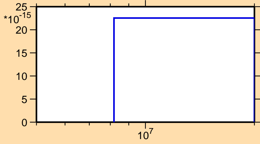
\sigma vs. E for ^{224}\text{Fr} (mt 42)
