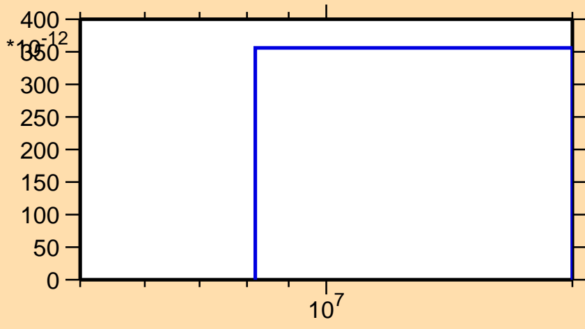
\sigma vs. E for ^{224}\text{Fr}(n,p\alpha)
