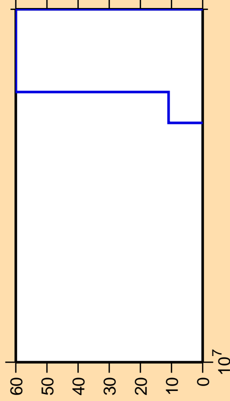
\Delta\sigma/\sigma vs. E for ^{225}\text{Fr} (mt 45)
