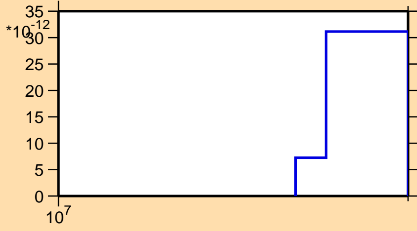
\sigma vs. E for ^{225}\text{Fr}(\text{mt117})
