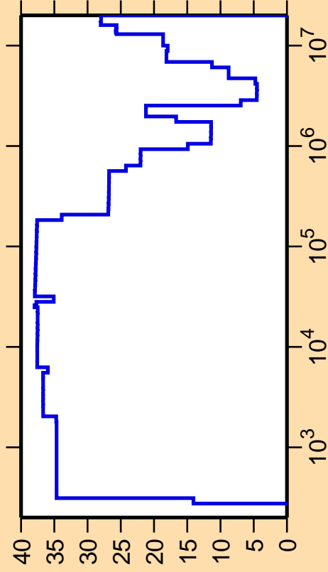
\Delta\sigma/\sigma vs. E for ^{225}\text{Fr}(n,\text{nonel.})
