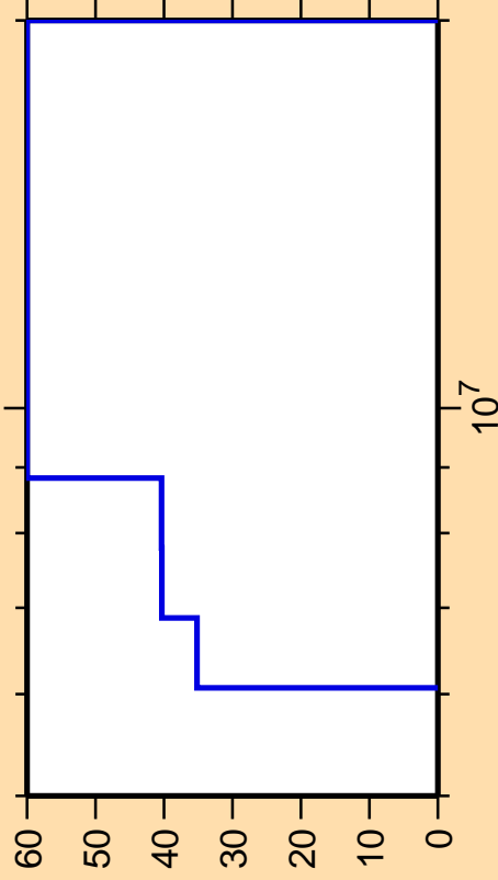
\Delta\sigma/\sigma vs. E for ^{225}\text{Fr}(n,n\text{cont.})
