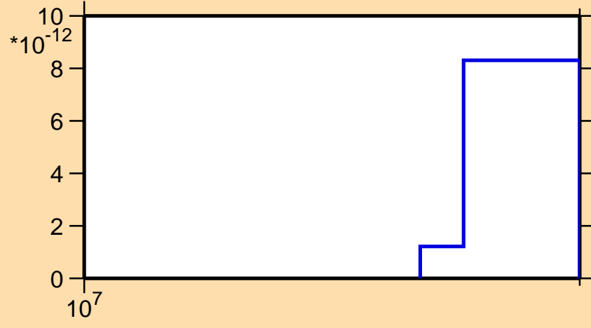
\sigma vs. E for ^{225}\text{Fr} (mt 45)
