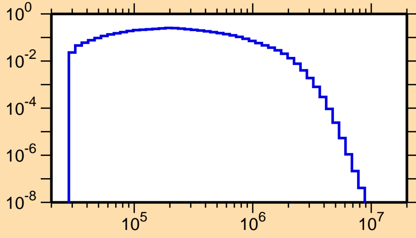
\sigma vs. E for ^{225}\text{Fr}(n,n_1)
