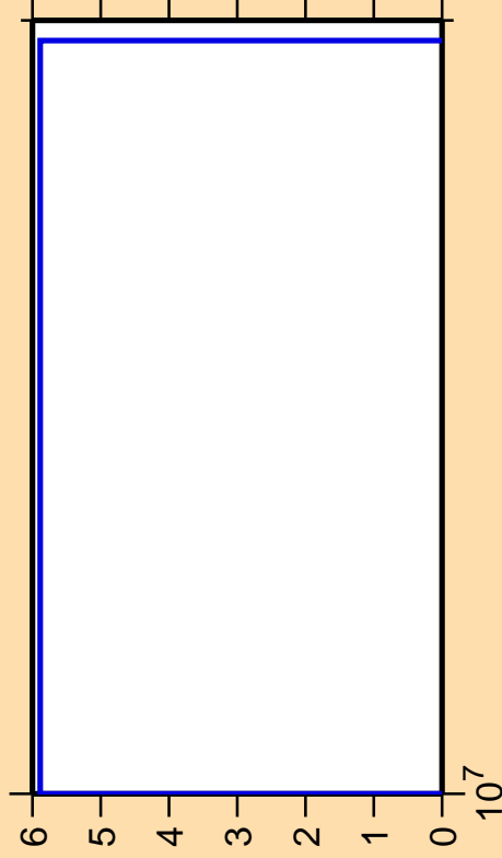
\Delta\sigma/\sigma vs. E for ^{225}\text{Fr}(\text{mt117})
