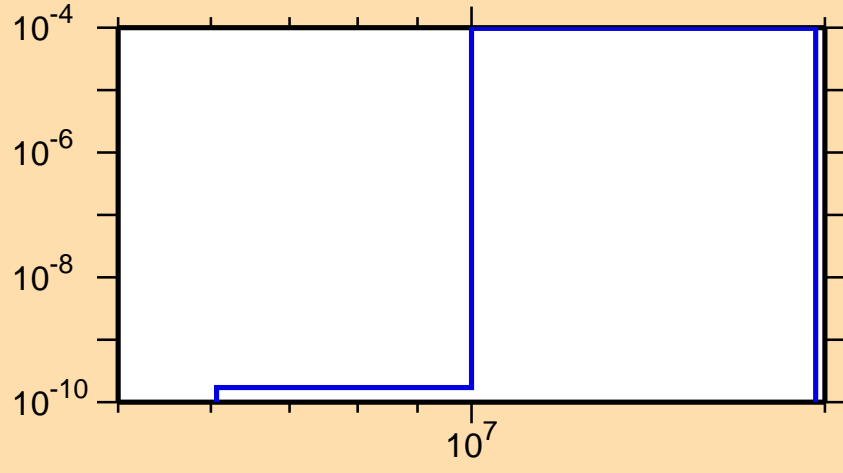
\sigma vs. E for ^{225}\text{Fr}(n,d)
