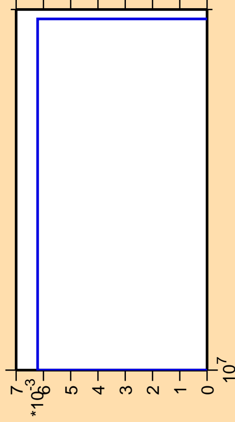
\Delta\sigma/\sigma vs. E for ^{225}\text{Fr} (mt 42)
