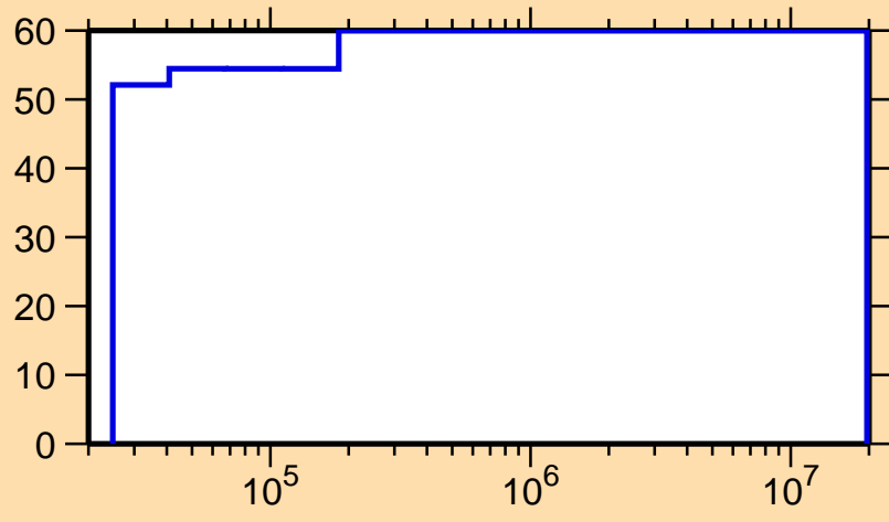
\Delta\sigma/\sigma vs. E for ^{225}\text{Fr}(n,n_1)
