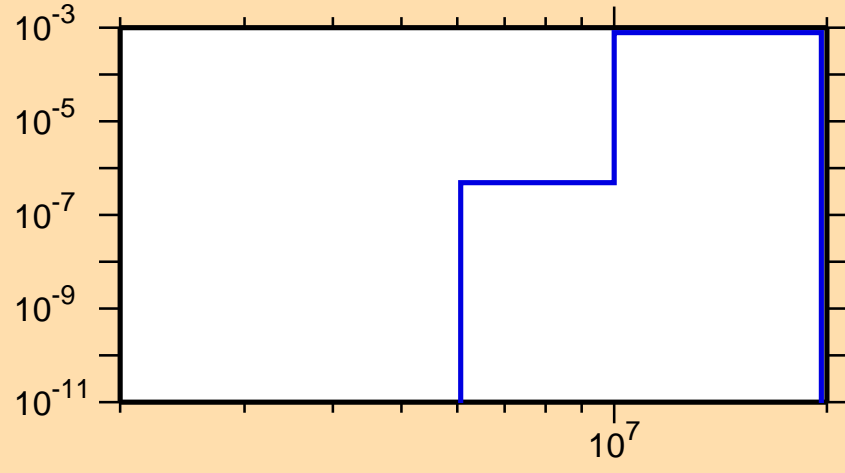
\sigma vs. E for ^{225}\text{Fr}(n,p)
