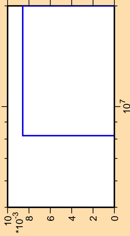
\Delta\sigma/\sigma vs. E for ^{225}\text{Fr}(\text{mt } 42)
