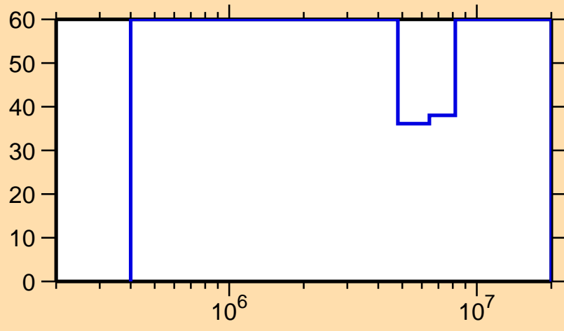
\Delta\sigma/\sigma vs. E for ^{225}\text{Fr}(n,n\text{cont.})
