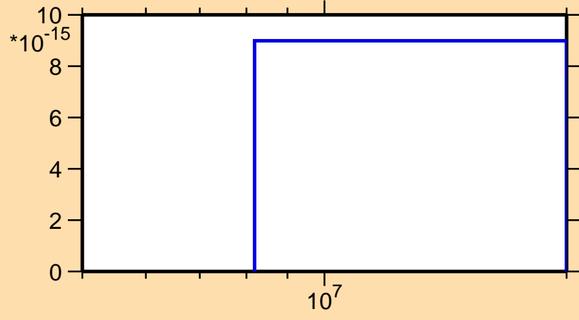
\sigma vs. E for ^{225}\text{Fr}(\text{mt } 42)
