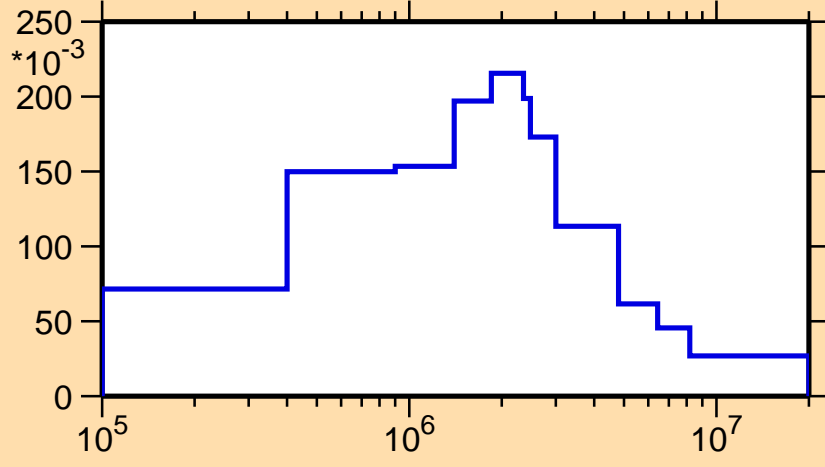
\sigma vs. E for ^{225}\text{Fr}(n,n_4)
