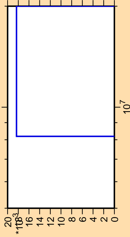
\Delta\sigma/\sigma vs. E for ^{225}\text{Fr}(n,\text{He3})
