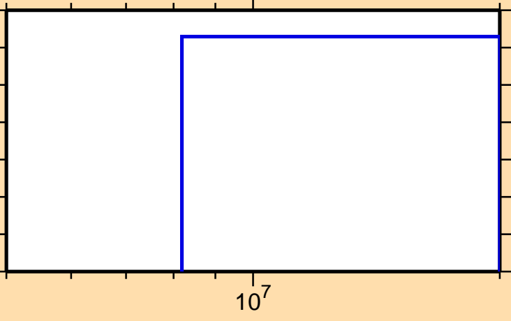
\sigma vs. E for ^{225}\text{Fr}(n,3n\alpha)
