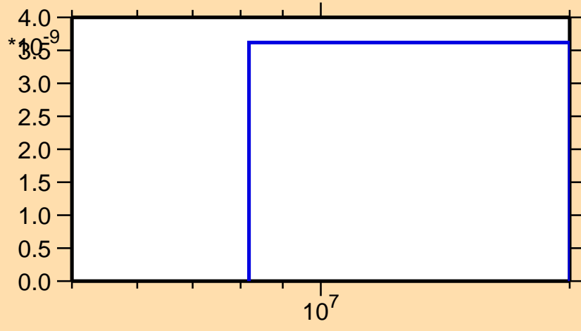
\sigma vs. E for ^{225}\text{Fr}(n,2np)
