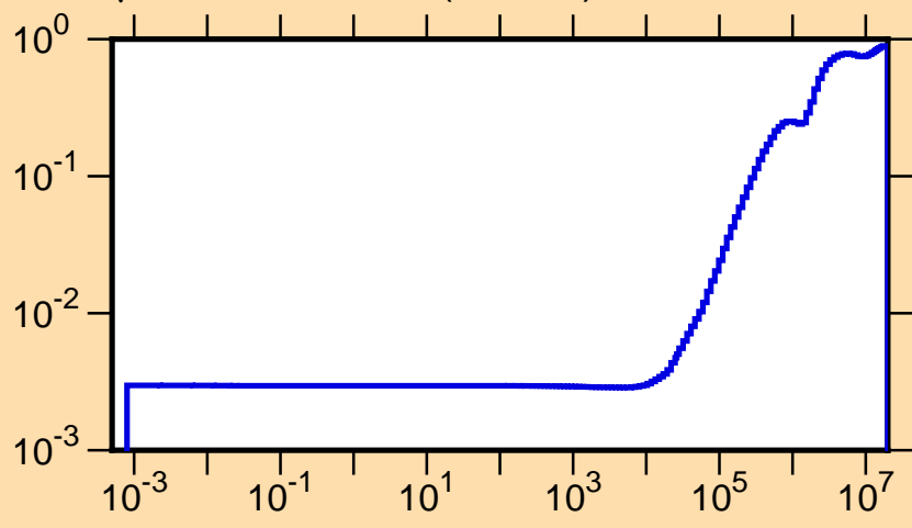
\mu vs. E for ^{226}\text{Fr}(\text{mt251})
