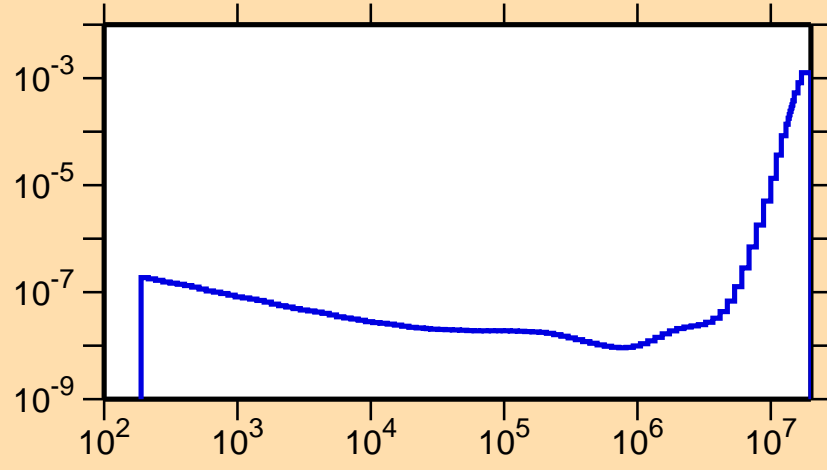
\sigma vs. E for ^{226}\text{Fr}(n,\alpha)
