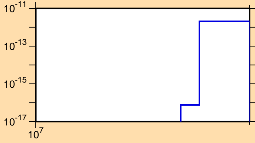
\sigma vs. E for ^{226}\text{Fr}(\text{mt } 42)
