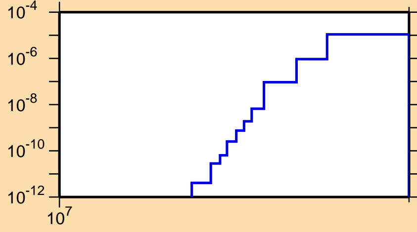
\sigma vs. E for ^{226}\text{Fr}(n,2np)
