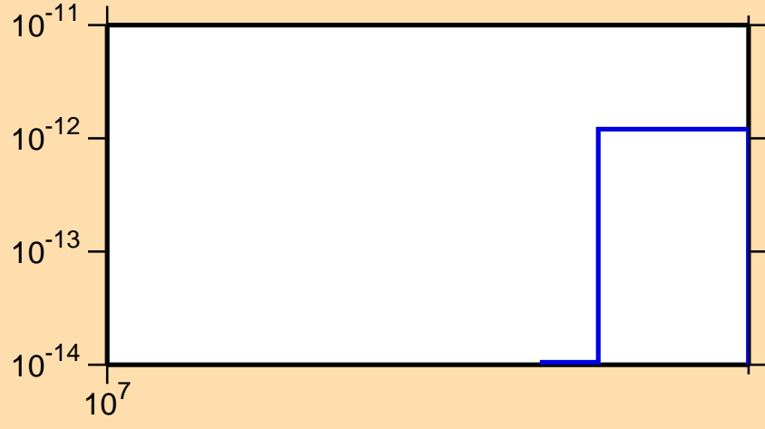
\sigma vs. E for ^{226}\text{Fr}(n,\text{He}3)
