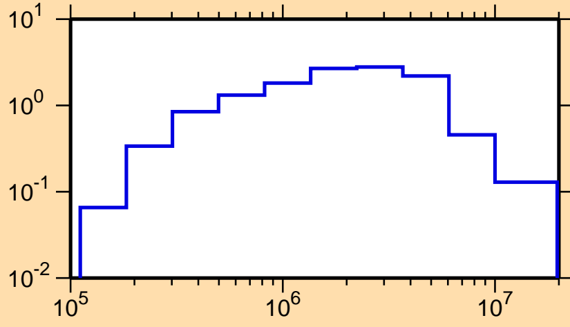
\sigma vs. E for ^{226}\text{Fr}(n,n\text{cont.})
