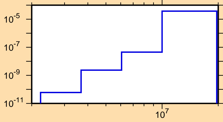
\sigma vs. E for ^{226}\text{Fr}(n,n\alpha)
