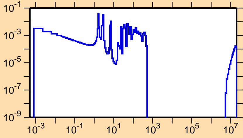
\sigma vs. E for ^{227}\text{Fr}(n,f)
