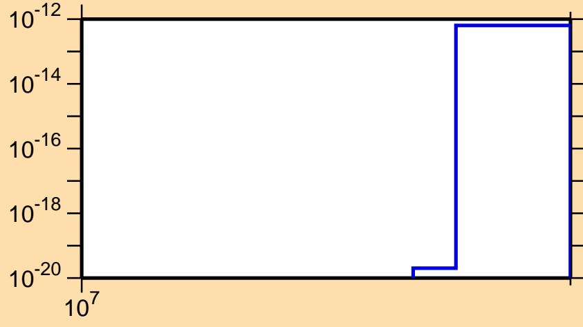
\sigma vs. E for ^{227}\text{Fr} (mt 42)
