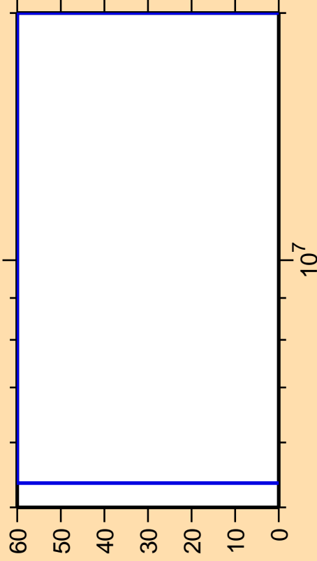
\Delta\sigma/\sigma vs. E for ^{227}\text{Fr}(n,2n)
