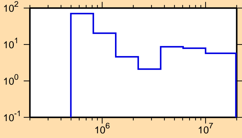
\Delta\sigma/\sigma vs. E for ^{227}\text{Fr}(n,\text{nonel.})
