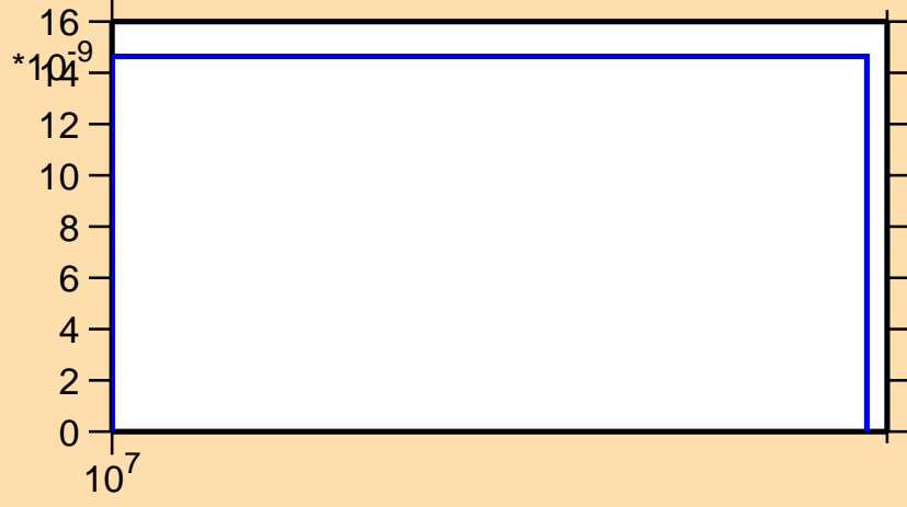
\sigma vs. E for ^{227}\text{Fr}(n,\text{nd})
