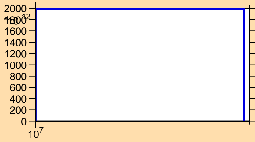
\sigma vs. E for ^{227}\text{Fr}(n,2np)
