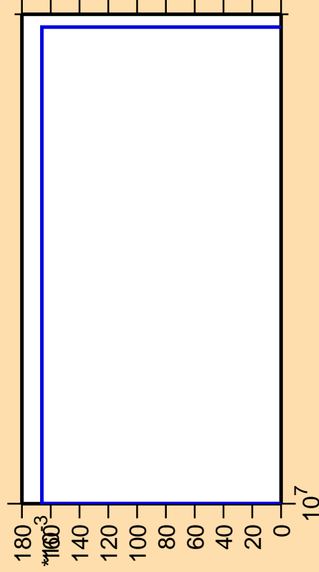
\Delta\sigma/\sigma vs. E for ^{227}\text{Fr}(\text{mt } 11)
