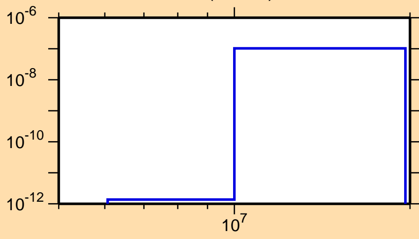
\sigma vs. E for ^{227}\text{Fr}(n,2n\alpha)
