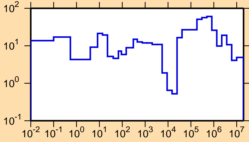
\Delta\sigma/\sigma vs. E for ^{227}\text{Fr}(n,\text{tot.})
