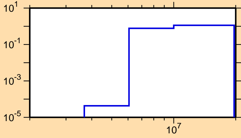
\sigma vs. E for ^{227}\text{Fr}(n,2n)
