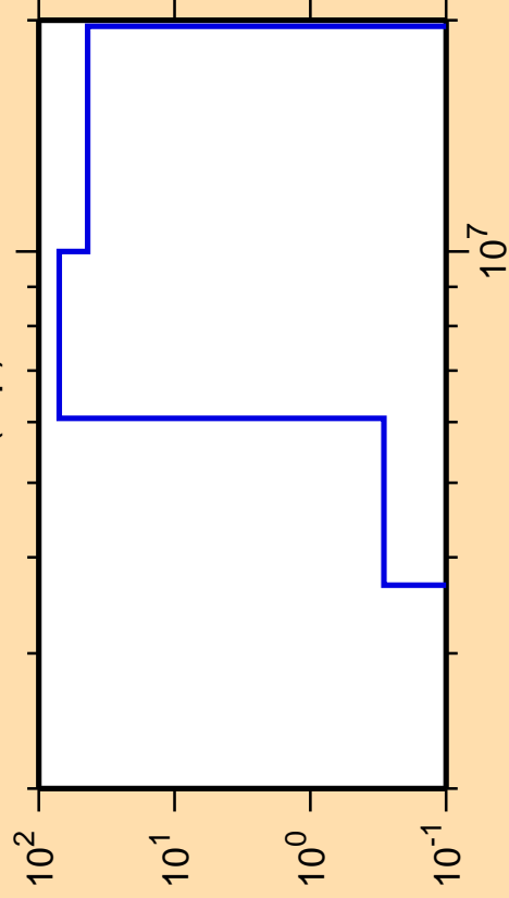
\Delta\sigma/\sigma vs. E for ^{227}\text{Fr}(n,p)
