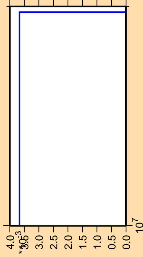
\Delta\sigma/\sigma vs. E for ^{227}\text{Fr}(\text{mt } 42)
