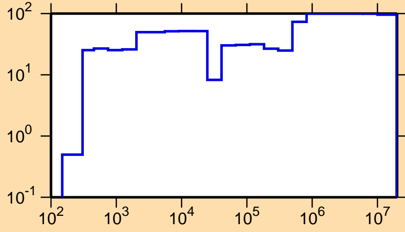
\Delta\sigma/\sigma vs. E for ^{227}\text{Fr}(n,\gamma)
