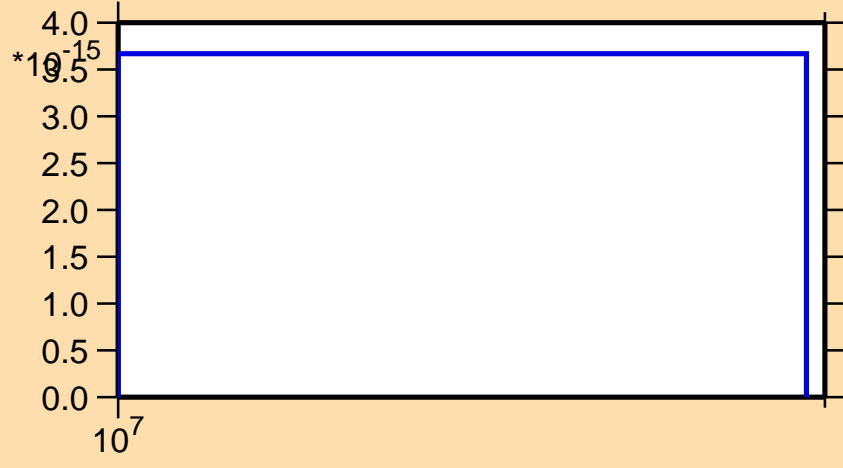
\sigma vs. E for ^{227}\text{Fr}(\text{mt } 42)
