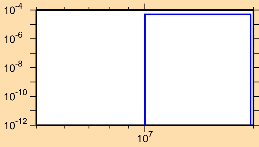
\sigma vs. E for ^{227}\text{Fr}(n,np)
