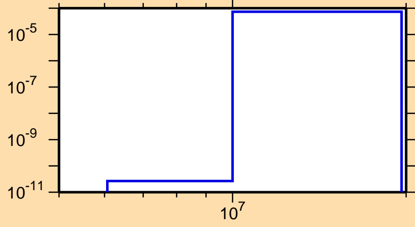
\sigma vs. E for ^{227}\text{Fr}(n,d)
