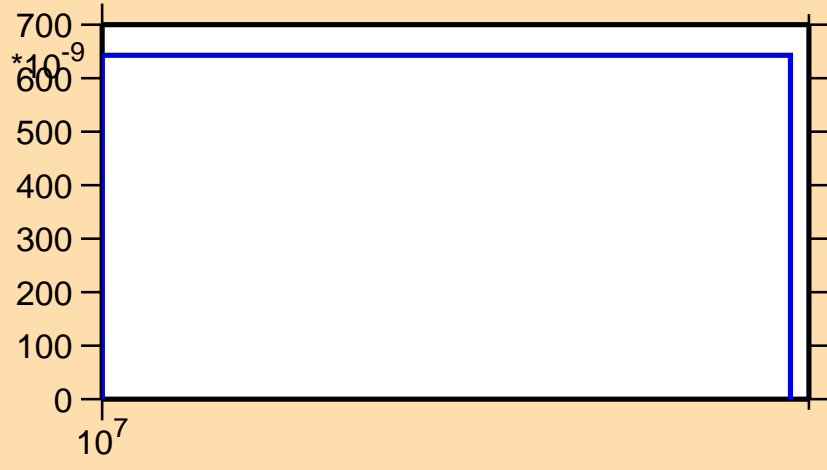
\sigma vs. E for ^{227}\text{Fr}(n,nt)
