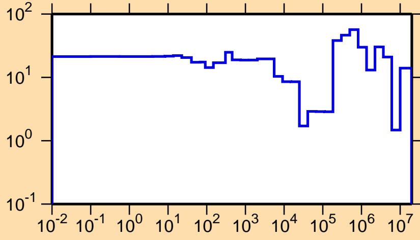
\Delta\sigma/\sigma vs. E for ^{227}\text{Fr}(n,el.)
