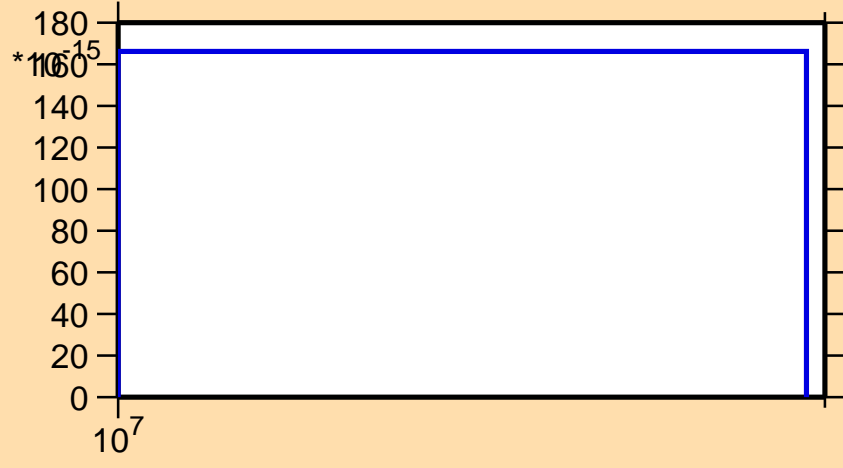
\sigma vs. E for ^{227}\text{Fr}(\text{mt } 11)
