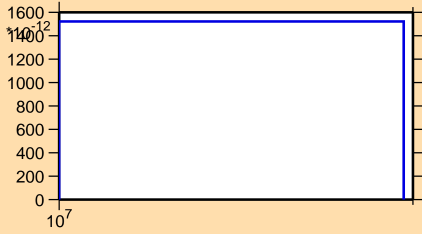
\sigma vs. E for ^{227}\text{Fr}(n,3n\alpha)
