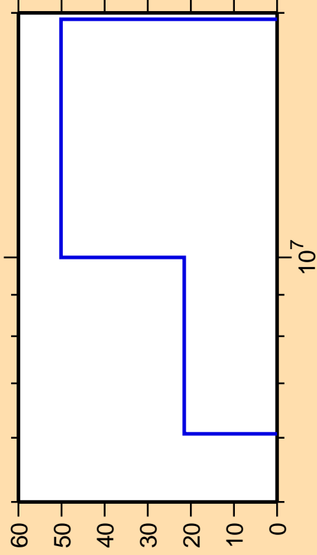
\Delta\sigma/\sigma vs. E for ^{227}\text{Fr}(n,d)
