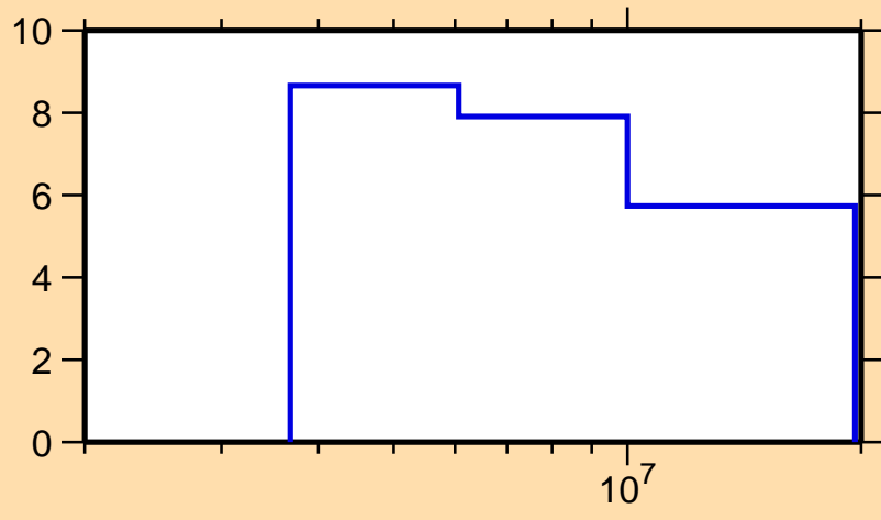
\Delta\sigma/\sigma vs. E for ^{227}\text{Fr}(n,\text{nonel.})
