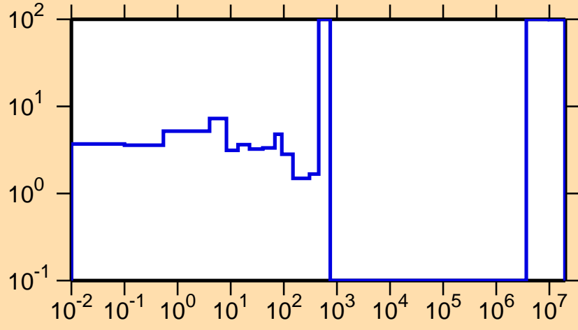
\Delta\sigma/\sigma vs. E for ^{227}\text{Fr}(n,f)
