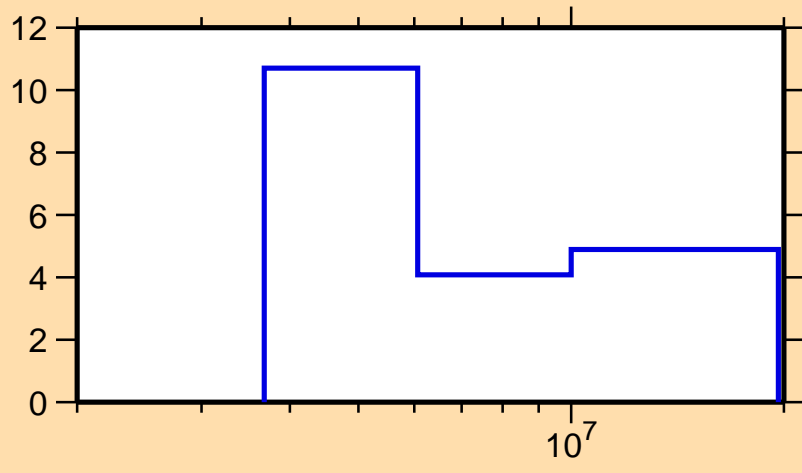
\Delta\sigma/\sigma vs. E for ^{227}\text{Fr}(n,\text{tot.})
