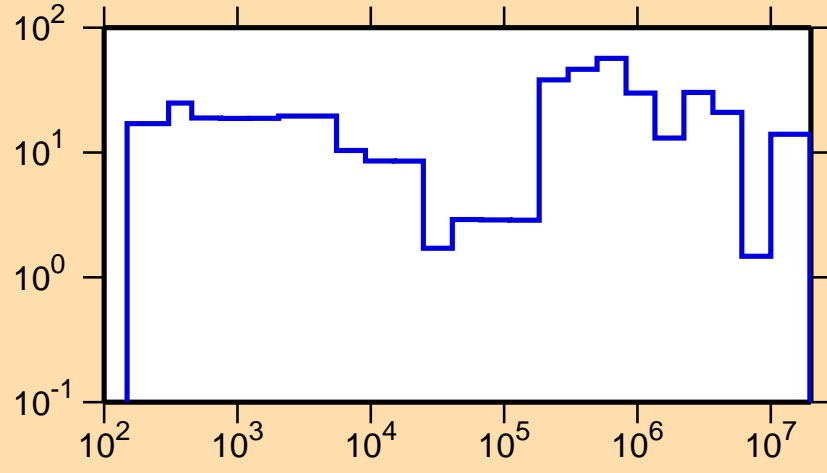
\Delta\sigma/\sigma vs. E for ^{227}\text{Fr}(n,\text{el.})
