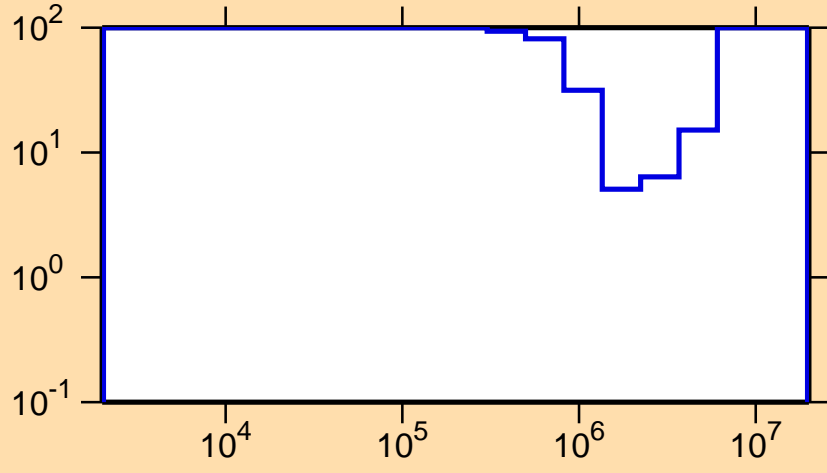
\Delta\sigma/\sigma vs. E for ^{227}\text{Fr}(n,\text{inel.})
