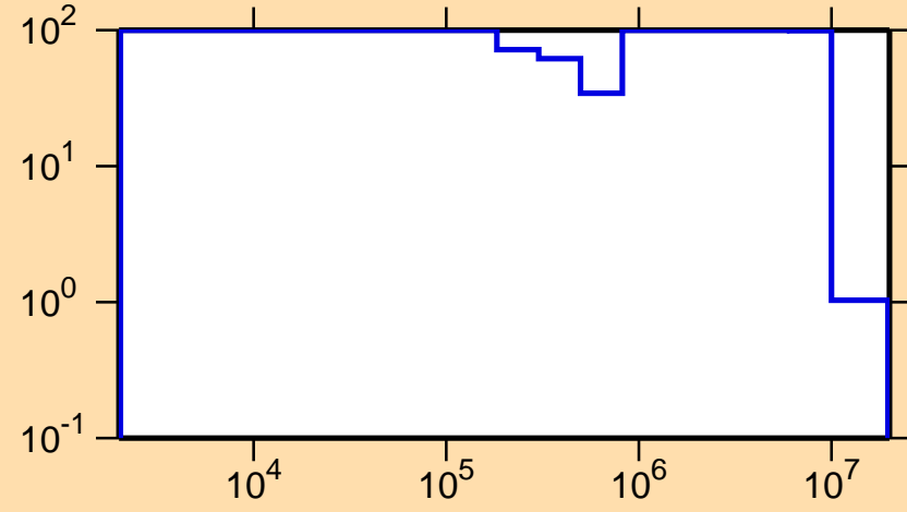
\Delta\sigma/\sigma vs. E for ^{227}\text{Fr}(n,n_1)
