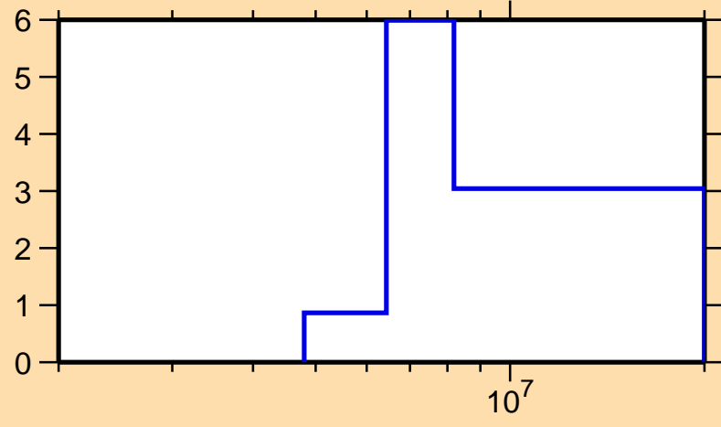
\Delta\sigma/\sigma vs. E for ^{227}\text{Fr}(n,\text{tot.})
