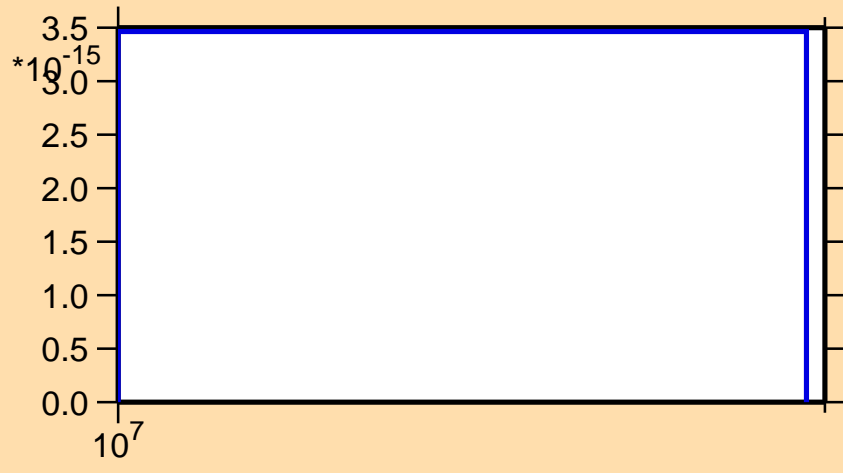
\sigma vs. E for ^{228}\text{Fr}(\text{mt } 42)
