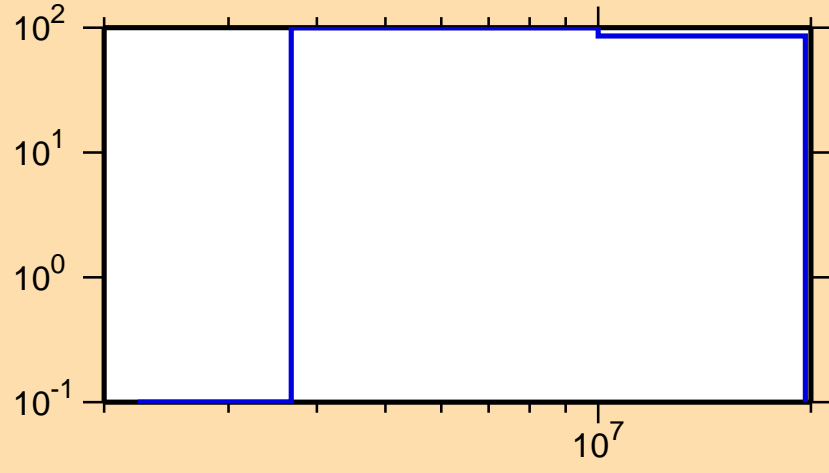
\Delta\sigma/\sigma vs. E for ^{228}\text{Fr}(n,p)
