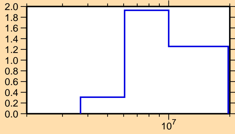
\sigma vs. E for ^{228}\text{Fr}(n,2n)
