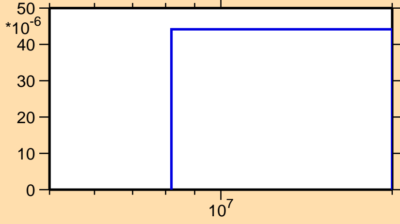
\sigma vs. E for ^{228}\text{Fr}(n,d)
