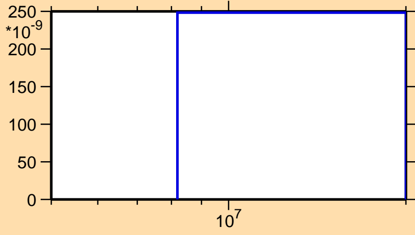
\sigma vs. E for ^{228}\text{Fr}(n,\text{nd})
