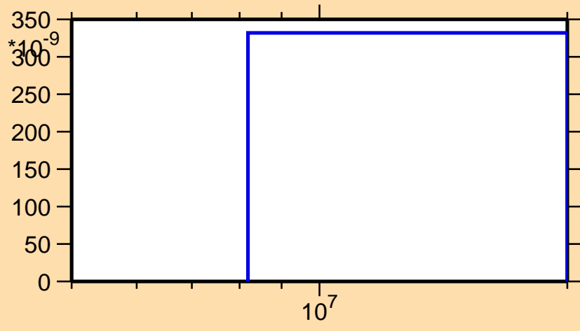
\sigma vs. E for ^{228}\text{Fr}(n,nt)
