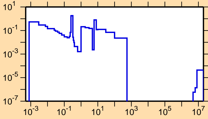
\sigma vs. E for ^{228}\text{Fr}(n,f)
