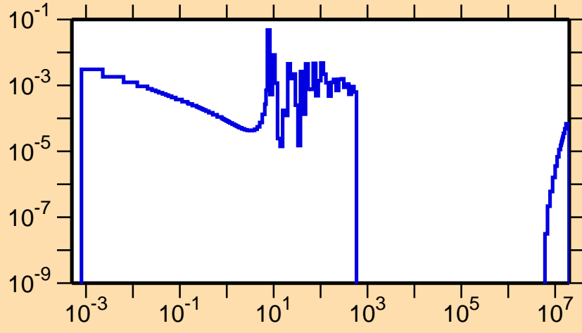
\sigma vs. E for ^{229}\text{Fr}(n,f)
