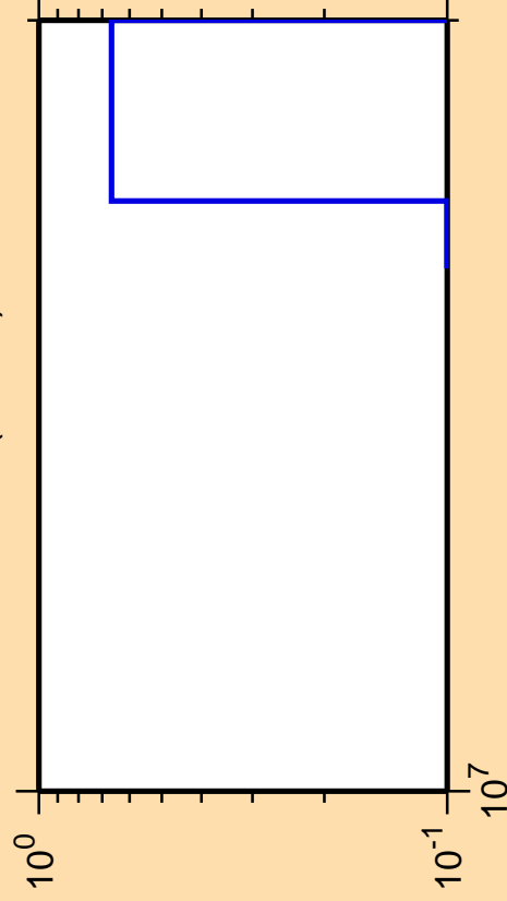
\Delta\sigma/\sigma vs. E for ^{229}\text{Fr} (mt 42)
