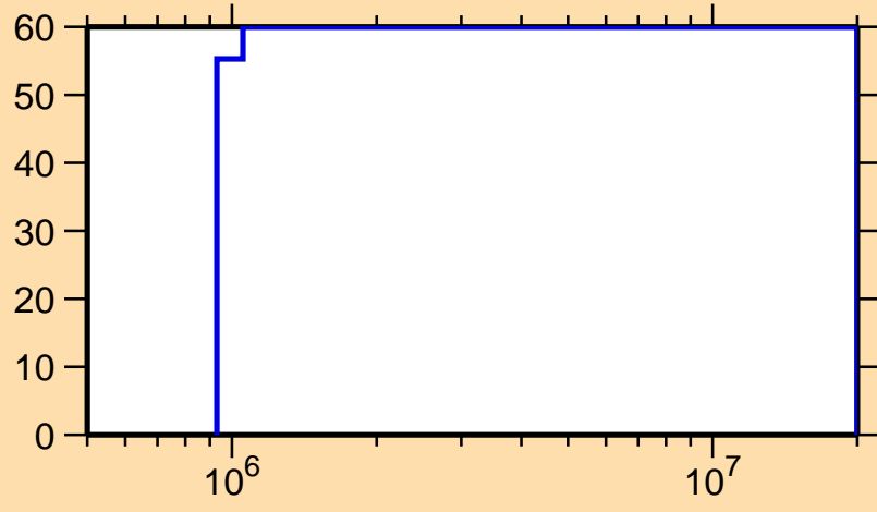
\Delta\sigma/\sigma vs. E for ^{229}\text{Fr}(n, ncont.)
