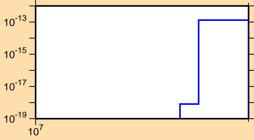
\sigma vs. E for ^{229}\text{Fr} (mt 42)
