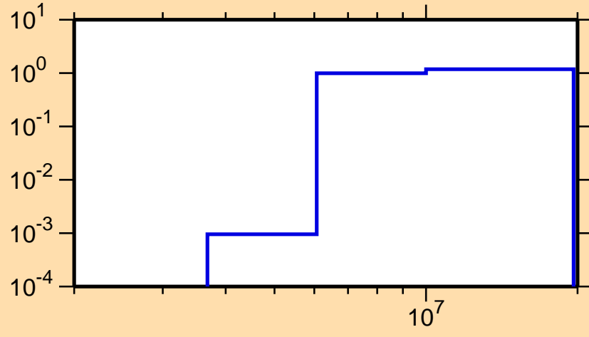
\sigma vs. E for ^{229}\text{Fr}(n,2n)
