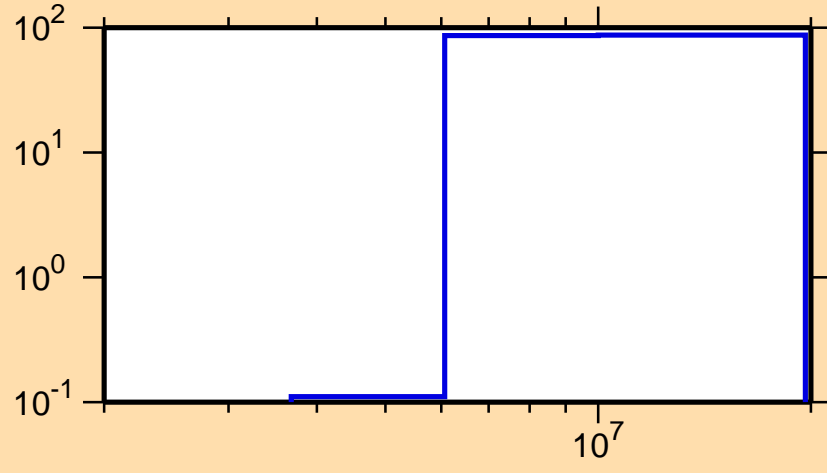
\Delta\sigma/\sigma vs. E for ^{229}\text{Fr}(n,p)
