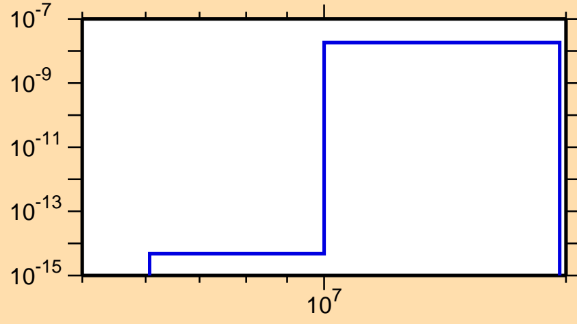
\sigma vs. E for ^{229}\text{Fr}(n,2n\alpha)
