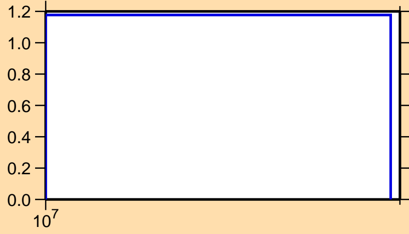
\sigma vs. E for ^{229}\text{Fr}(n,3n)
