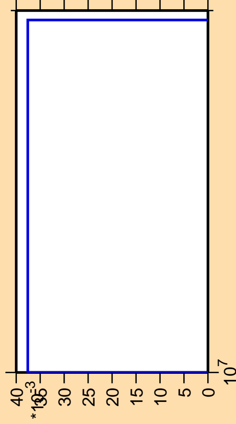
\Delta\sigma/\sigma vs. E for ^{229}\text{Fr} (mt 11)
