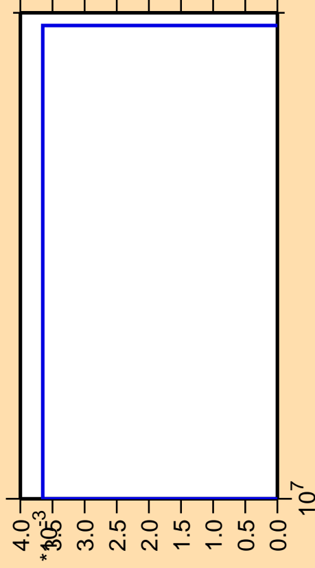
\Delta\sigma/\sigma vs. E for ^{229}\text{Fr}(\text{mt } 42)
