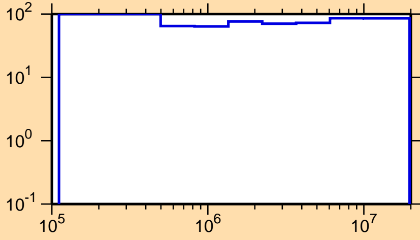
\Delta\sigma/\sigma vs. E for ^{229}\text{Fr}(n,n\text{cont.})
