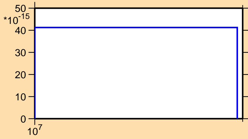
\sigma vs. E for ^{229}\text{Fr} (mt 11)
