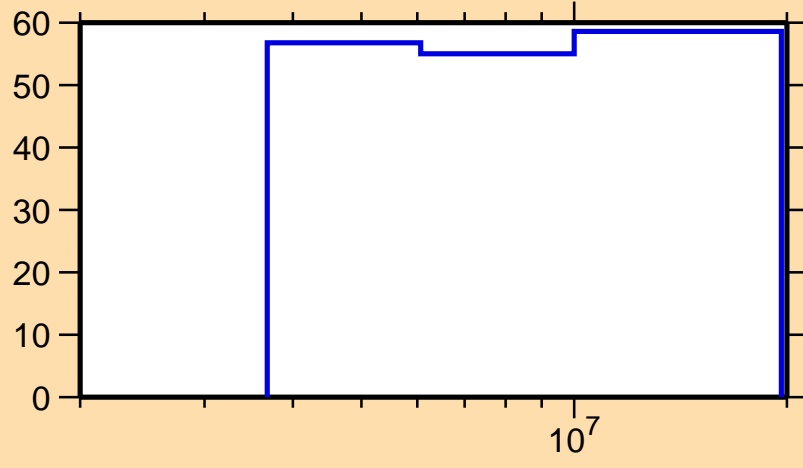
\Delta\sigma/\sigma vs. E for ^{229}\text{Fr}(n,\text{nonel.})
