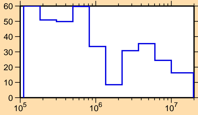
\Delta\sigma/\sigma vs. E for ^{229}\text{Fr}(n,\text{tot.})
