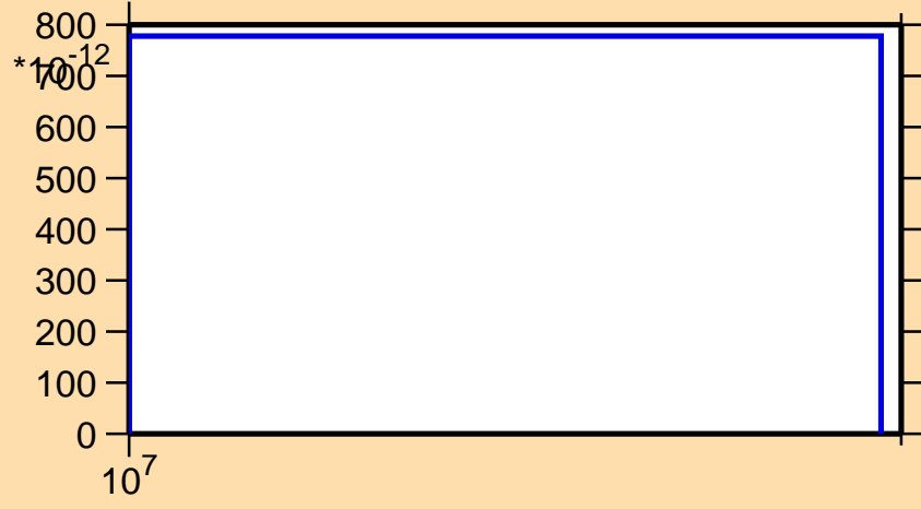
\sigma vs. E for ^{229}\text{Fr}(n,2np)
