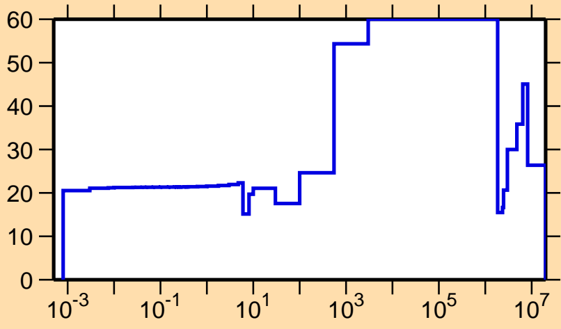
\Delta\sigma/\sigma vs. E for ^{229}\text{Fr}(n,el.)
