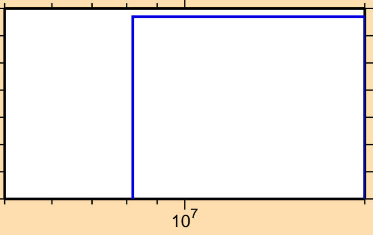
\sigma vs. E for ^{229}\text{Fr}(n,t)
