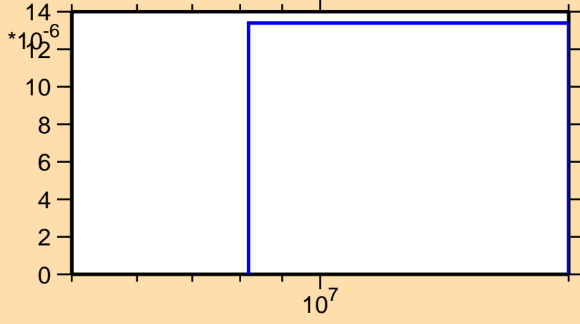
\sigma vs. E for ^{229}\text{Fr}(n,t)
