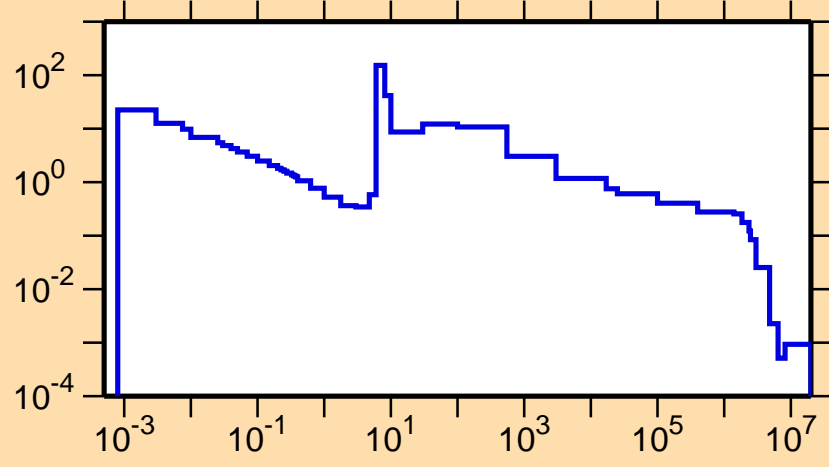
\sigma vs. E for ^{229}\text{Fr}(n,\gamma)
