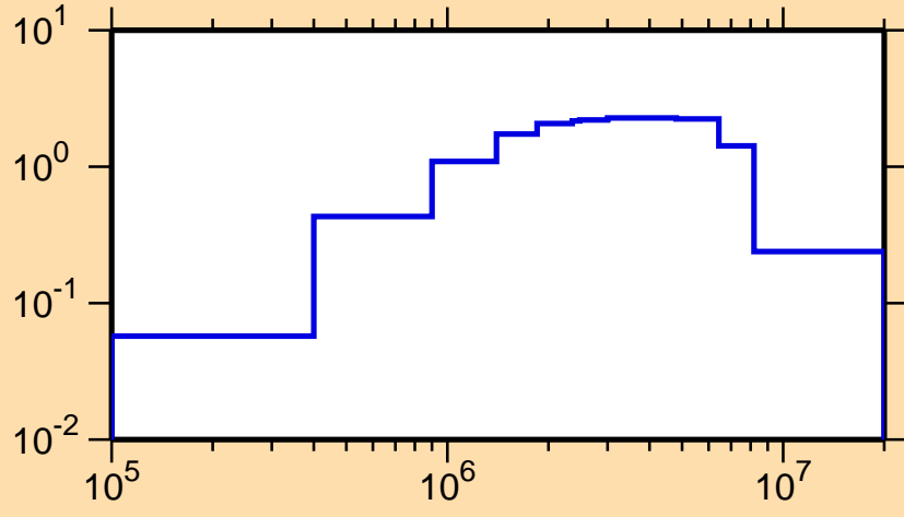
\sigma vs. E for ^{229}\text{Fr}(n,n\text{cont.})
