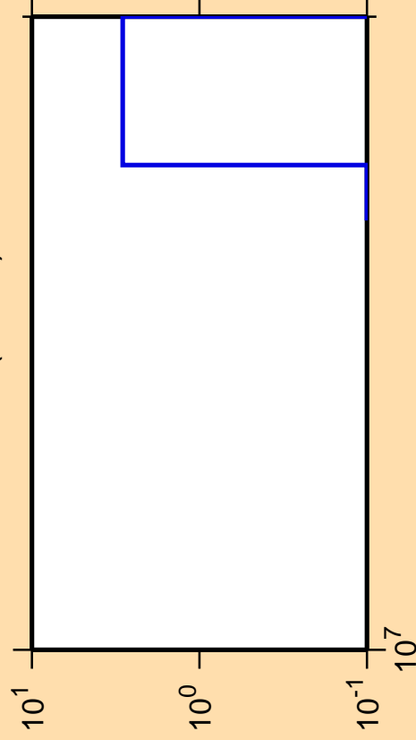
\Delta\sigma/\sigma vs. E for ^{230}\text{Fr} (mt 11)
