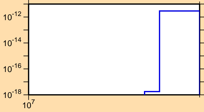
\sigma vs. E for ^{230}\text{Fr} (mt 11)
