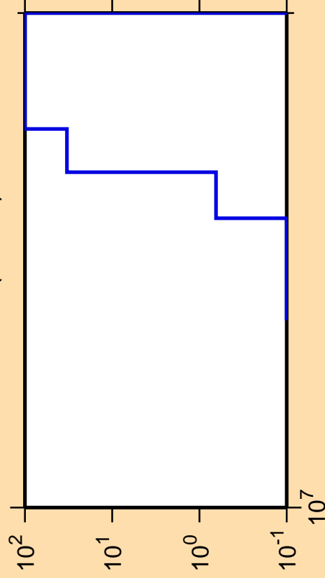
\Delta\sigma/\sigma vs. E for ^{230}\text{Fr}(n,3n\alpha)
