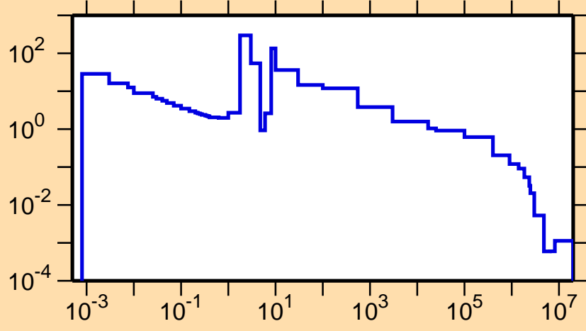
\sigma vs. E for ^{230}\text{Fr}(n,\gamma)
