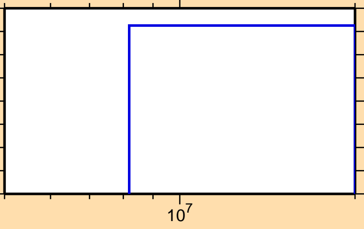
\sigma vs. E for ^{230}\text{Fr}(n,d)
