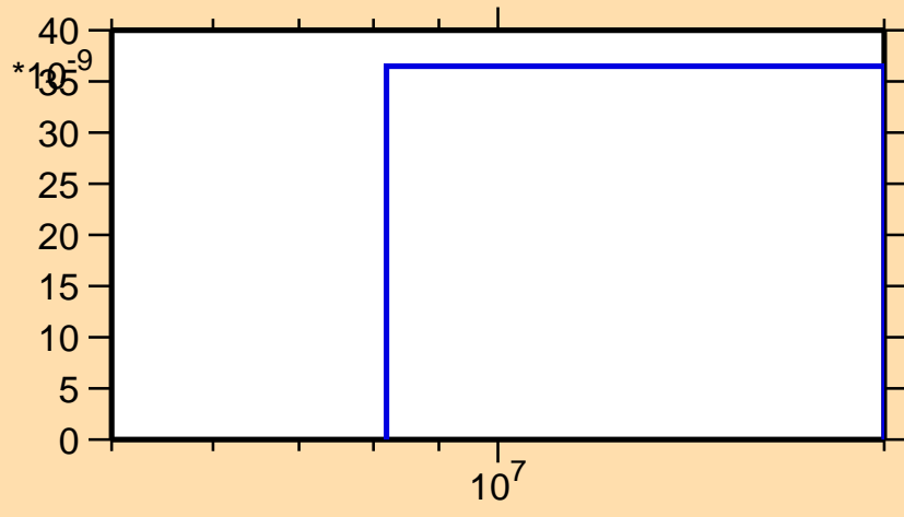
\sigma vs. E for ^{230}\text{Fr}(n,2n\alpha)
