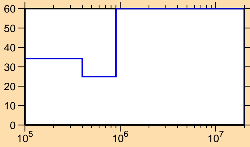
\Delta\sigma/\sigma vs. E for ^{230}\text{Fr}(n,\text{el.})
