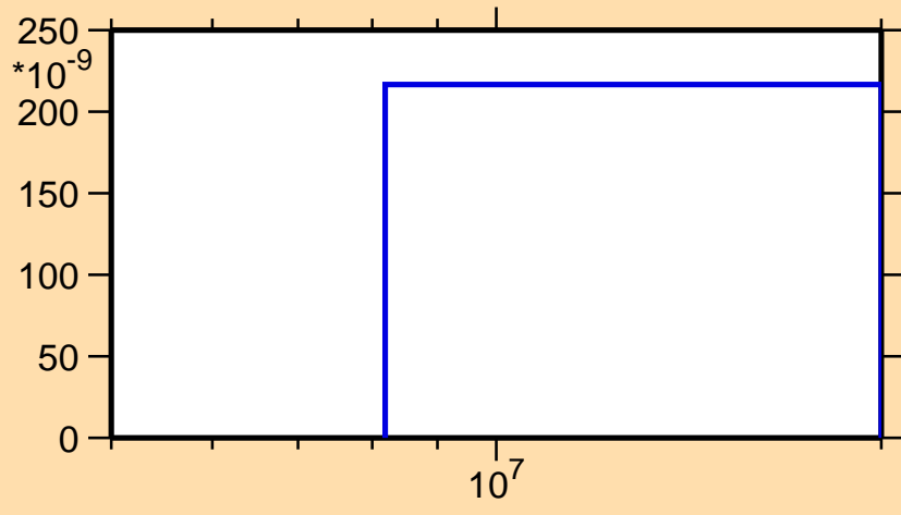
\sigma vs. E for ^{230}\text{Fr}(n,nt)
