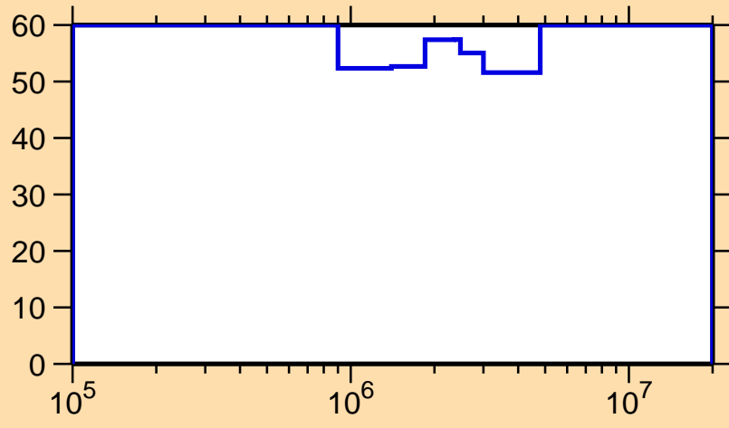
\Delta\sigma/\sigma vs. E for ^{230}\text{Fr}(n,n\text{cont.})
