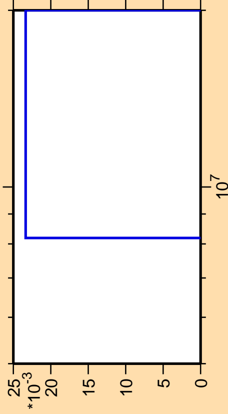
\Delta\sigma/\sigma vs. E for ^{230}\text{Fr}(\text{mt } 11)
