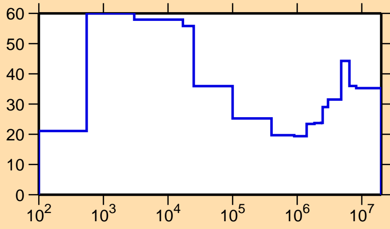
\Delta\sigma/\sigma vs. E for ^{230}\text{Fr}(n,\text{tot.})
