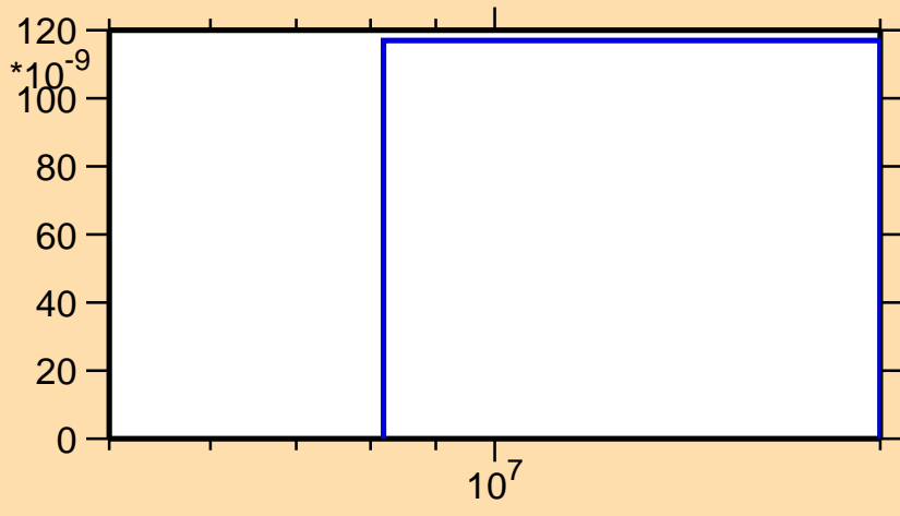
\sigma vs. E for ^{230}\text{Fr}(n,\text{nd})
