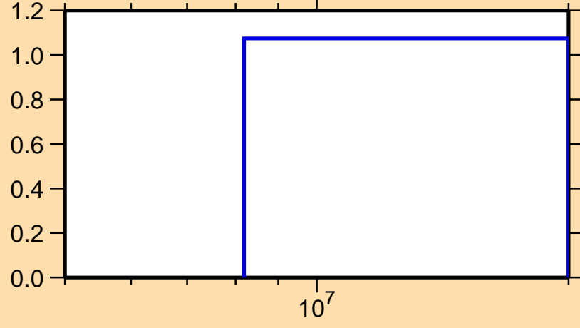
\sigma vs. E for ^{230}\text{Fr}(n,3n)
