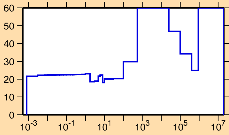
\Delta\sigma/\sigma vs. E for ^{230}\text{Fr}(n,el.)
