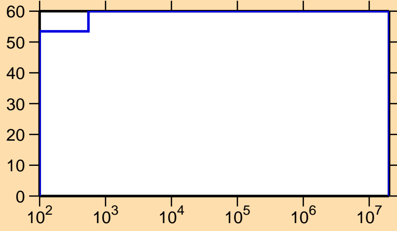
\Delta\sigma/\sigma vs. E for ^{230}\text{Fr}(n,\gamma)
