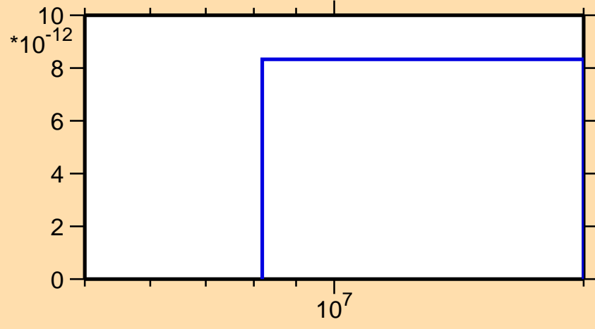
\sigma vs. E for ^{230}\text{Fr}(n,3n\alpha)
