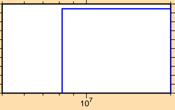
\sigma vs. E for ^{230}\text{Fr}(n,2np)
