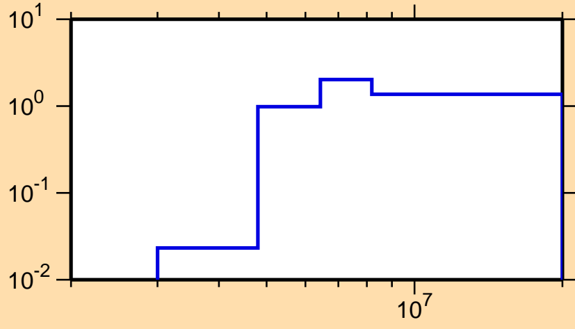
\sigma vs. E for ^{230}\text{Fr}(n,2n)
