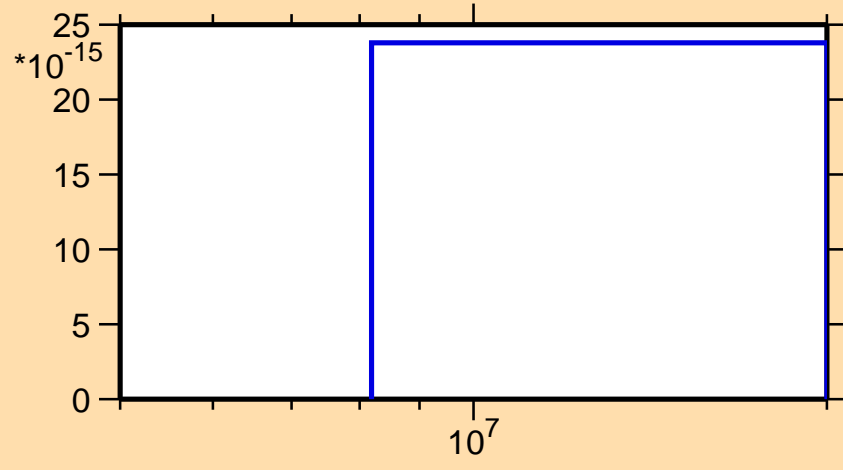
\sigma vs. E for ^{230}\text{Fr}(\text{mt } 11)
