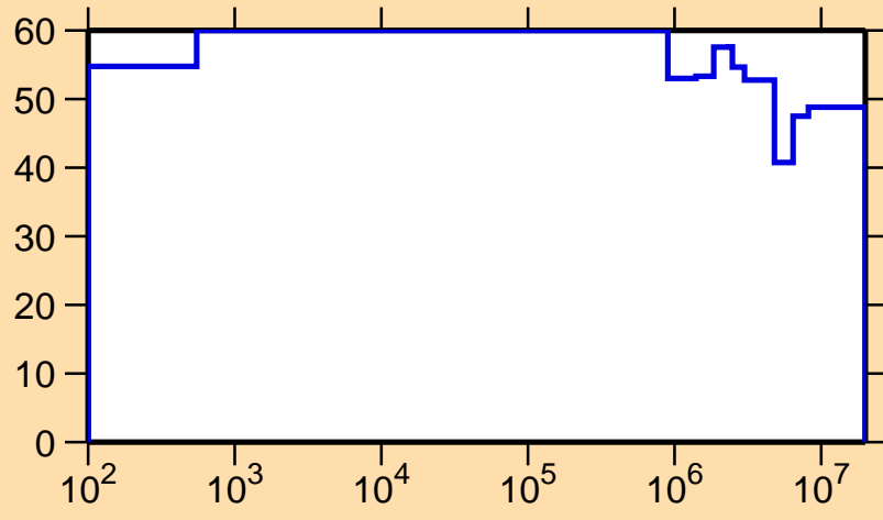
\Delta\sigma/\sigma vs. E for ^{230}\text{Fr}(n,\text{nonel.})
