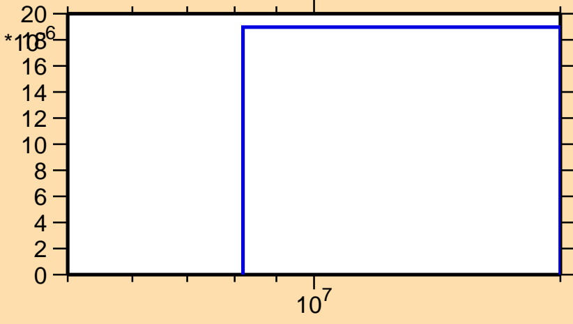
\sigma vs. E for ^{230}\text{Fr}(n,np)
