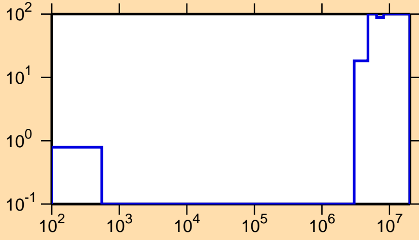
\Delta\sigma/\sigma vs. E for ^{230}\text{Fr}(n,f)
