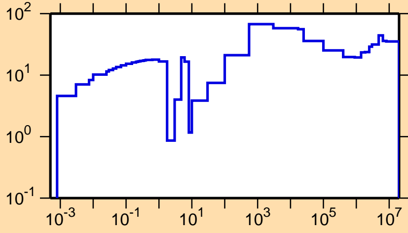
\Delta\sigma/\sigma vs. E for ^{230}\text{Fr}(n,\text{tot.})
