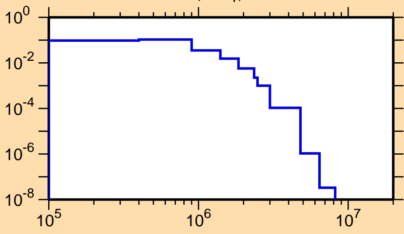
\sigma vs. E for ^{230}\text{Fr}(n,n_1)
