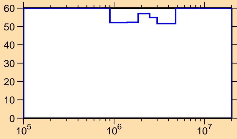
\Delta\sigma/\sigma vs. E for ^{230}\text{Fr}(n,\text{inel.})
