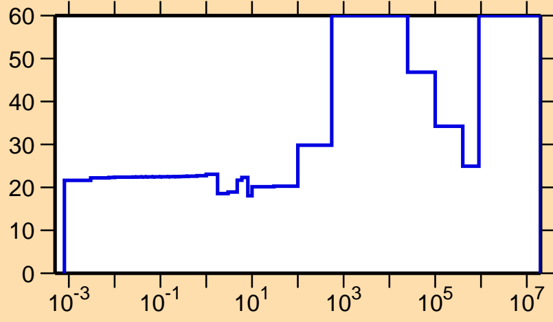
\Delta\sigma/\sigma vs. E for ^{230}\text{Fr}(n,\text{el.})
