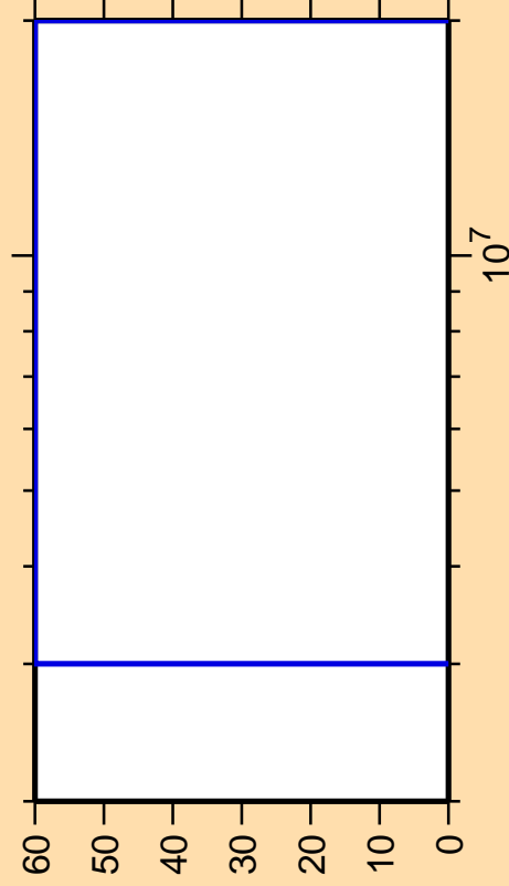
\Delta\sigma/\sigma vs. E for ^{230}\text{Fr}(n,2n)
