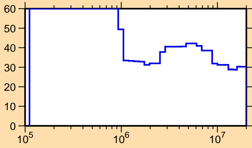
\Delta\sigma/\sigma vs. E for ^{231}\text{Fr}(n,tot.)
