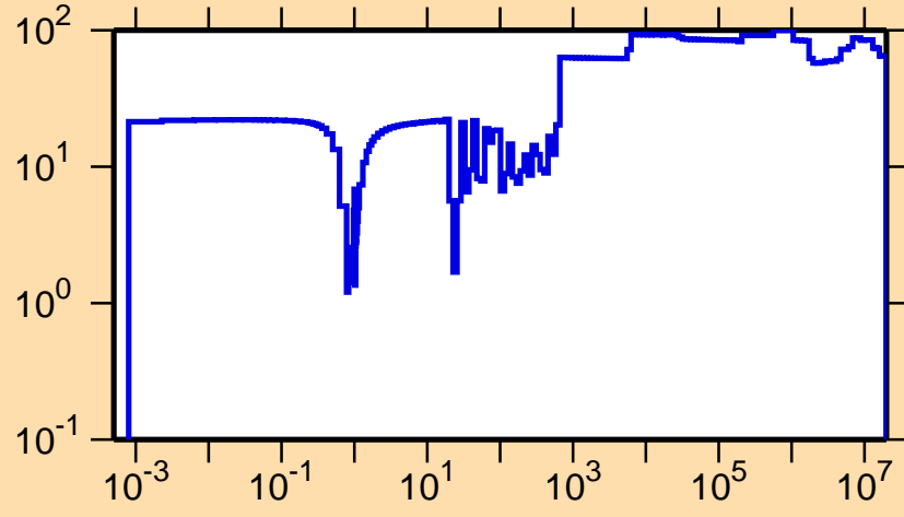
\Delta\sigma/\sigma vs. E for ^{231}\text{Fr}(n,el.)
