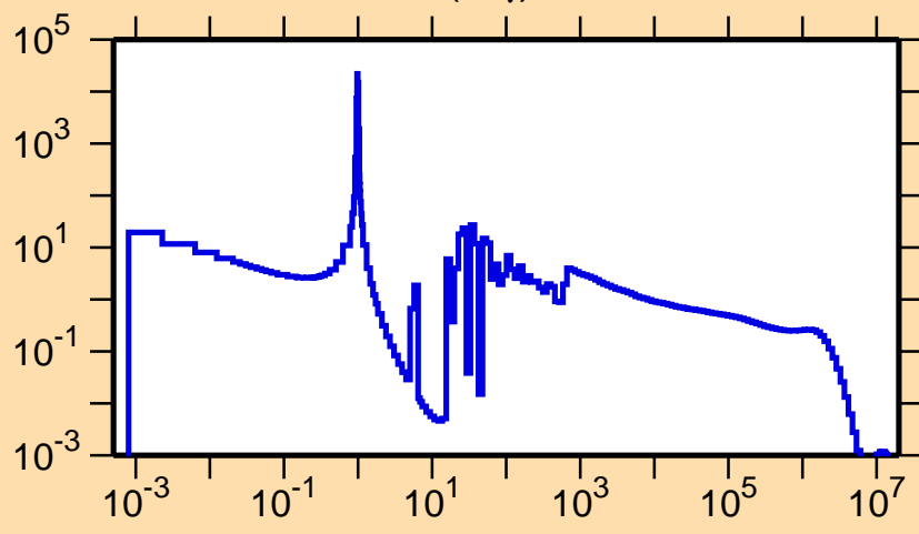
\sigma vs. E for ^{231}\text{Fr}(n,\gamma)
