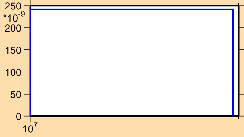
\sigma vs. E for ^{231}\text{Fr}(n,nt)
