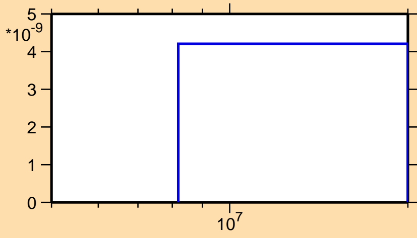
\sigma vs. E for ^{231}\text{Fr}(n,2n\alpha)
