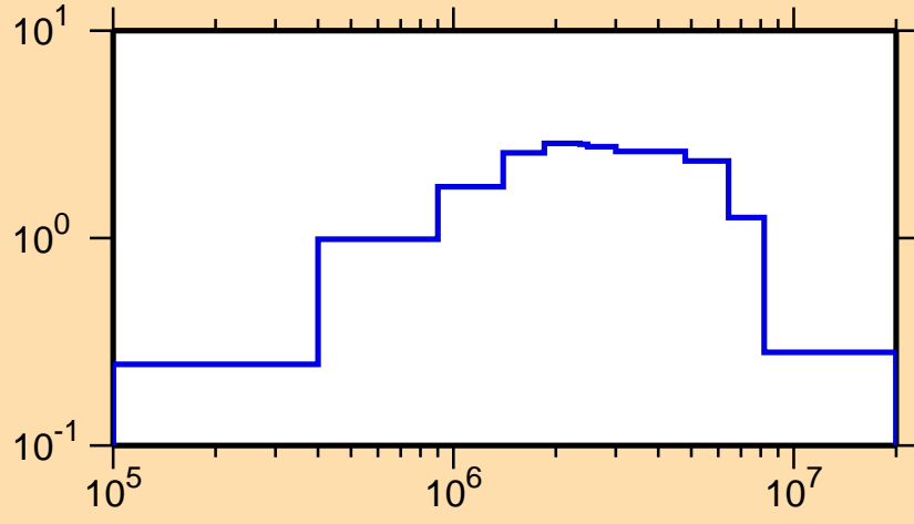
\sigma vs. E for ^{231}\text{Fr}(n,\text{inel.})
