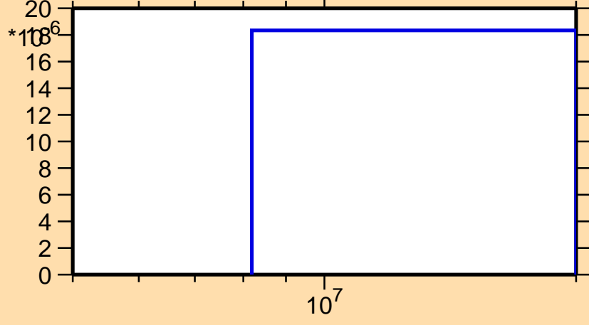
\sigma vs. E for ^{231}\text{Fr}(n,d)
