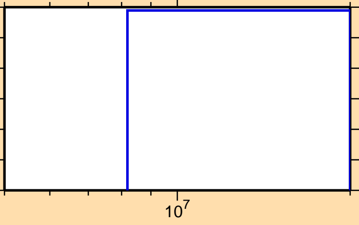
\sigma vs. E for ^{231}\text{Fr}(n,np)
