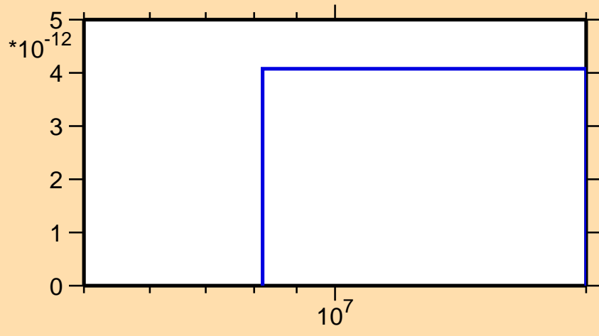
\sigma vs. E for ^{231}\text{Fr}(n,3n\alpha)
