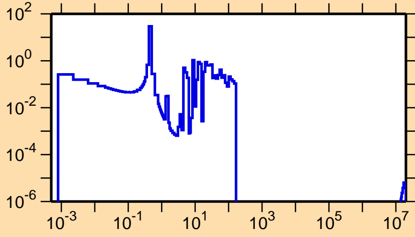
\sigma vs. E for ^{232}\text{Fr}(n,f)
