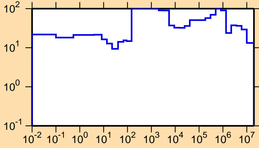
\Delta\sigma/\sigma vs. E for ^{232}\text{Fr}(n,el.)
