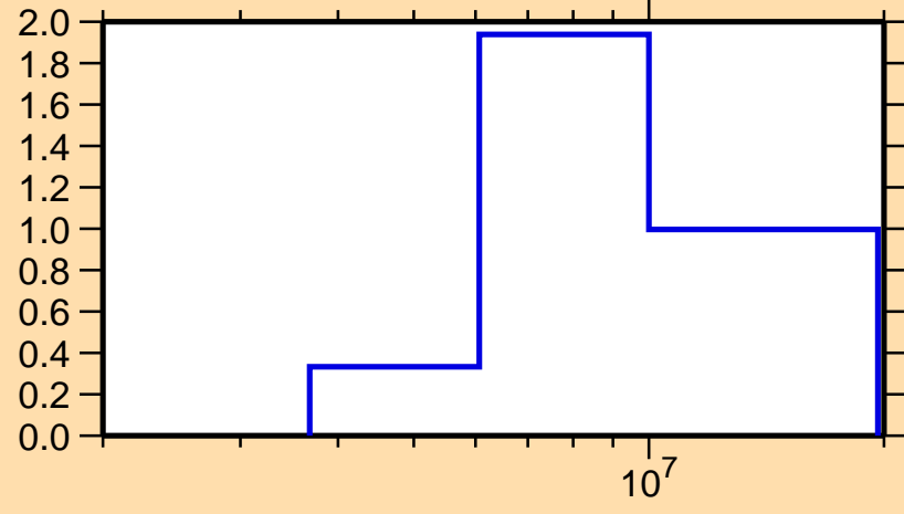
\sigma vs. E for ^{232}\text{Fr}(n,2n)
